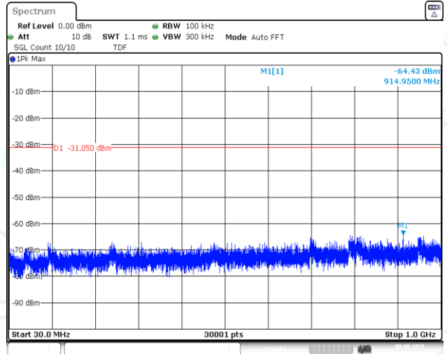
11AX20SISO-Ant1-2462-30~1000-PASS
