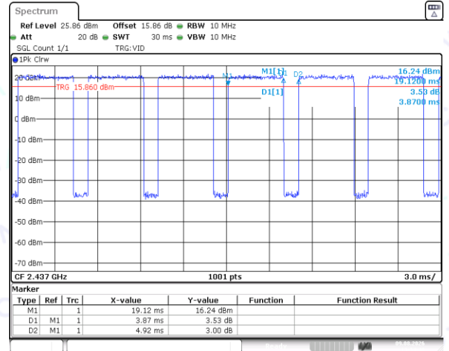
NTNV-11AX20SISO-Ant1-2437
