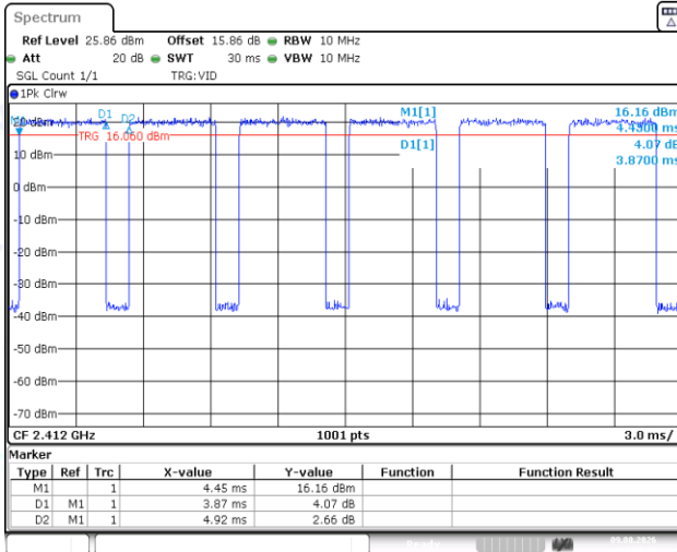
NTNV-11AX20SISO-Ant1-2412
