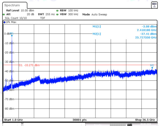
11AX40SISO-Ant1-2422-0~Reference-PASS
