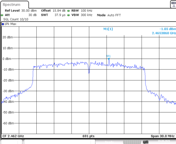
11AX20SISO-Ant1-2462-0~Reference-PASS
