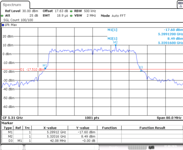
11AX40SISO-Ant1-5310
