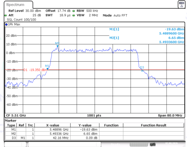
11AX40SISO-Ant1-5510
