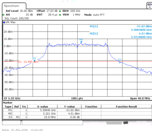
11A-Ant1-5320
