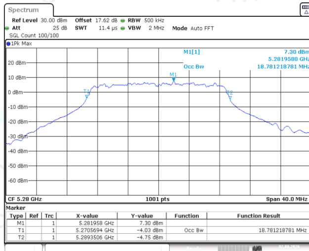
11AC20SISO-Ant1-5280
