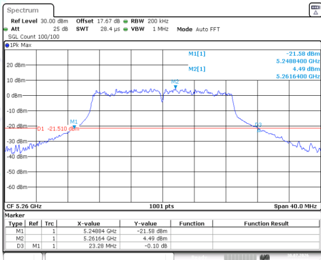
11N20SISO-Ant1-5260
