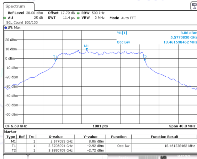
11N20SISO-Ant1-5580
