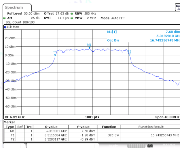
11A-Ant1-5320
