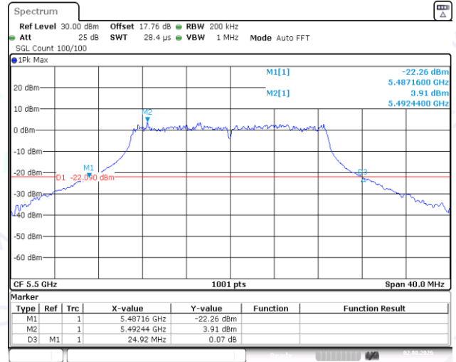
11AC20SISO-Ant1-5500
