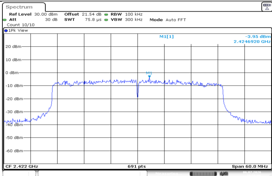
11AX40SISO-Ant1-2422-0~Reference-PASS
