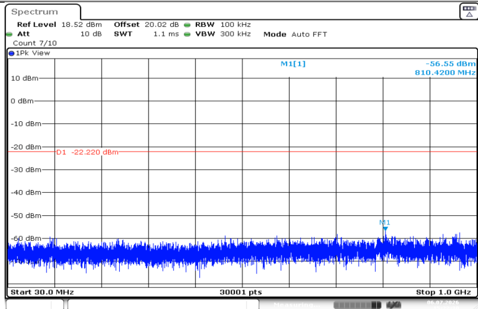
11B-Ant1-2412-0~Reference-PASS
