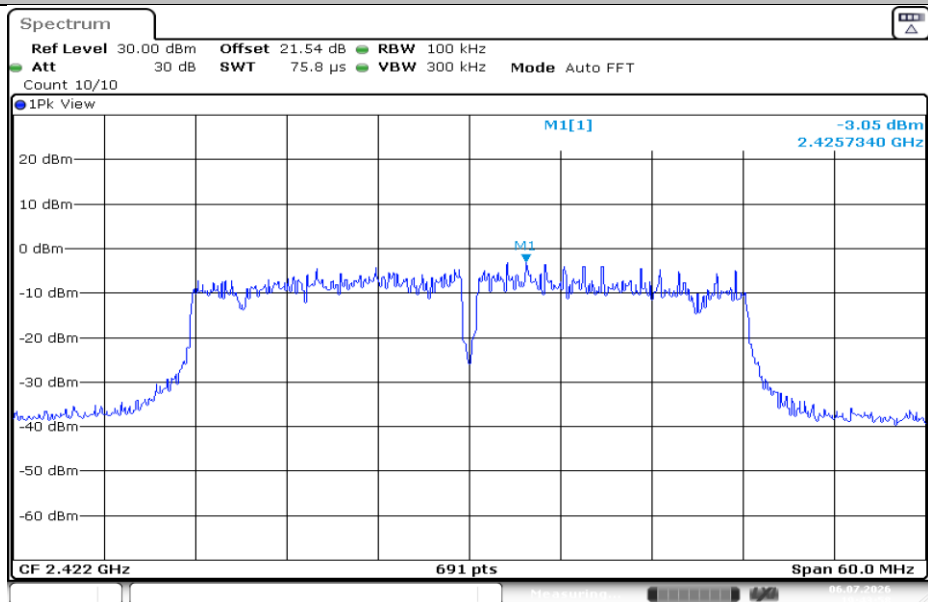
11N40SISO-Ant1-2422-0~Reference-PASS
