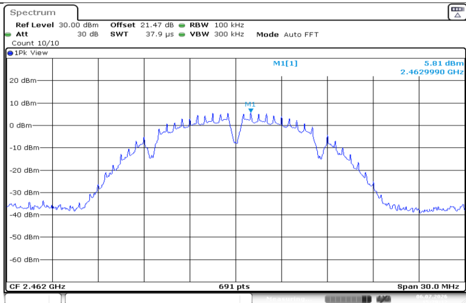
11B-Ant1-2462-0~Reference-PASS
