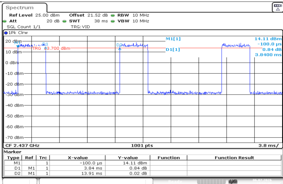
NTNV-11AX40SISO-Ant1-2437
