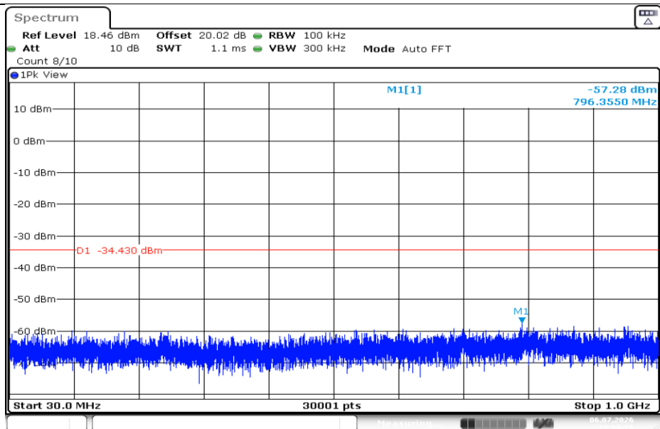
11N40SISO-Ant1-2452-30~1000-PASS
