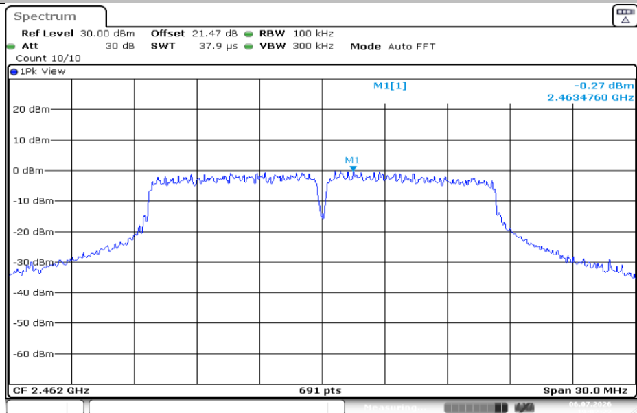
11G-Ant1-2462-0~Reference-PASS
