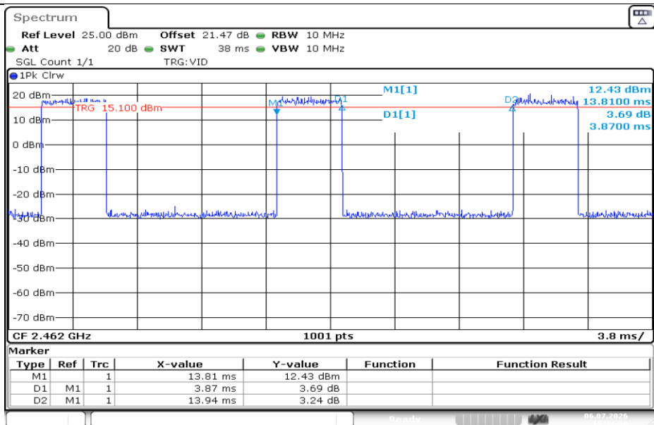
NTNV-11AX20SISO-Ant1-2462
