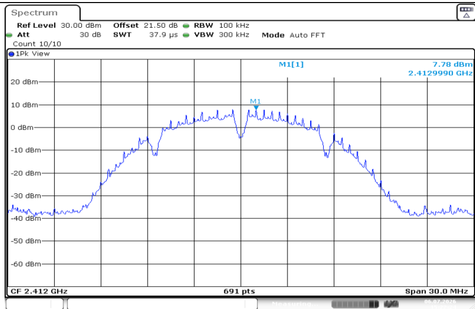
11B-Ant1-2412-0~Reference-PASS
