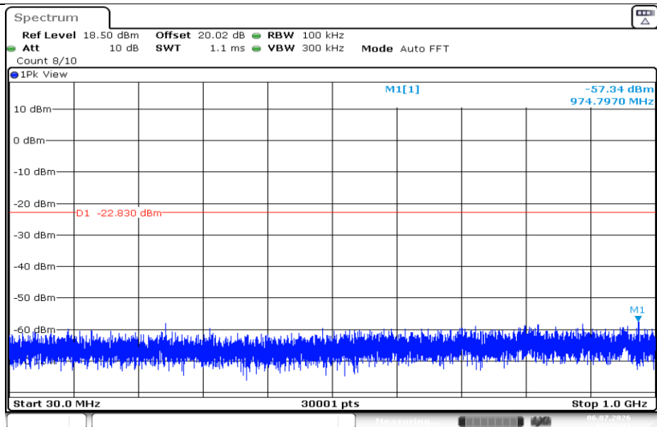
11B-Ant1-2437-30~1000-PASS
