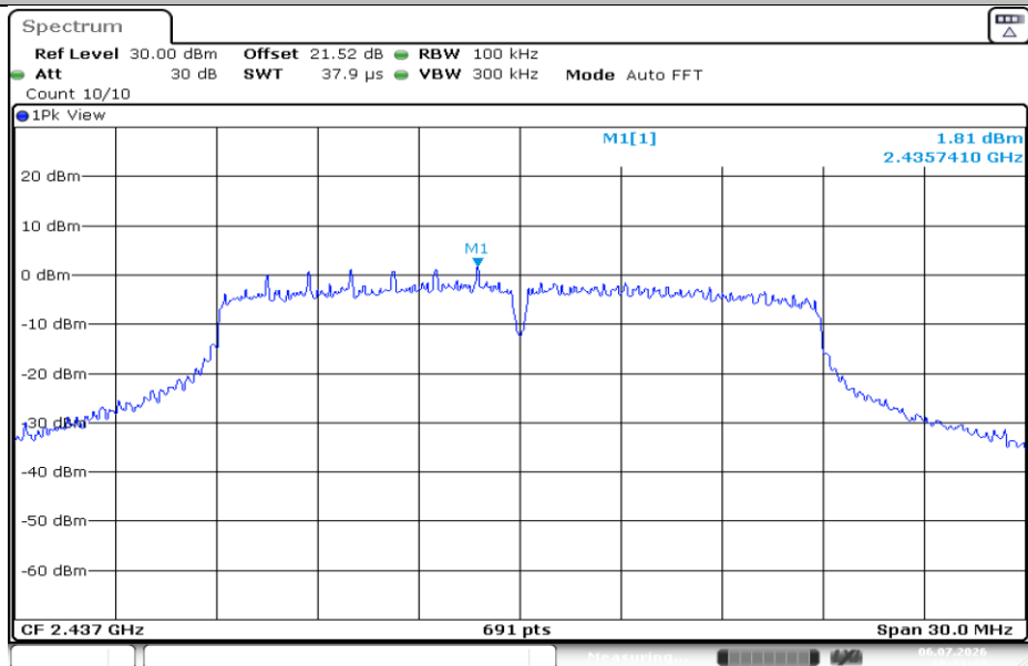
11N20SISO-Ant1-2437-0~Reference-PASS
