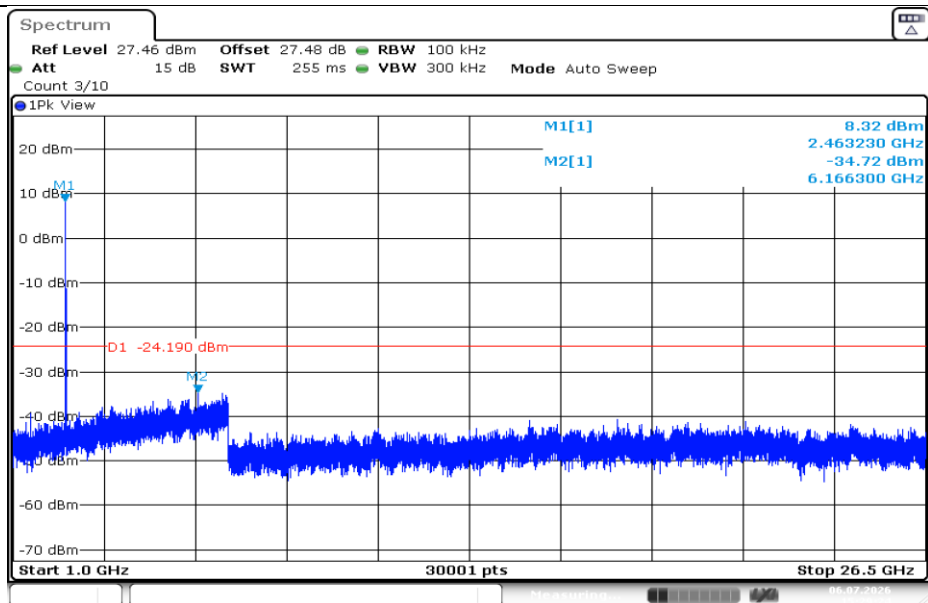
11B-Ant1-2462-1000~26500-PASS
