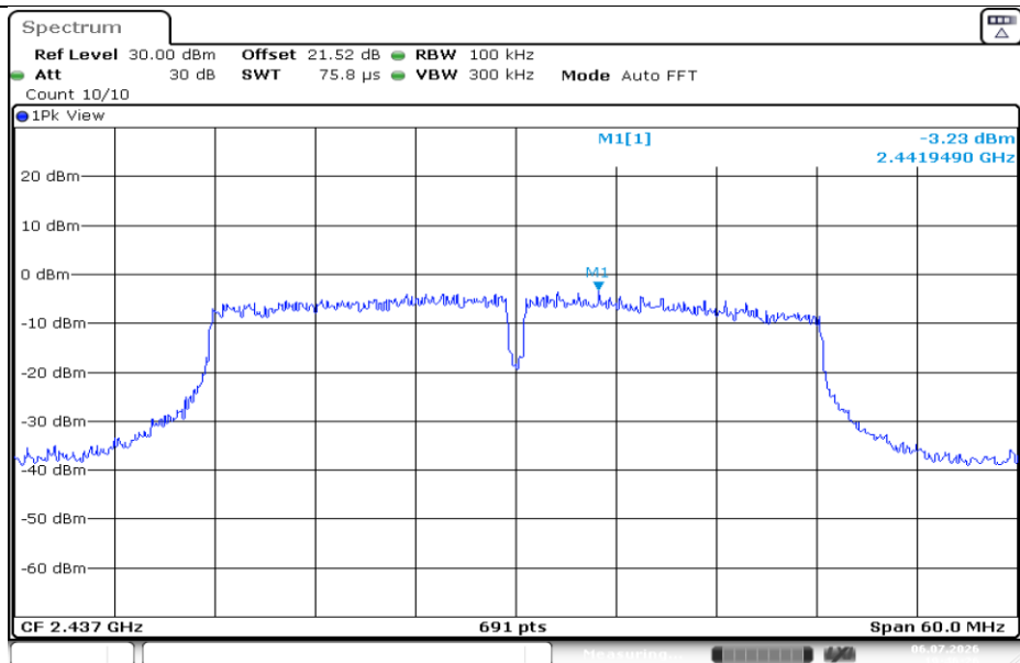
11N40SISO-Ant1-2437-0~Reference-PASS
