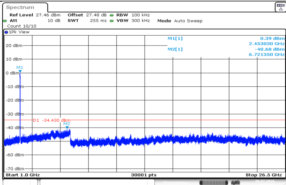
11N40SISO-Ant1-2452-1000~26500-PASS
