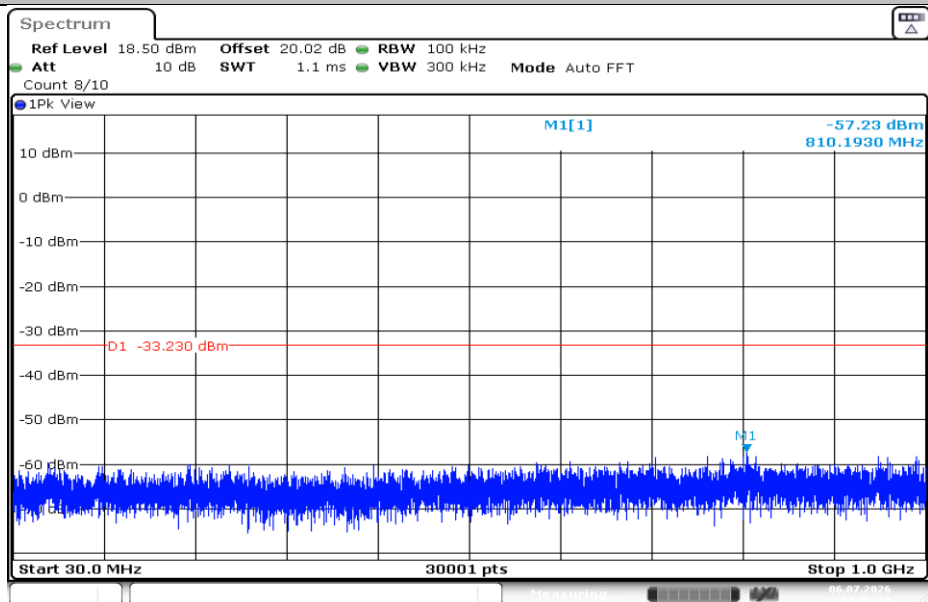
11N40SISO-Ant1-2437-30~1000-PASS
