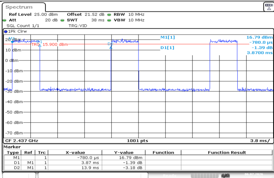
NTNV-11AX20SISO-Ant1-2437
