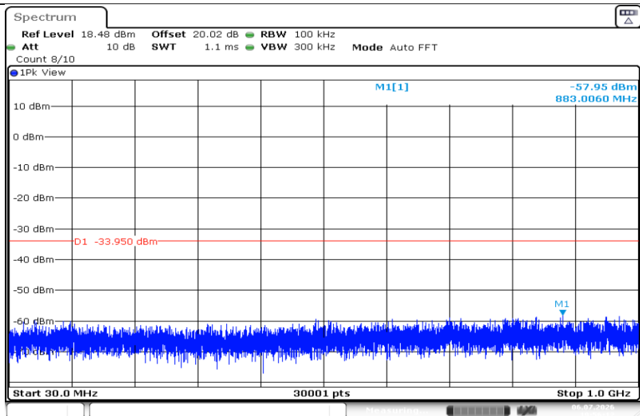
11AX40SISO-Ant1-2422-30~1000-PASS
