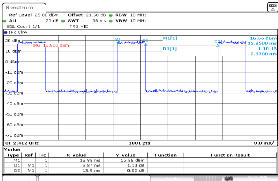
NTNV-11AX20SISO-Ant1-2412
