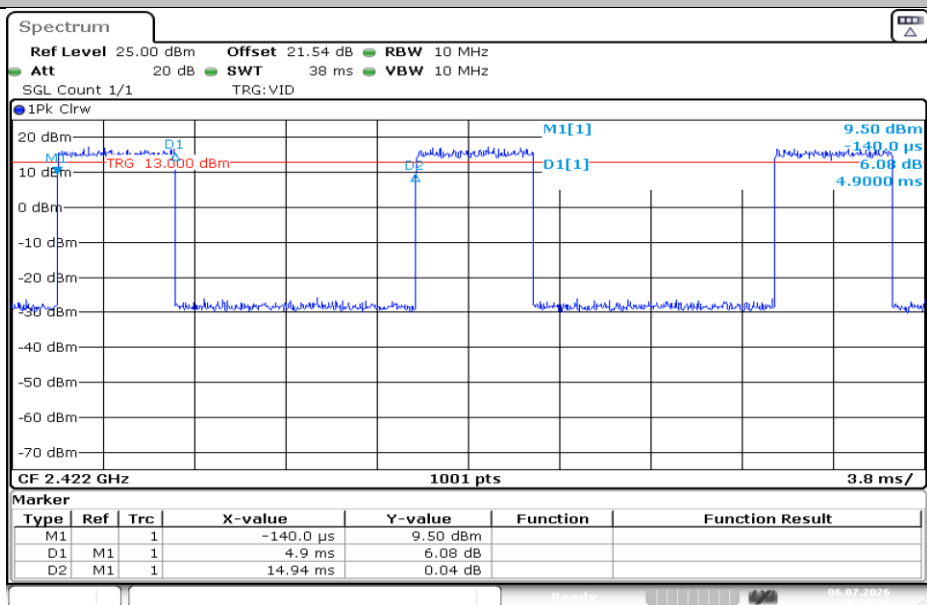
NTNV-11N40SISO-Ant1-2422
