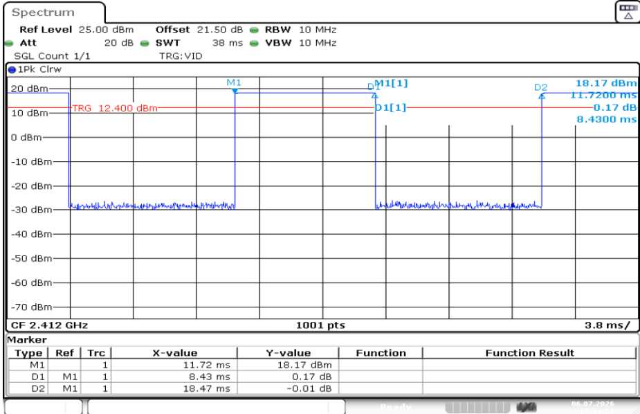
NTNV-11B-Ant1-2412
