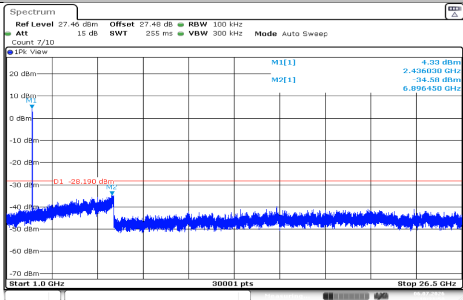
11N20SISO-Ant1-2437-1000~26500-PASS
