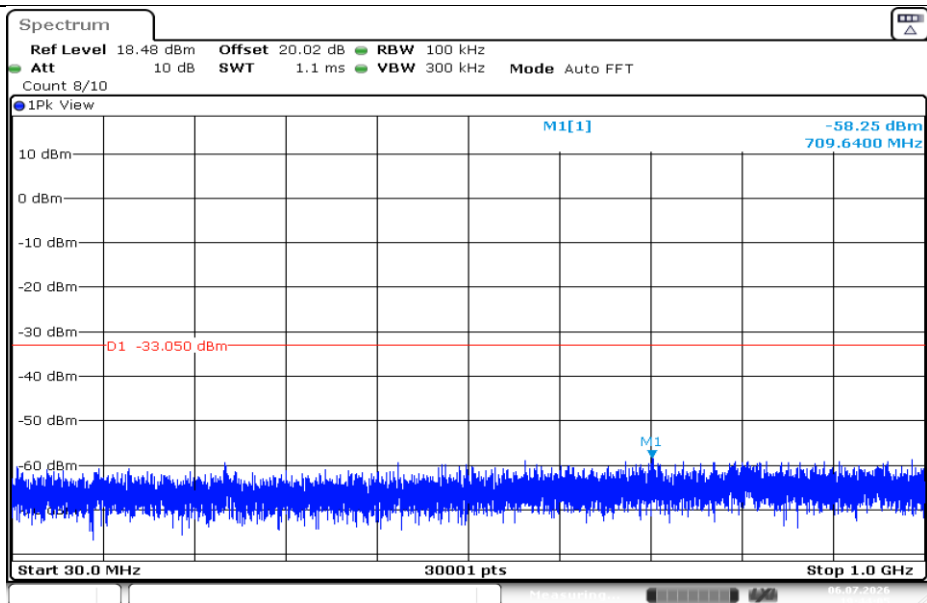
11N40SISO-Ant1-2422-30~1000-PASS
