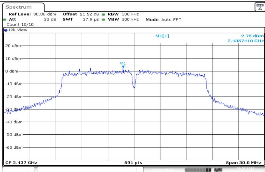
11G-Ant1-2437-0~Reference-PASS
