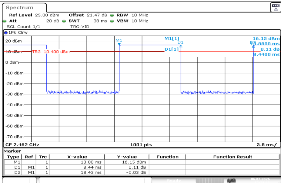
NTNV-11B-Ant1-2462
