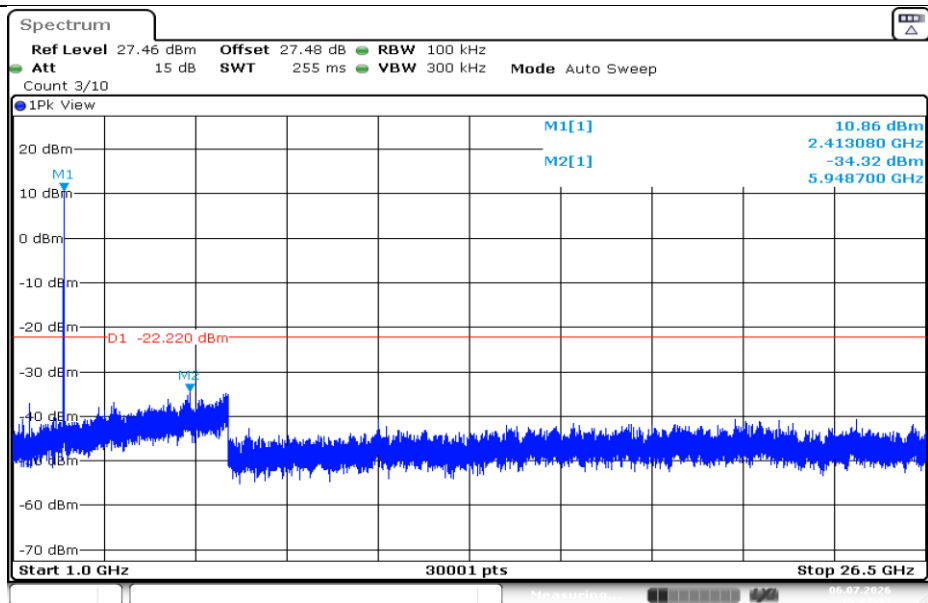
11B-Ant1-2412-1000~26500-PASS
