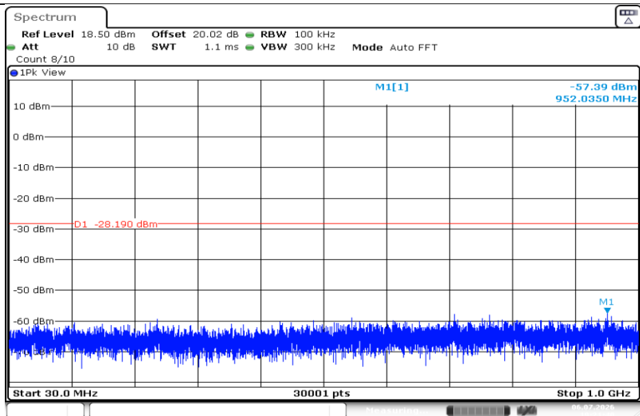
11N20SISO-Ant1-2437-30~1000-PASS
