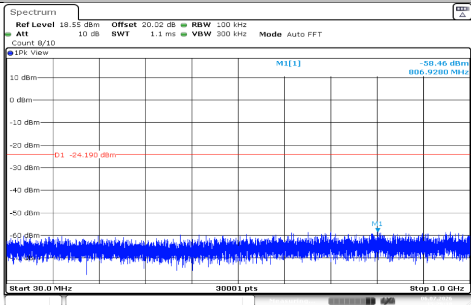
11B-Ant1-2462-30~1000-PASS
