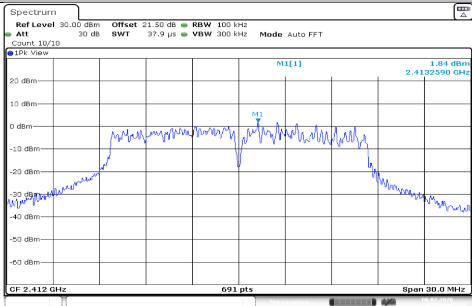
11G-Ant1-2412-0~Reference-PASS
