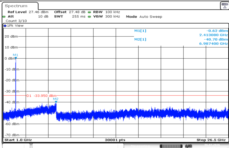
11AX40SISO-Ant1-2422-1000~26500-PASS
