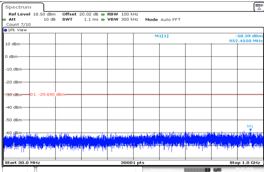
11AX20SISO-Ant1-2437-30~1000-PASS
