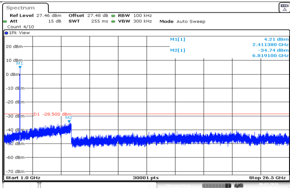
11N20SISO-Ant1-2412-1000~26500-PASS
