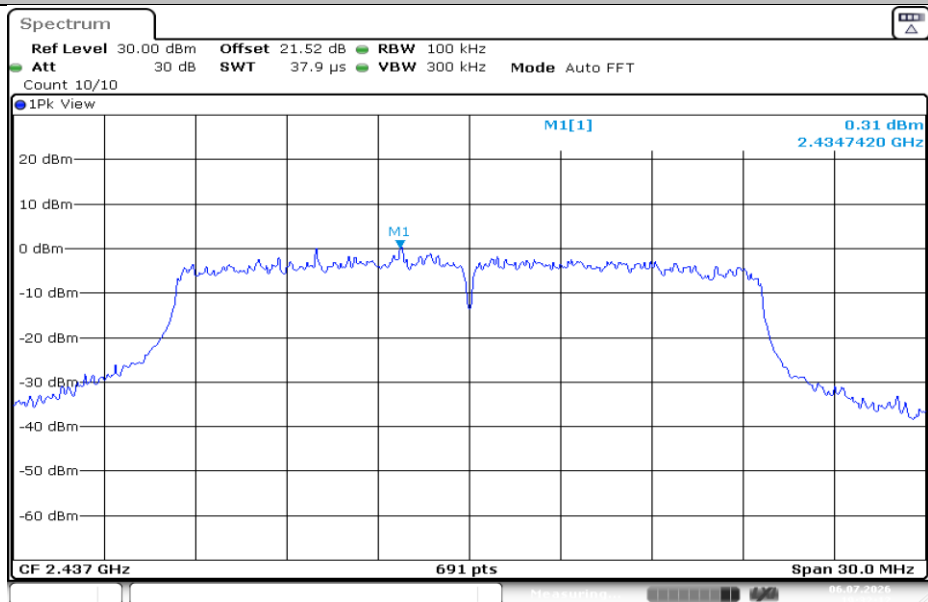
11AX20SISO-Ant1-2437-0~Reference-PASS
