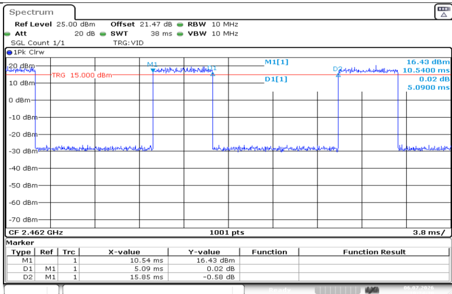
NTNV-11N20SISO-Ant1-2462
