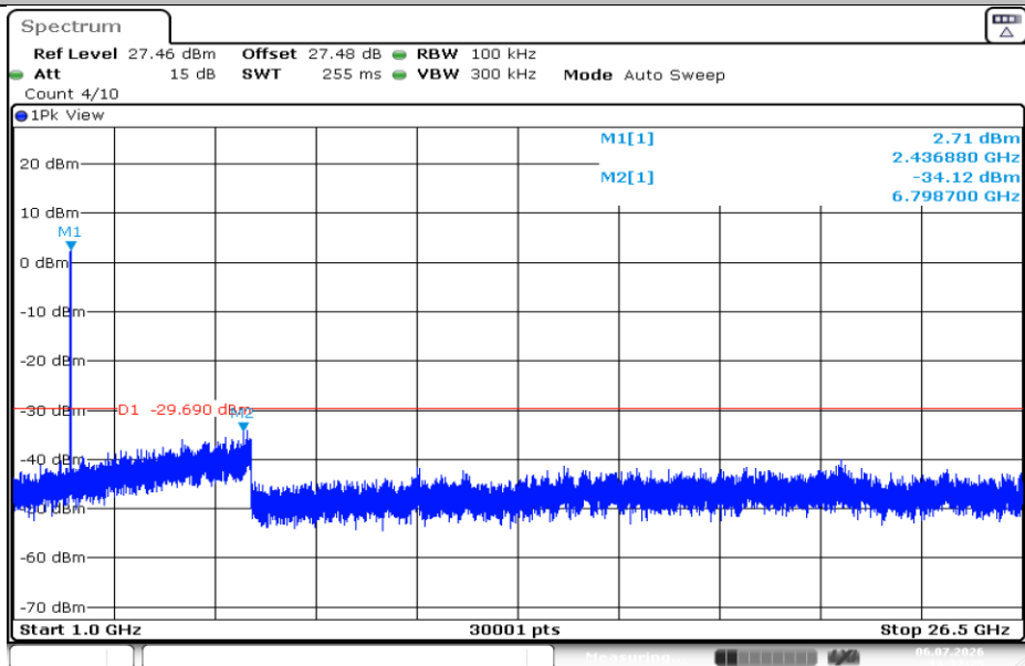
11AX20SISO-Ant1-2437-1000~26500-PASS
