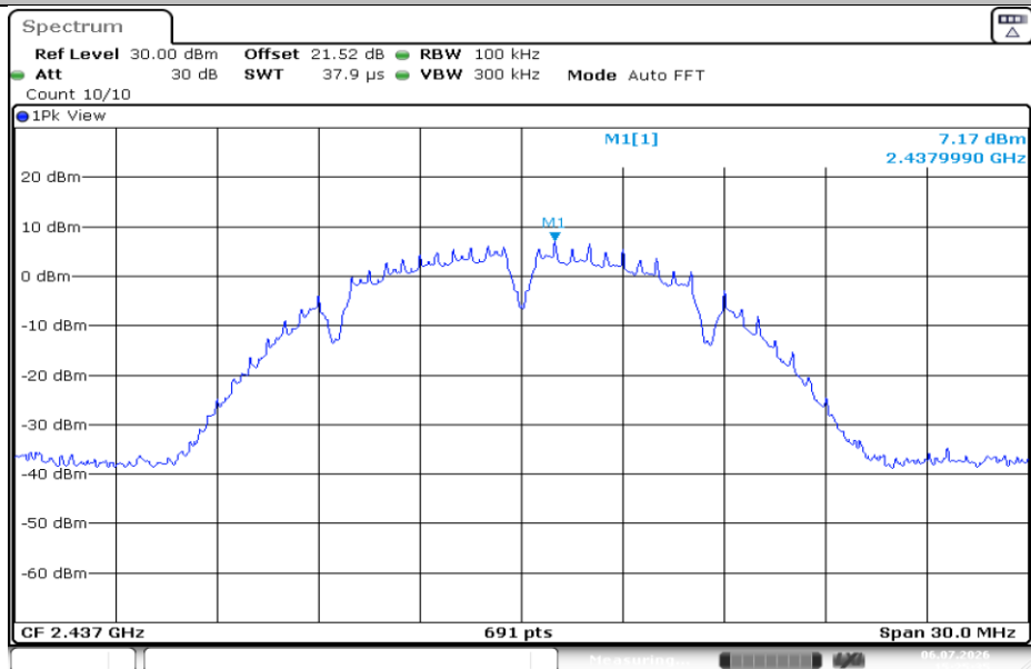
11B-Ant1-2437-0~Reference-PASS
