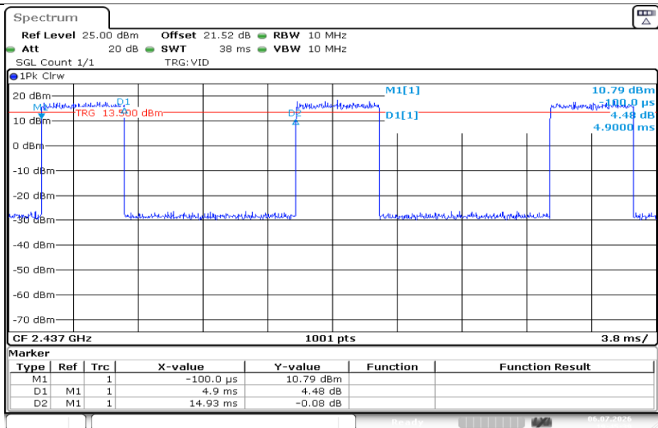
NTNV-11N40SISO-Ant1-2437
