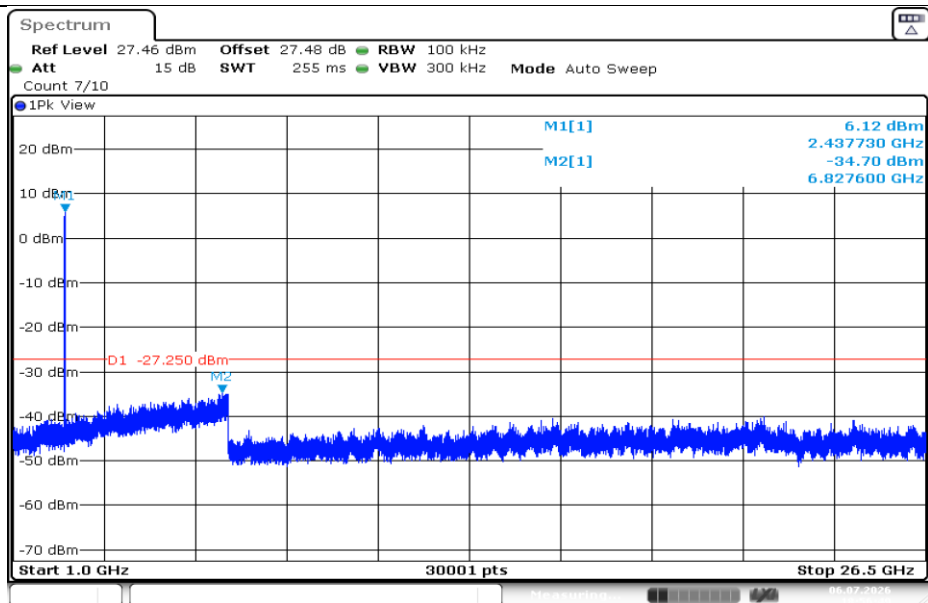
11G-Ant1-2437-1000~26500-PASS
