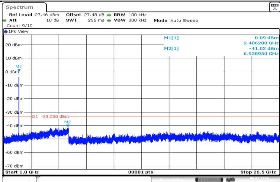
11N40SISO-Ant1-2422-1000~26500-PASS
