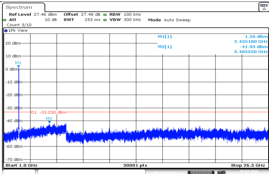
11N40SISO-Ant1-2437-1000~26500-PASS
