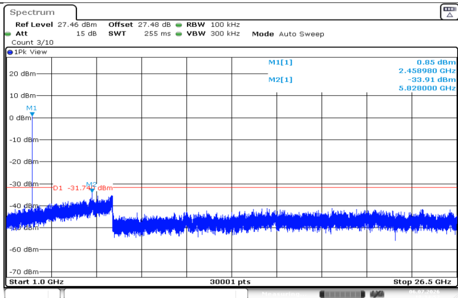
11AX20SISO-Ant1-2462-1000~26500-PASS
