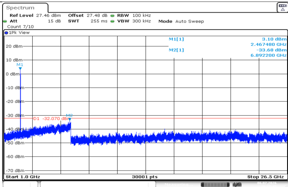
11N20SISO-Ant1-2462-1000~26500-PASS
