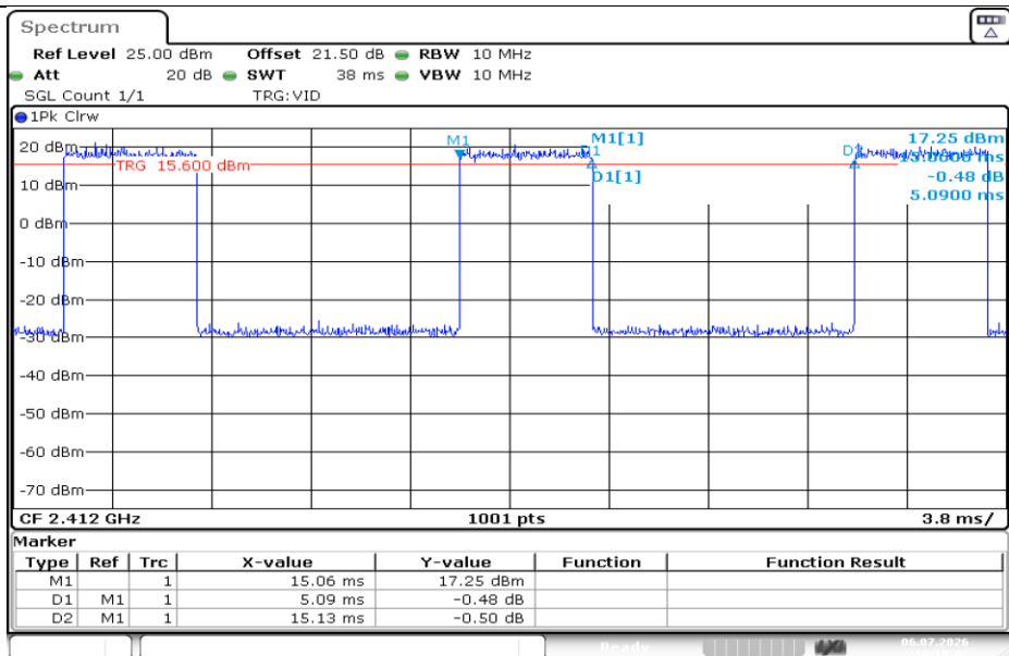
NTVN-11N20SISO-Ant1-2412
