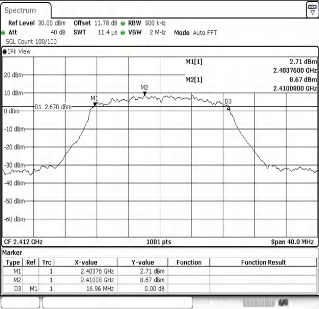
802.11n (HT20)-Ant1-2412-PASS
