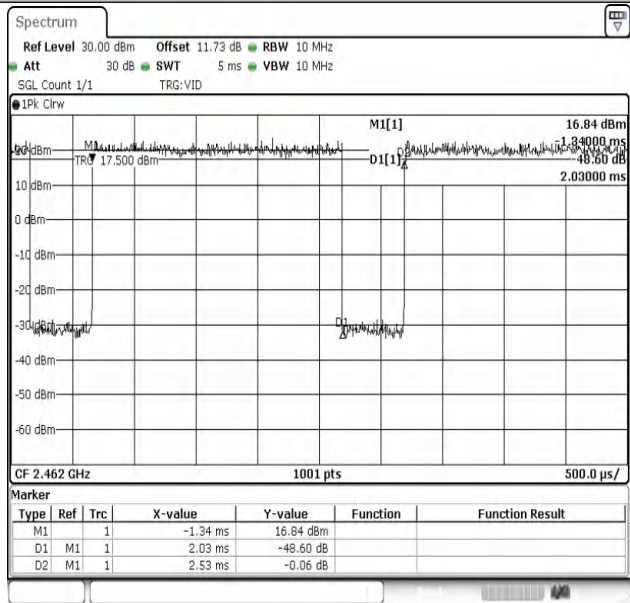
NTNV-802.11g-Ant1-2462
