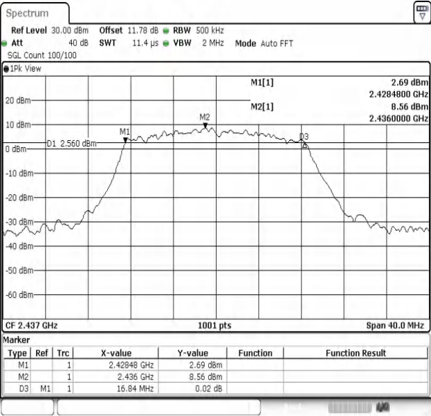
802.11n (HT20)-Ant1-2437-PASS
