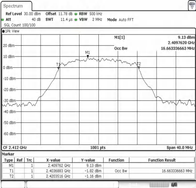
802.11g-Ant1-2412
