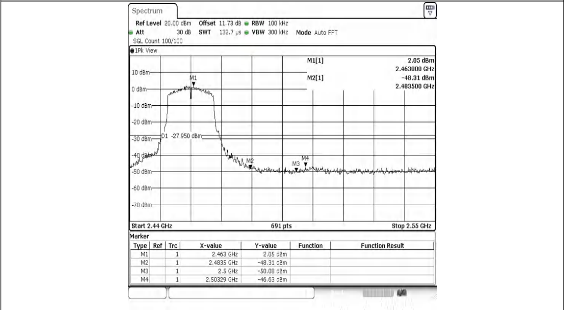
802.11g-Ant1-2462-PASS
