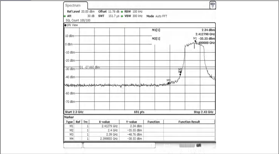
802.11g-Ant1-2412-PASS
