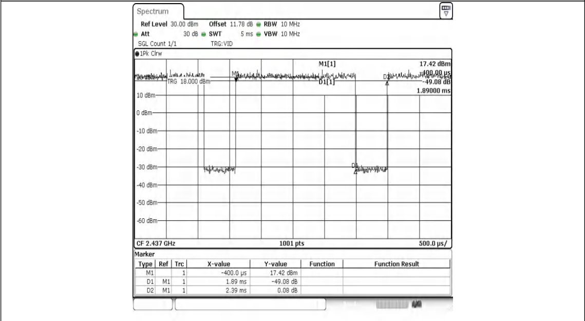
NTNV-802.11n (HT20)-Ant1-2437
