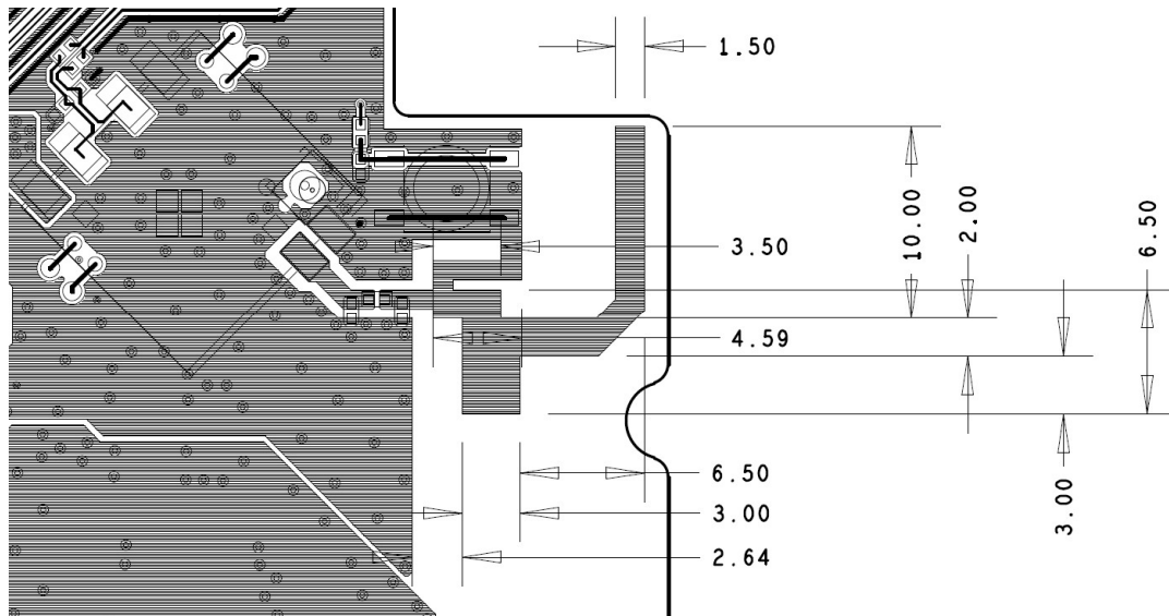
Antenna dimension
