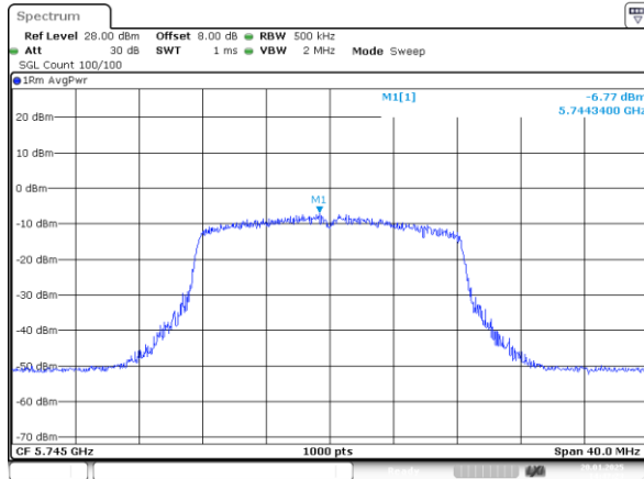
802.11a_5745MHz
