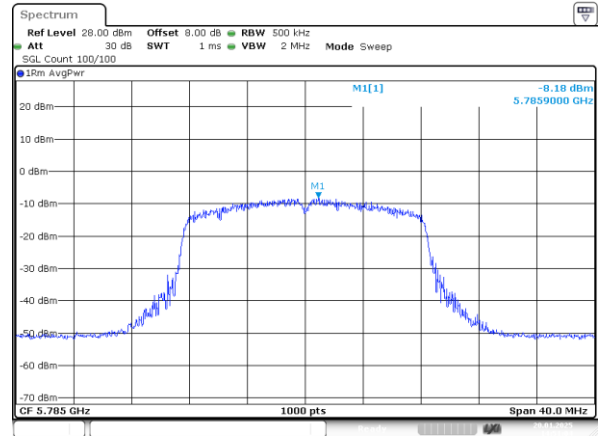
802.11a_5785MHz
