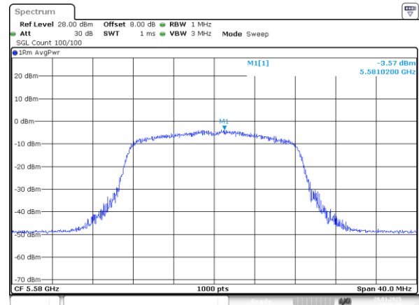
802.11a_5580MHz
