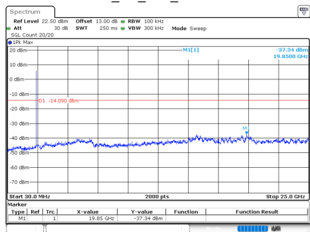
BLE_2M_Low_Channel
