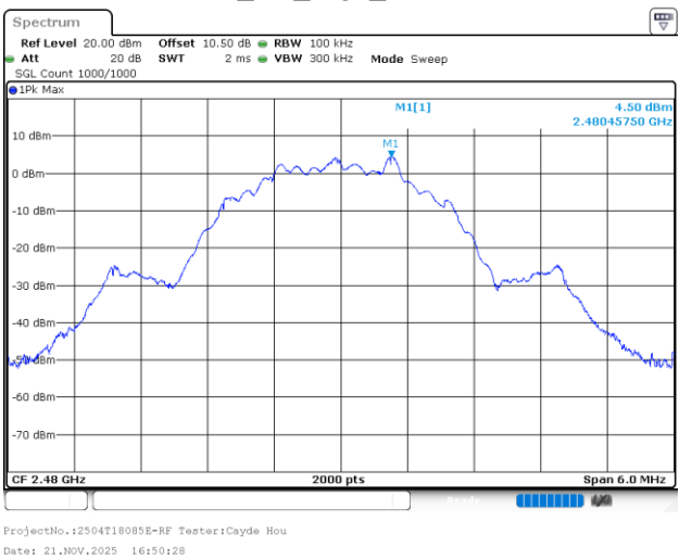
BLE_2M_High_Channel
