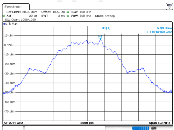
BLE_2M_Middle_Channel
