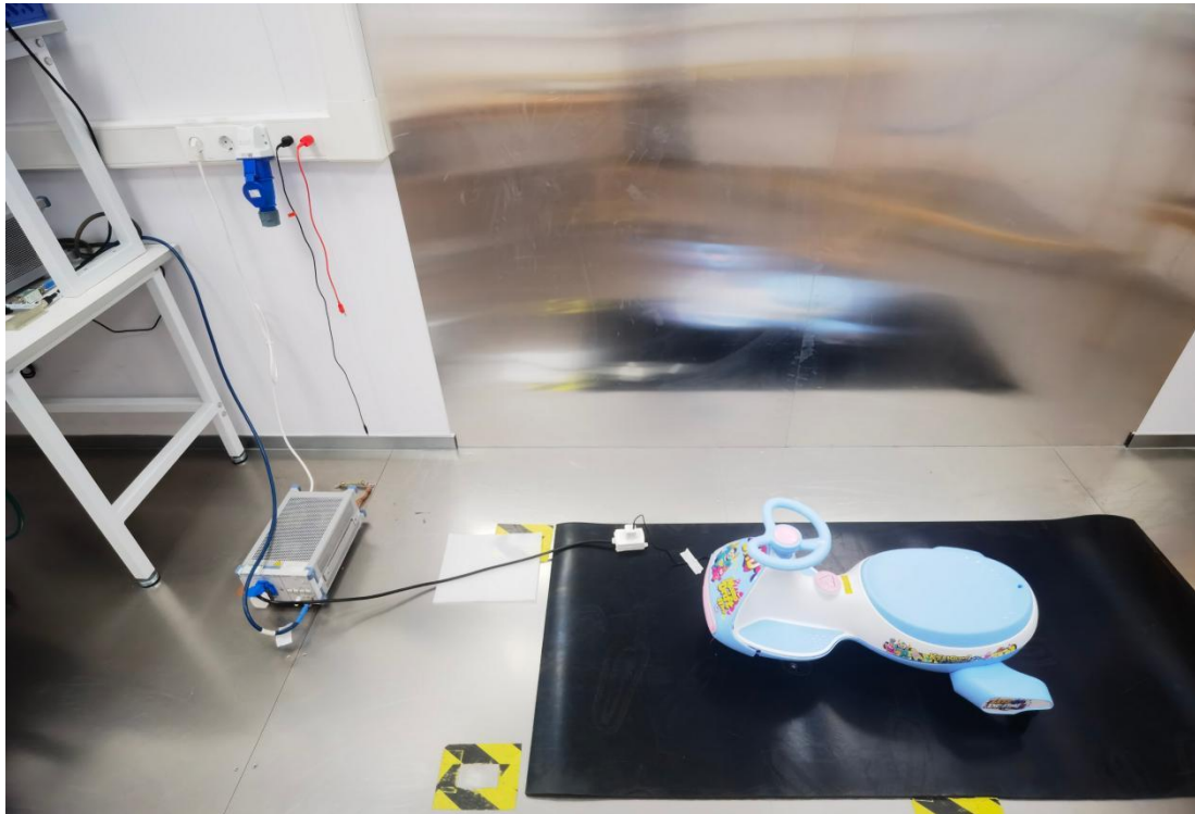
Conducted Emission at AC power line
