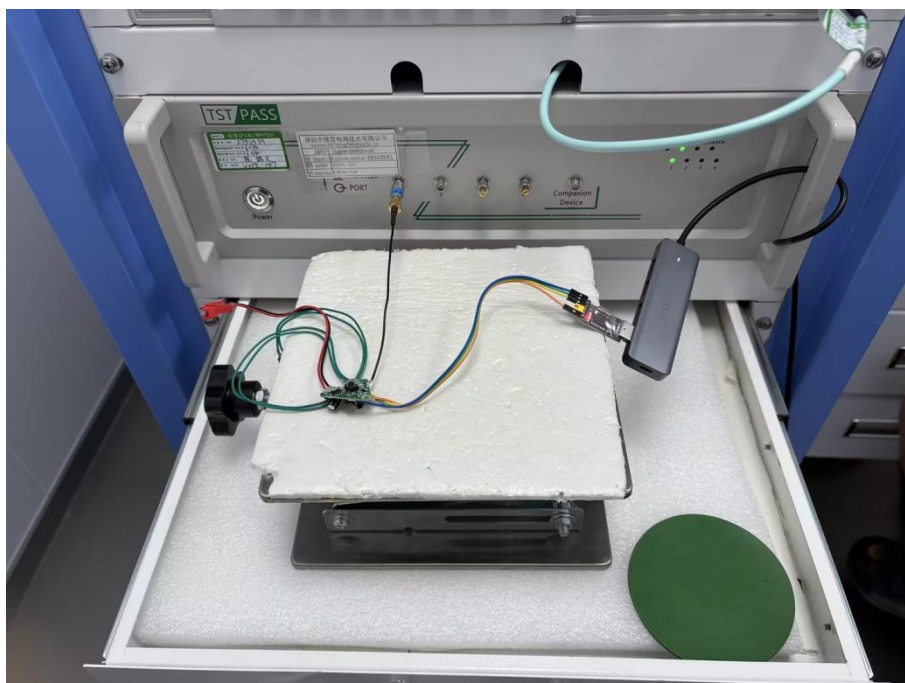
Conducted RF test
