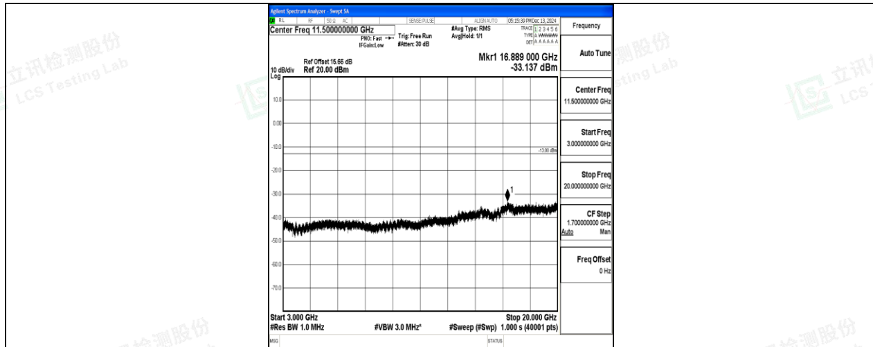
Band2_3MHz_16QAM_18900_1RB#0_3000~20000_3000~20000
