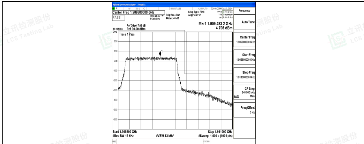
Band2_1.4MHz_16QAM_19193_6RB#0
