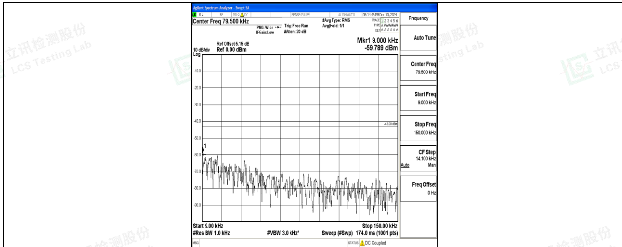
Band2_3MHz_QPSK_18900_1RB#0_0.009~0.15_0.009~0.15
