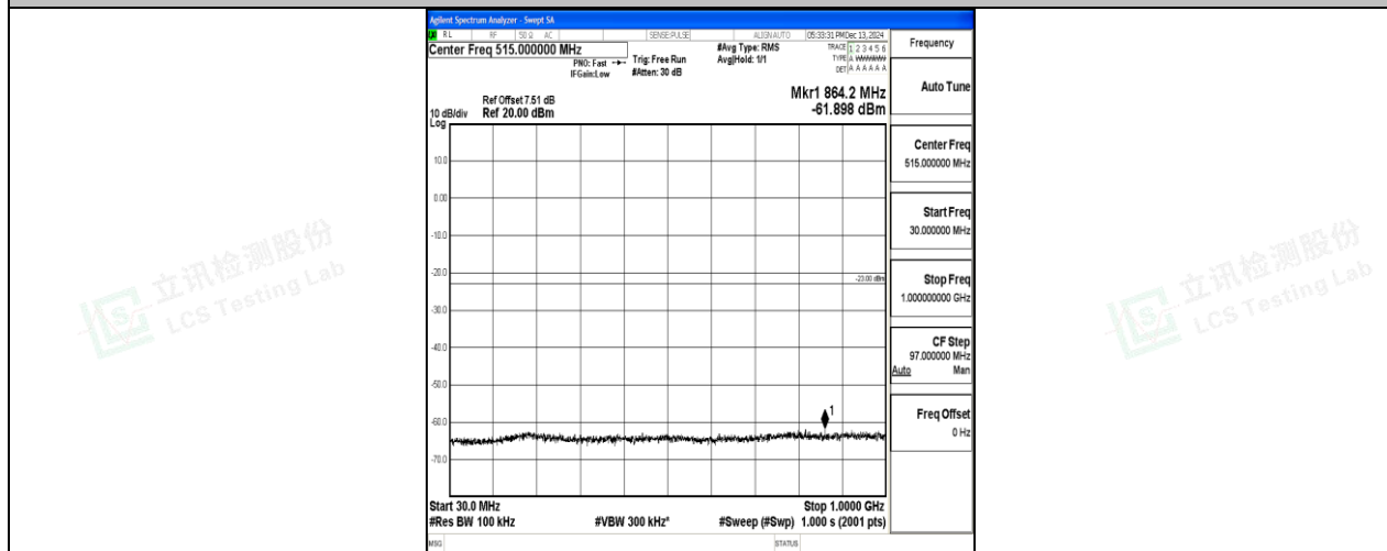
Band2_5MHz_QPSK_18900_1RB#0_30~1000_30~1000
