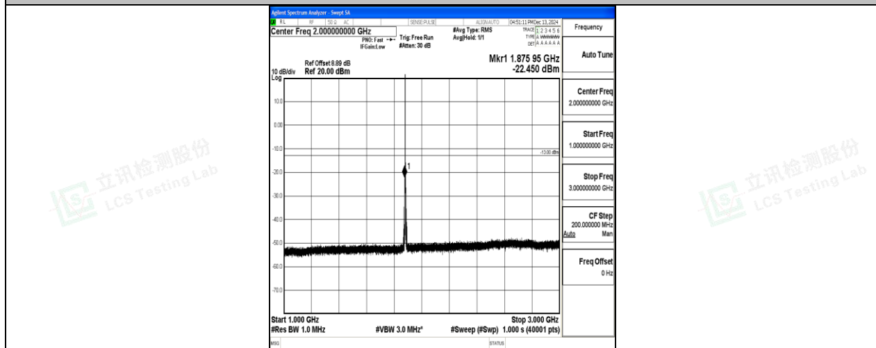
Band2_1.4MHz_16QAM_18900_1RB#0_1000~3000_1000~3000
