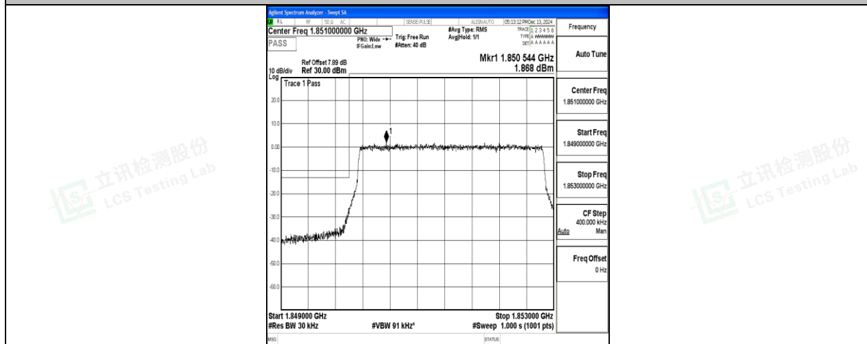
Band2_3MHz_16QAM_18615_15RB#0
