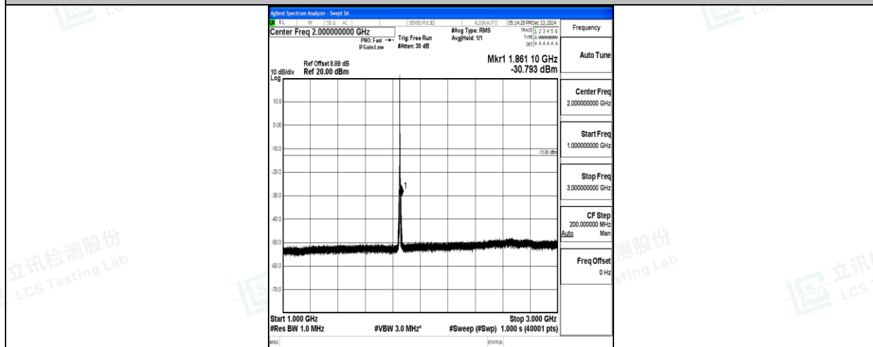
Band2_3MHz_16QAM_18615_1RB#0_1000~3000_1000~3000
