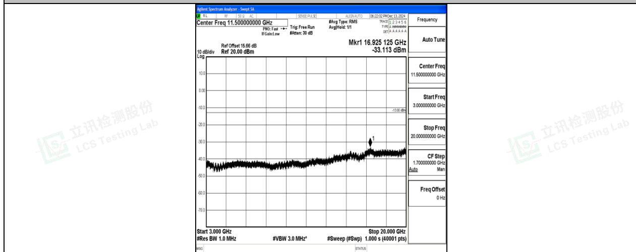
Band2_20MHz_16QAM_18700_1RB#0_3000~20000_3000~20000
