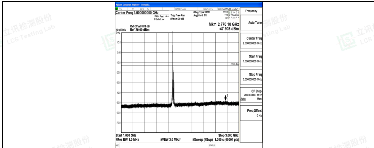
Band2_15MHz_QPSK_18900_1RB#0_1000~3000_1000~3000
