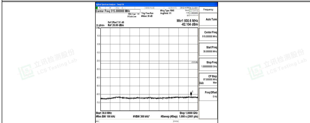
Band2_10MHz_16QAM_19150_1RB#0_30~1000_30~1000
