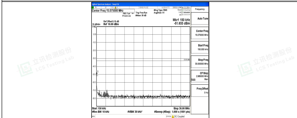
Band2_10MHz_QPSK_19150_1RB#0_0.15~30_0.15~30
