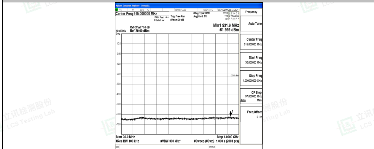
Band2_5MHz_16QAM_18900_1RB#0_30~1000_30~1000
