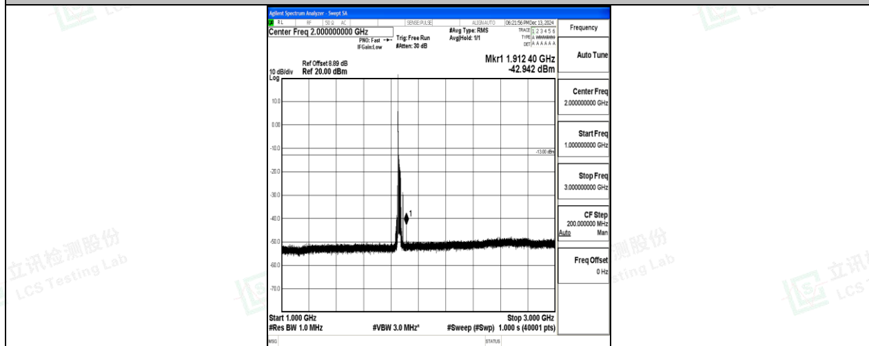
Band2_20MHz_16QAM_18700_1RB#0_1000~3000_1000~3000
