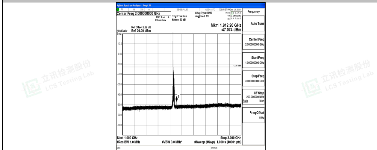
Band2_15MHz_QPSK_18675_1RB#0_1000~3000_1000~3000
