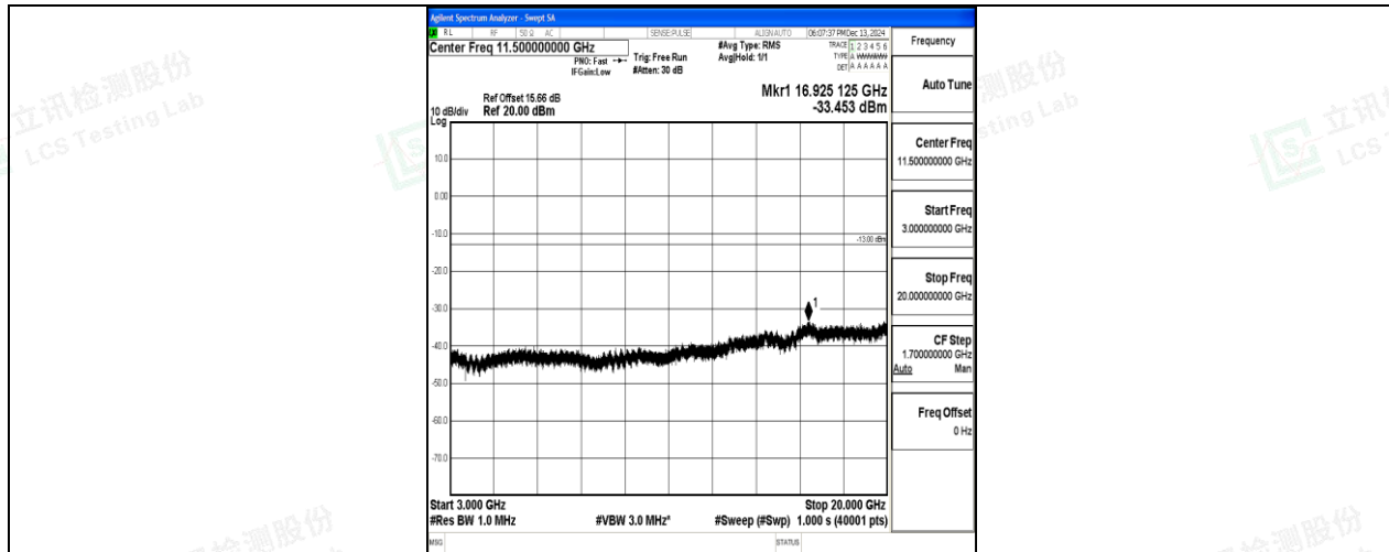
Band2_15MHz_16QAM_18900_1RB#0_3000~20000_3000~20000
