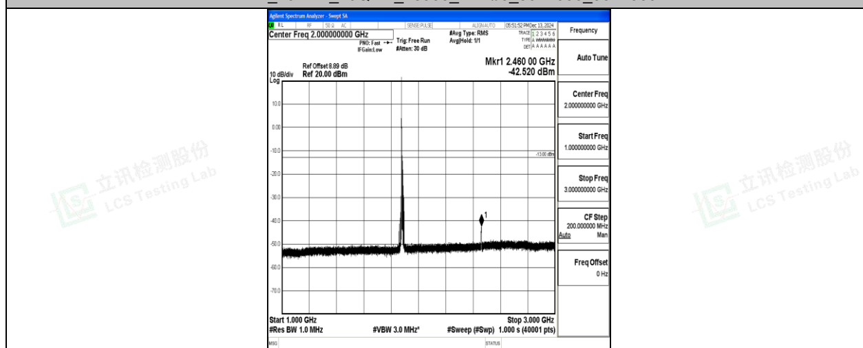
Band2_10MHz_16QAM_18900_1RB#0_1000~3000_1000~3000
