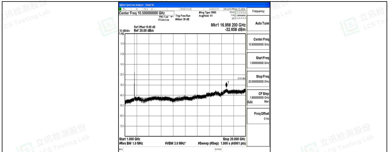
Band7_20MHz_16QAM_20850_1RB#0_1000~20000_1000~20000
