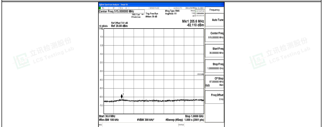
Band7_20MHz_16QAM_20850_1RB#0_30~1000_30~1000
