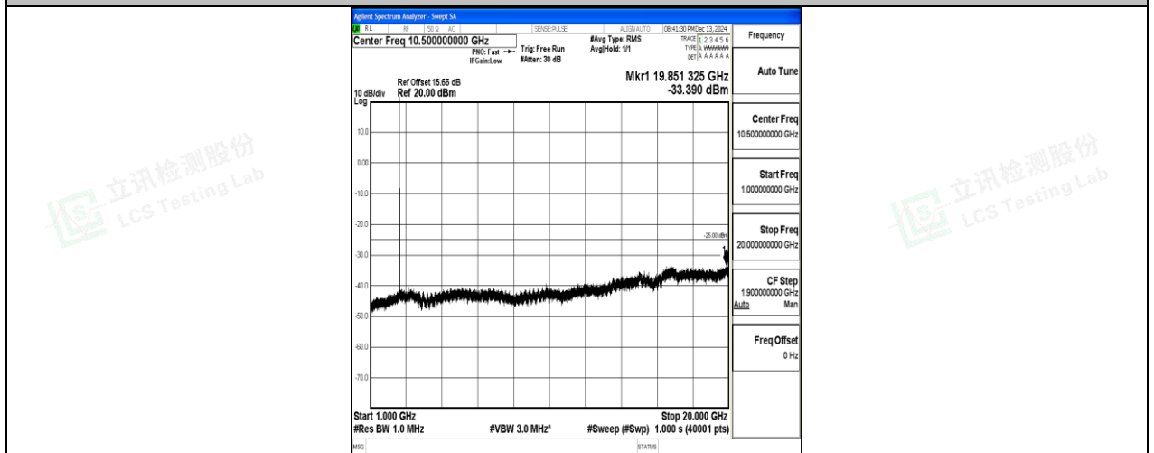
Band7_10MHz_16QAM_21400_1RB#0_1000~20000_1000~20000
