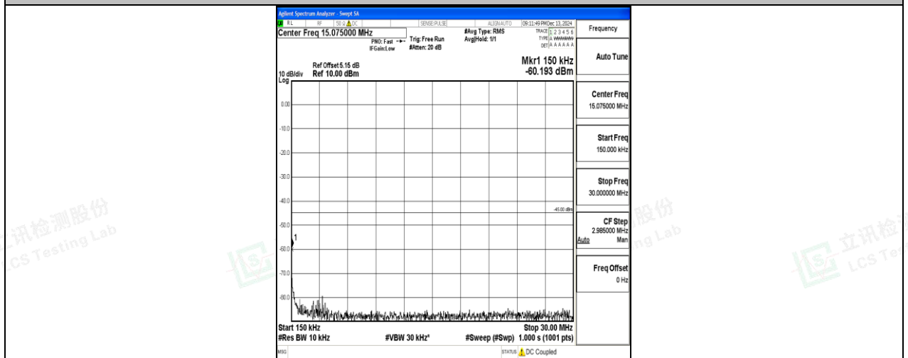
Band7_20MHz_16QAM_20850_1RB#0_0.15~30_0.15~30
