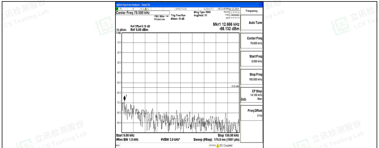
Band7_20MHz_16QAM_20850_1RB#0_0.009~0.15_0.009~0.15
