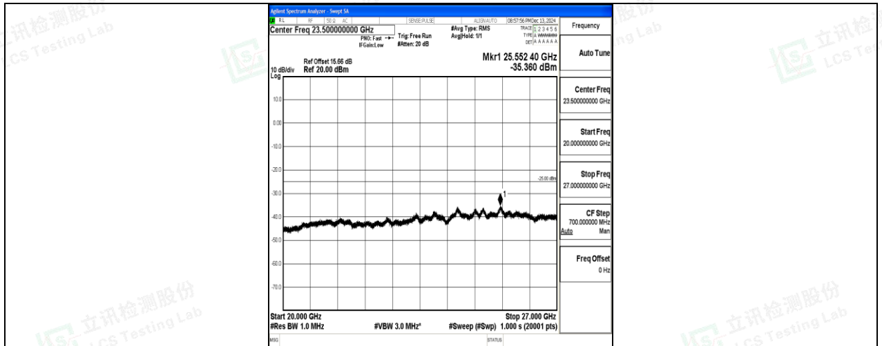
Band7_15MHz_16QAM_21375_1RB#0_20000~27000_20000~27000
