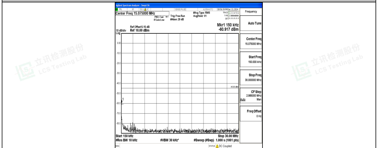
Band7_15MHz_16QAM_21100_1RB#0_0.15~30_0.15~30
