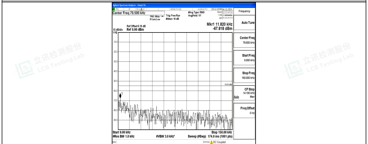
Band7_20MHz_QPSK_21100_1RB#0_0.009~0.15_0.009~0.15
