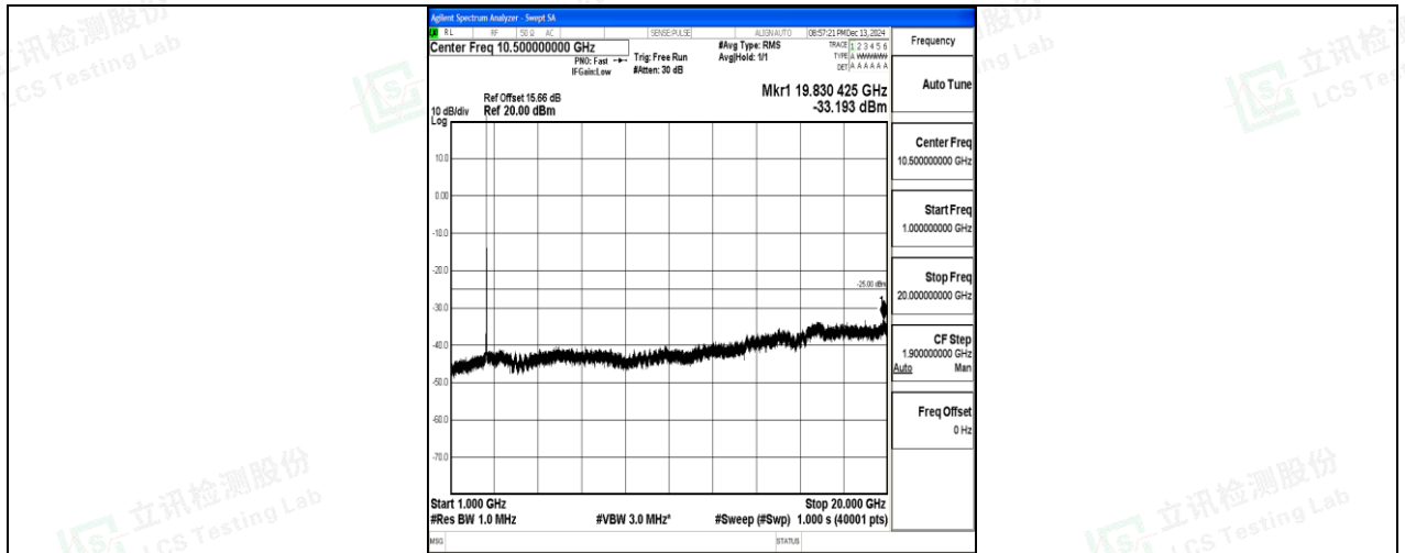
Band7_15MHz_QPSK_21375_1RB#0_1000~20000_1000~20000
