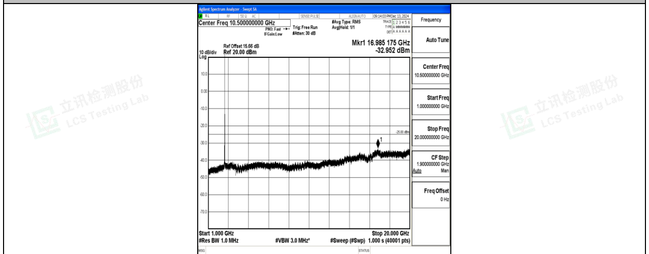
Band7_20MHz_16QAM_21350_1RB#0_1000~20000_1000~20000
