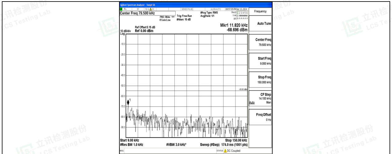
Band7_15MHz_QPSK_21375_1RB#0_0.009~0.15_0.009~0.15
