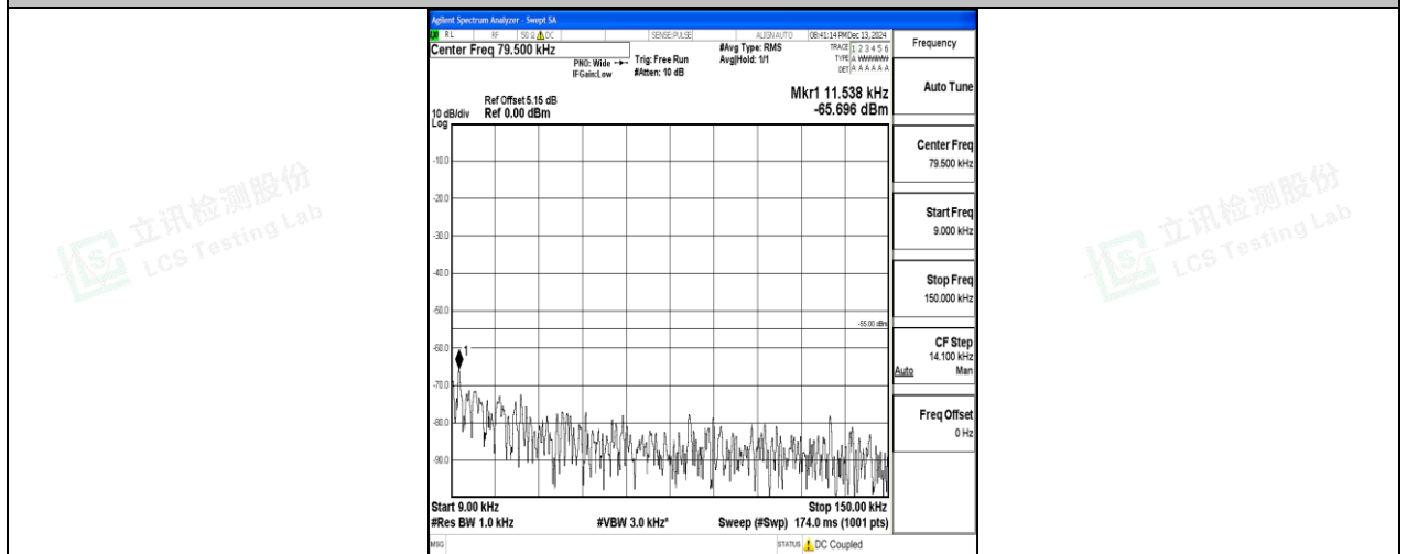
Band7_10MHz_16QAM_21400_1RB#0_0.009~0.15_0.009~0.15
