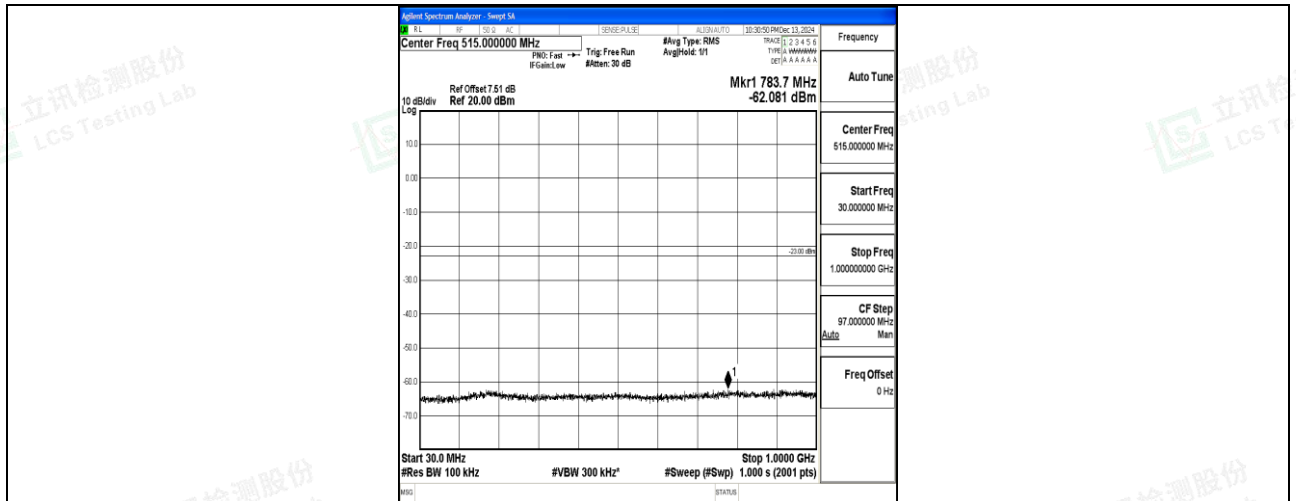
Band66_10MHz_QPSK_132622_1RB#0_30~1000_30~1000
