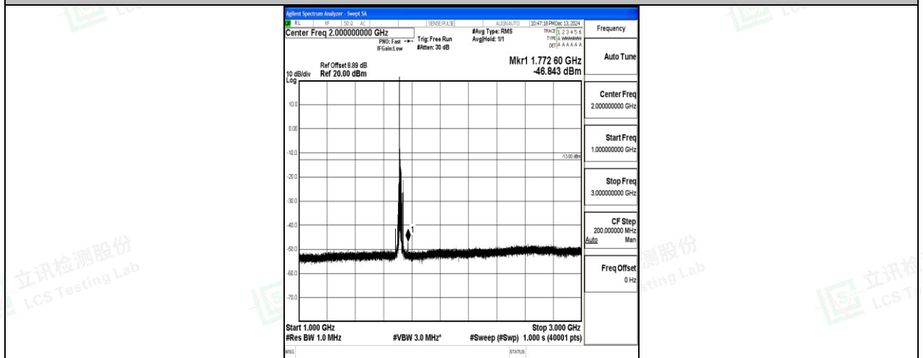
Band66_15MHz_16QAM_132047_1RB#0_1000~3000_1000~3000
