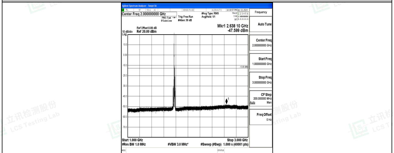
Band66_10MHz_QPSK_132622_1RB#0_1000~3000_1000~3000
