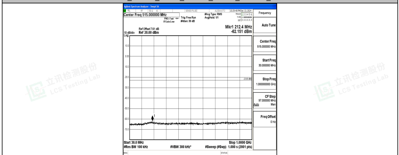
Band66_10MHz_QPSK_132322_1RB#0_30~1000_30~1000
