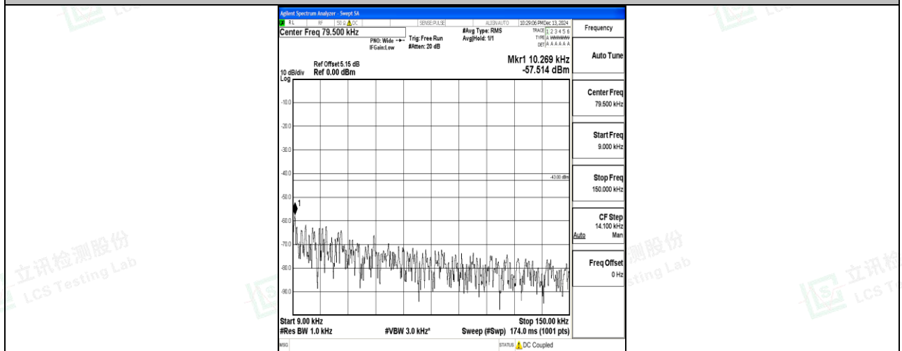
Band66_10MHz_16QAM_132022_1RB#0_0.009~0.15_0.009~0.15
