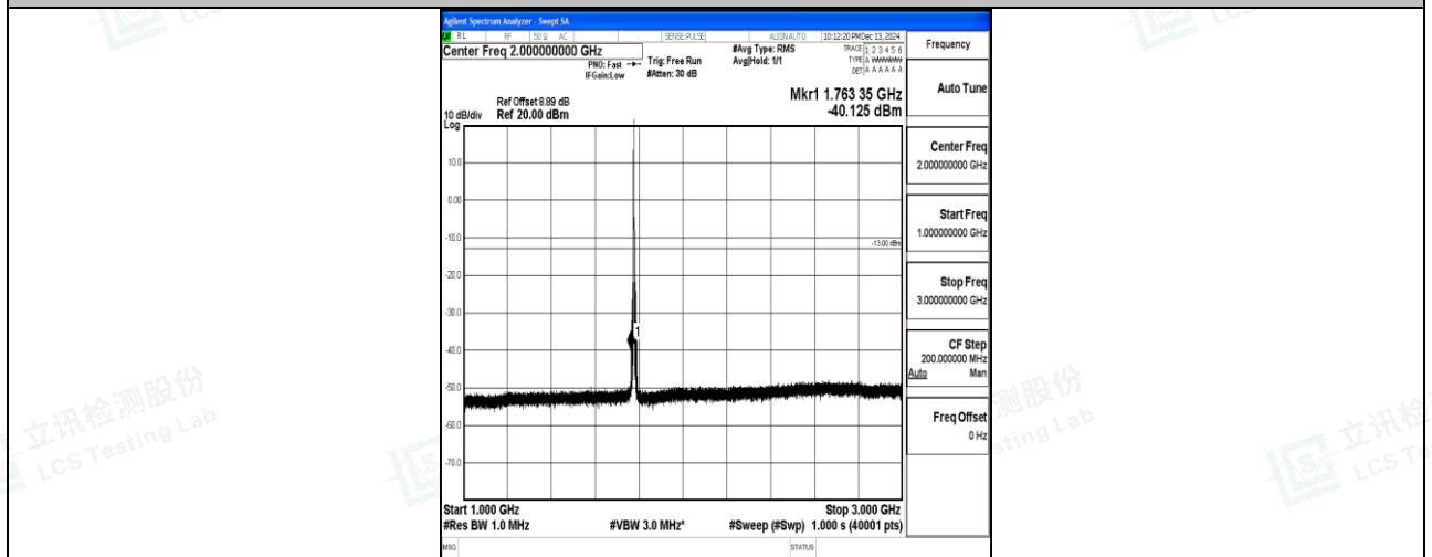
Band66_5MHz_QPSK_132647_1RB#0_1000~3000_1000~3000
