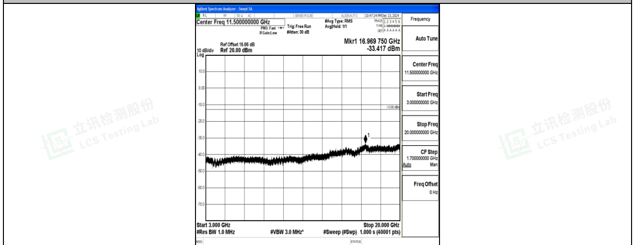
Band66_15MHz_16QAM_132047_1RB#0_3000~20000_3000~20000
