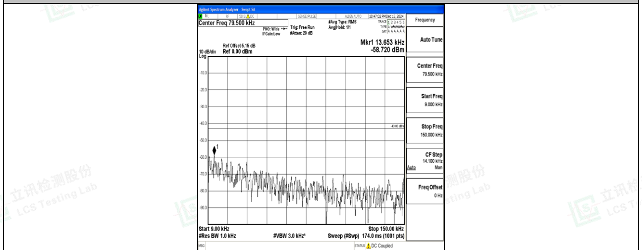
Band66_15MHz_16QAM_132047_1RB#0_0.009~0.15_0.009~0.15
