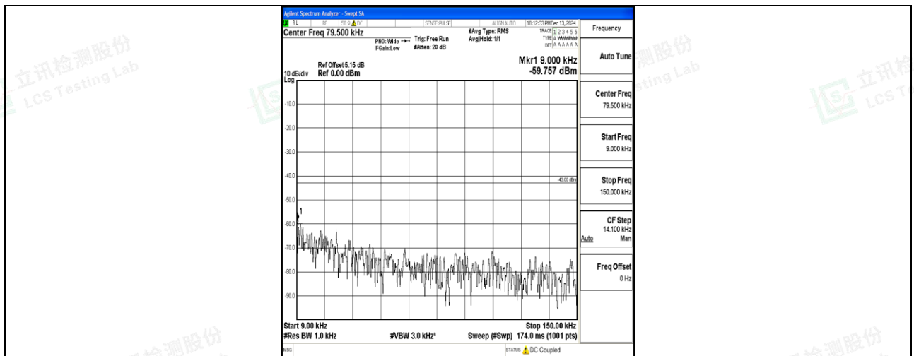
Band66_5MHz_16QAM_132647_1RB#0_0.009~0.15_0.009~0.15
