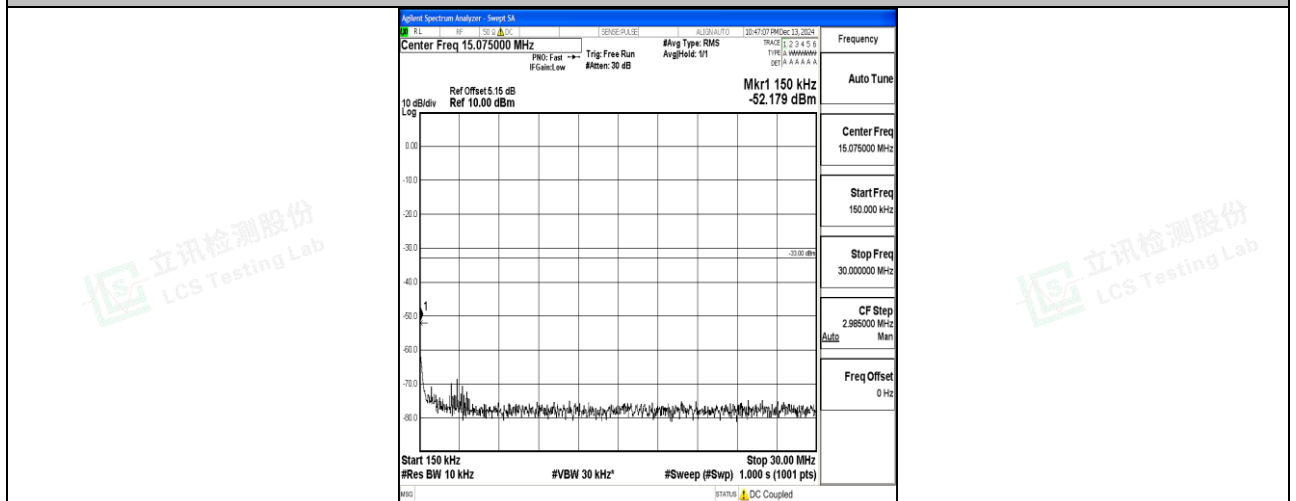
Band66_15MHz_16QAM_132047_1RB#0_0.15~30_0.15~30
