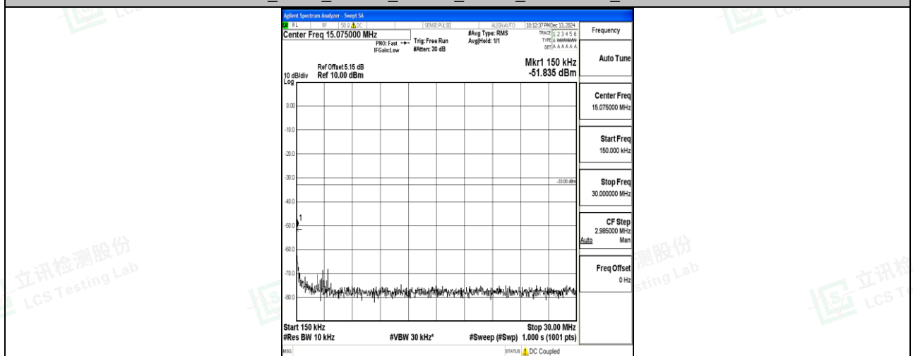
Band66_5MHz_16QAM_132647_1RB#0_0.15~30_0.15~30
