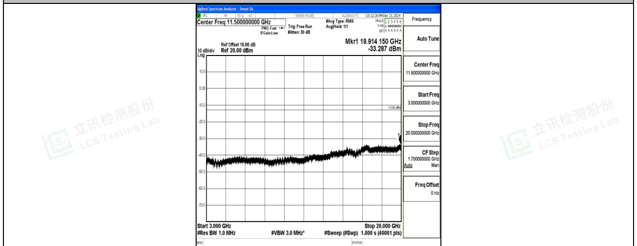
Band66_5MHz_QPSK_132647_1RB#0_3000~20000_3000~20000
