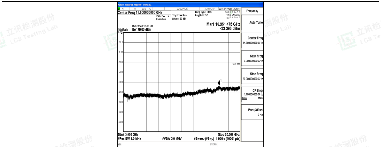
Band66_15MHz_QPSK_132047_1RB#0_3000~20000_3000~20000
