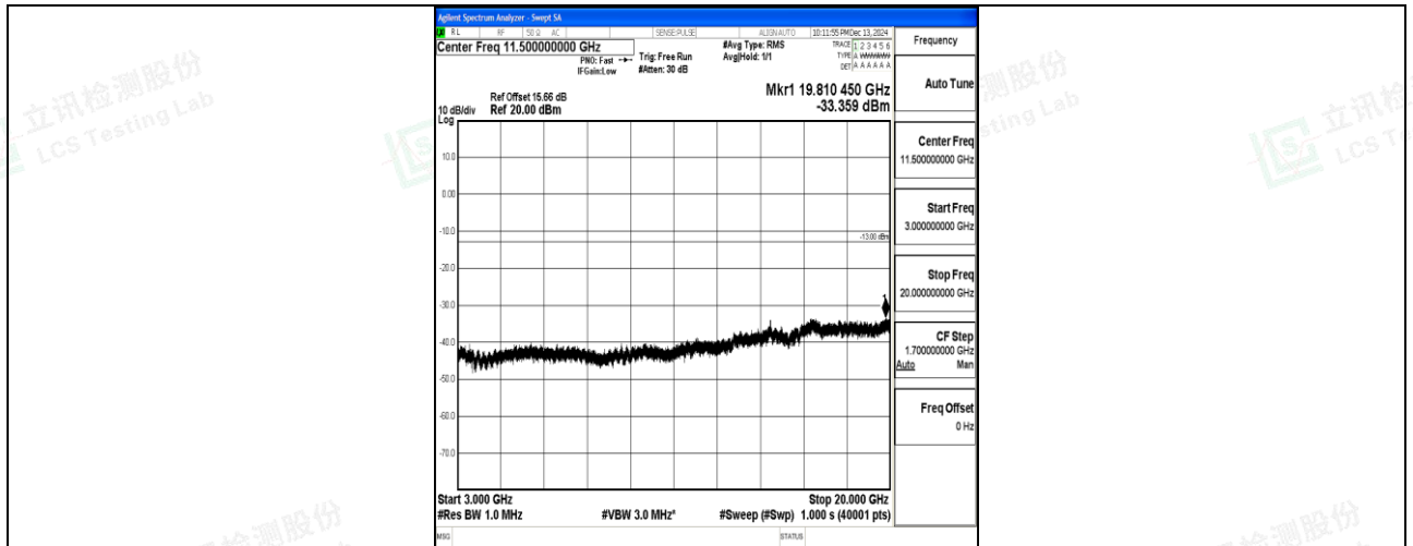
Band66_5MHz_16QAM_132322_1RB#0_3000~20000_3000~20000
