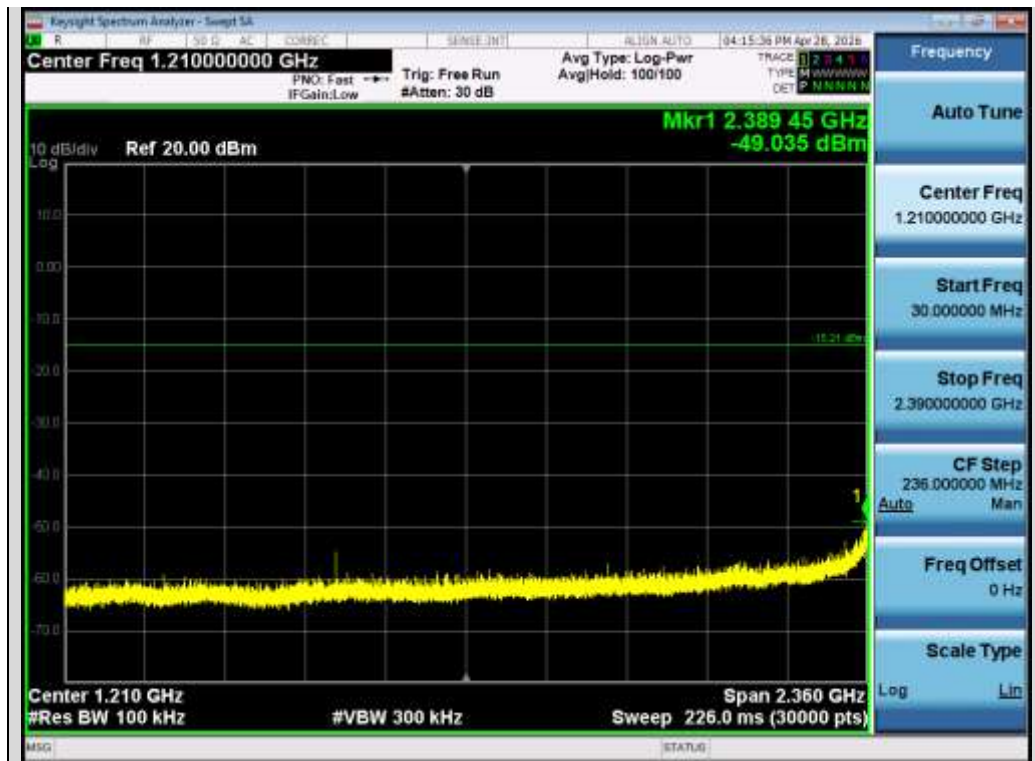
Test_Graph_802.11g_Chain B_2412_6Mbps_Lower Band Emissions
