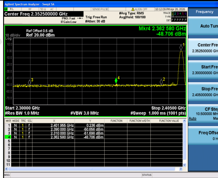
2.4G Ant1 Low 2402 Peak
