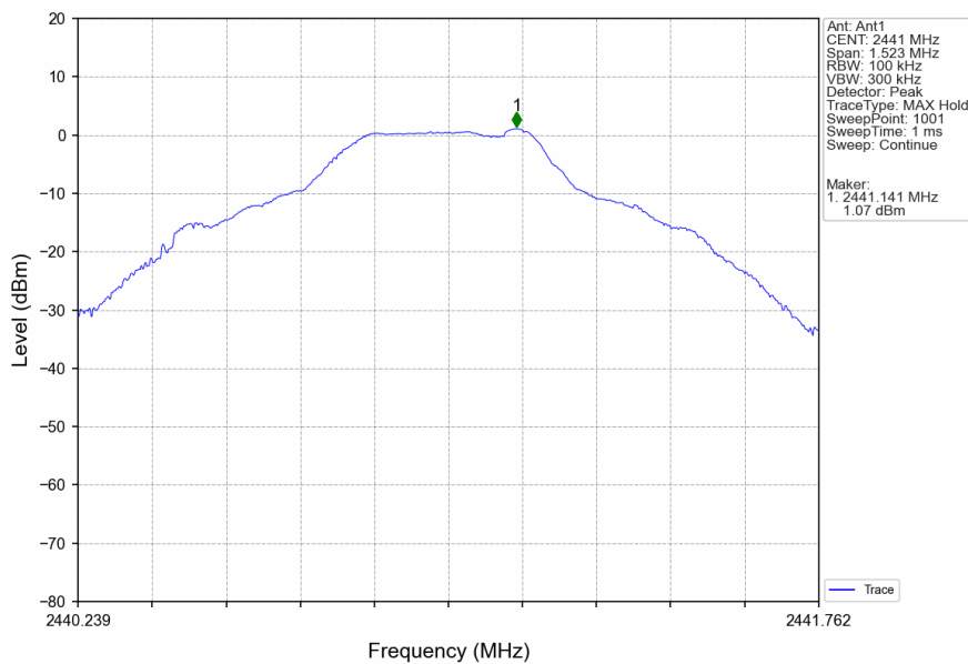
GFSK_DH5_MCH_2441MHz_Ant1_NTNV
