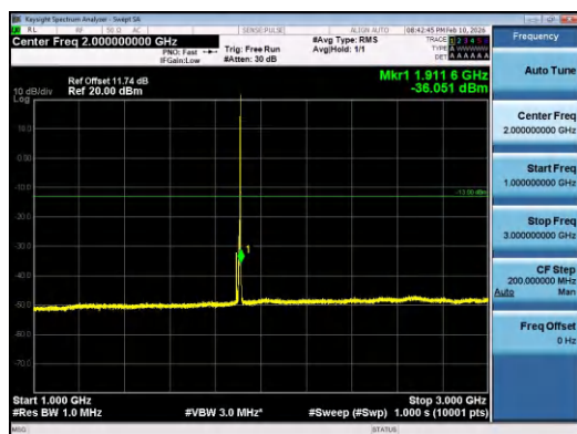
Band2-10MHz-QPSK-19150-1RB#49-1000~3000-PA SS
