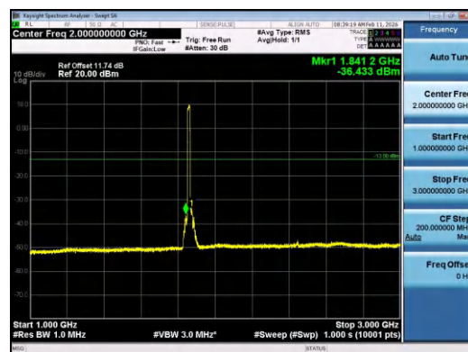
Band2-15MHz-QPSK-18675-75RB#0-1000~3000-PA SS
