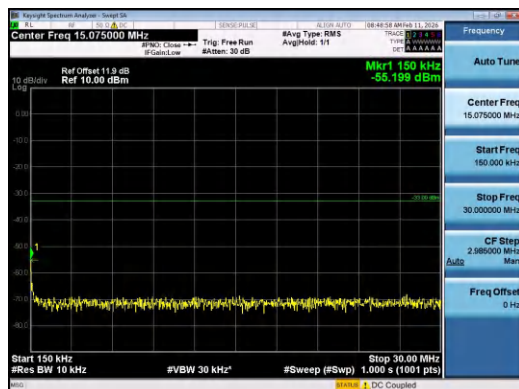
Band2-15MHz-QPSK-19125-1RB#74-0.15~30-PASS
