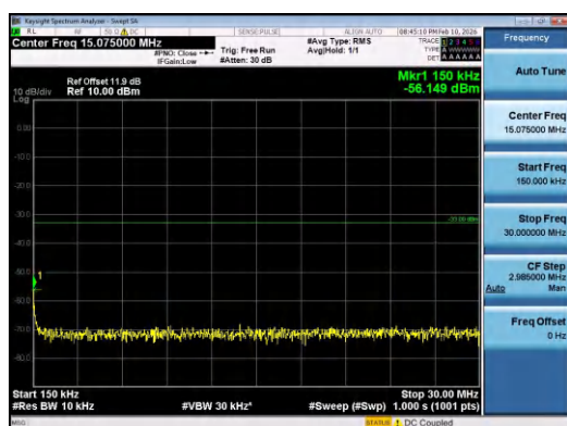
Band2-10MHz-16QAM-19150-50RB#0-0.15~30-PAS S
