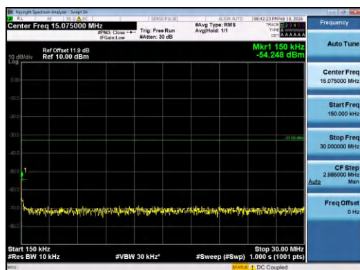
Band2-10MHz-QPSK-19150-1RB#49-0.15~30-PASS
