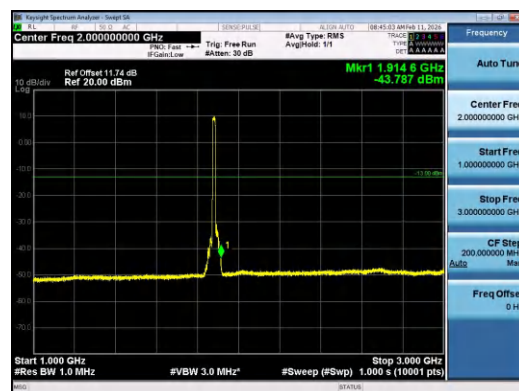
Band2-15MHz-QPSK-18900-75RB#0-1000~3000-PASS SS
