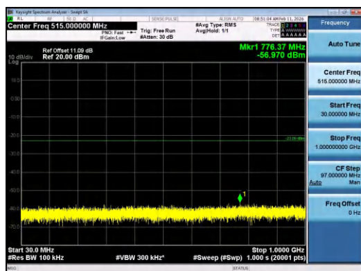
Band2-15MHz-QPSK-19125-75RB#0-30~1000-PASS
