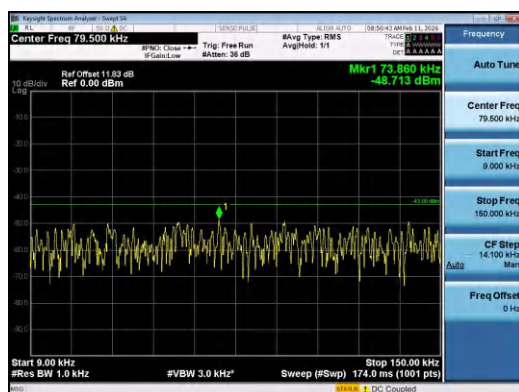
Band2-15MHz-QPSK-19125-75RB#0-0.009~0.15-PA SS
