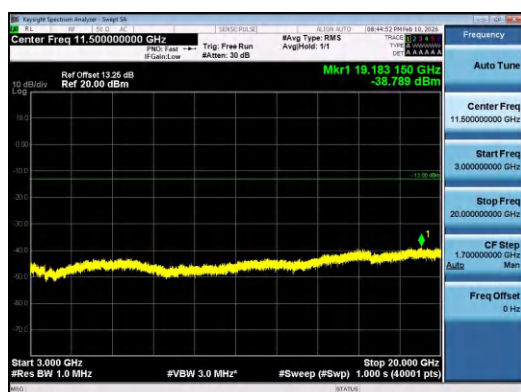
Band2-10MHz-QPSK-19150-50RB#0-3000~20000-PASS
