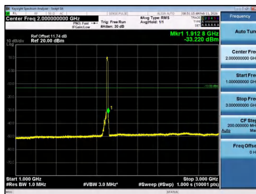
Band2-15MHz-QPSK-19125-75RB#0-1000~3000-PA SS
