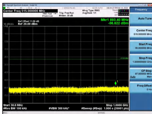
Band2-10MHz-QPSK-19150-50RB#0-30~1000-PASS
