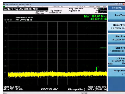
Band2-15MHz-16QAM-18900-1RB#0-30~1000-PASS
