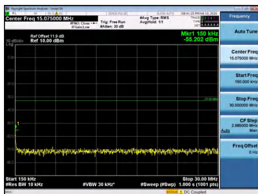
Band2-10MHz-16QAM-19150-1RB#0-0.15~30-PASS
