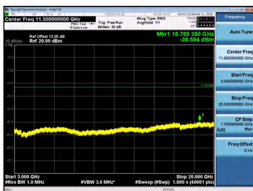
Band2-15MHz-QPSK-18900-75RB#0-3000~20000-PASS ASS
