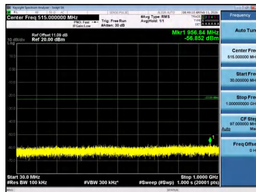
Band2-15MHz-QPSK-19125-1RB#74-30~1000-PASS
