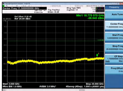
Band2-10MHz-16QAM-19150-1RB#49-3000~20000- PASS
