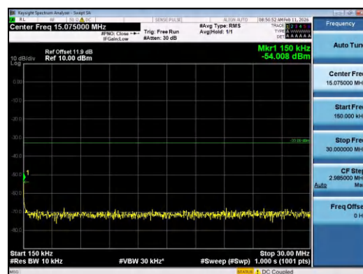
Band2-15MHz-QPSK-19125-75RB#0-0.15~30-PASS
