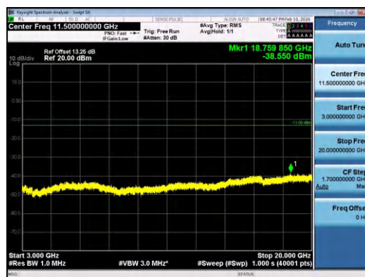
Band2-10MHz-16QAM-19150-50RB#0-3000~20000- PASS
