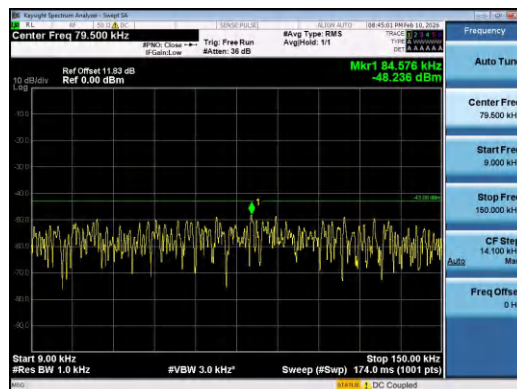
Band2-10MHz-16QAM-19150-50RB#0-0.009~0.15-P ASS
