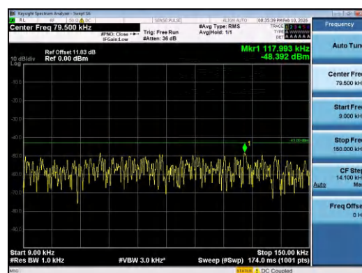
Band2-10MHz-16QAM-18900-1RB#0-0.009~0.15-PA SS
