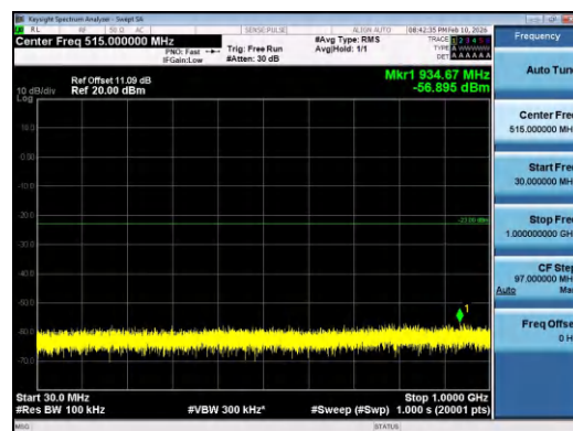
Band2-10MHz-QPSK-19150-1RB#49-30~1000-PASS
