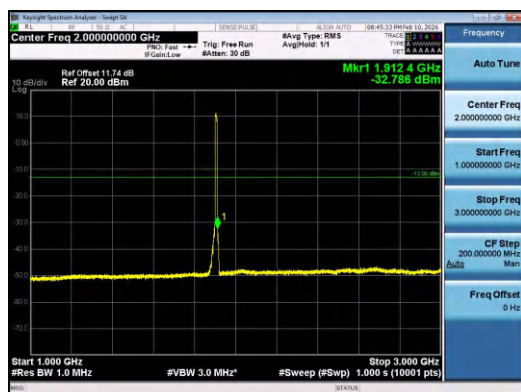
Band2-10MHz-16QAM-19150-50RB#0-1000~3000-P ASS
