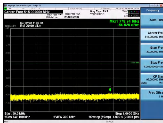
Band2-10MHz-16QAM-18900-1RB#0-30~1000-PASS
