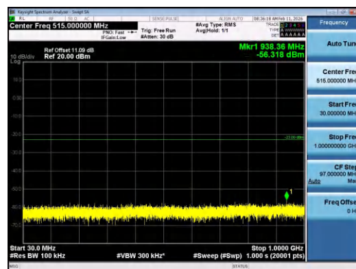
Band2-15MHz-16QAM-18675-1RB#0-30~1000-PASS
