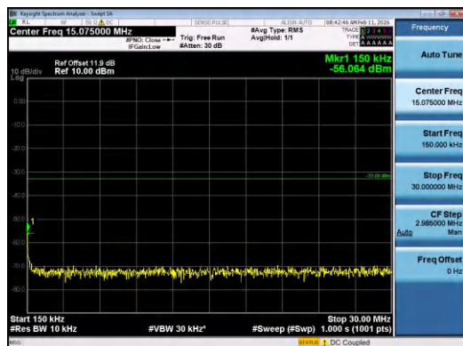
Band2-15MHz-QPSK-18900-1RB#74-0.15~30-PASS
