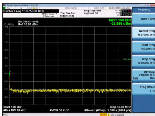
Band2-10MHz-16QAM-18900-1RB#0-0.15~30-PASS
