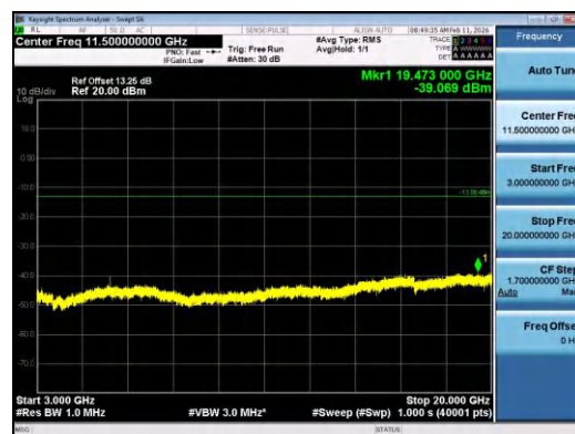
Band2-15MHz-QPSK-19125-1RB#74-3000~20000-P ASS
