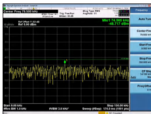
Band2-15MHz-16QAM-19125-1RB#0-0.009~0.15-PA SS
