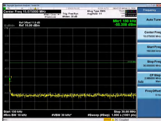
Band2-15MHz-16QAM-19125-1RB#0-0.15~30-PASS
