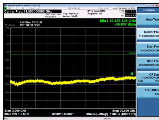
Band2-15MHz-QPSK-18900-1RB#74-3000~20000-P ASS
