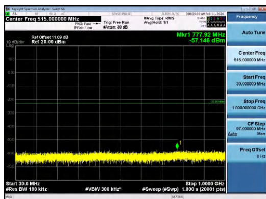
Band2-15MHz-QPSK-18675-75RB#0-30~1000-PASS
