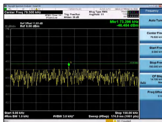
Band2-10MHz-16QAM-19150-1RB#0-0.009~0.15-PASS
