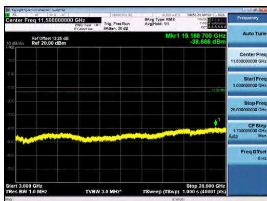
Band2-15MHz-QPSK-19125-75RB#0-3000~20000-P ASS
