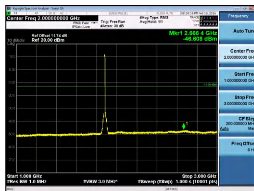
Band2-10MHz-QPSK-18900-50RB#0-1000~3000-PA SS
