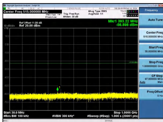
Band2-10MHz-QPSK-18900-50RB#0-30~1000-PASS
