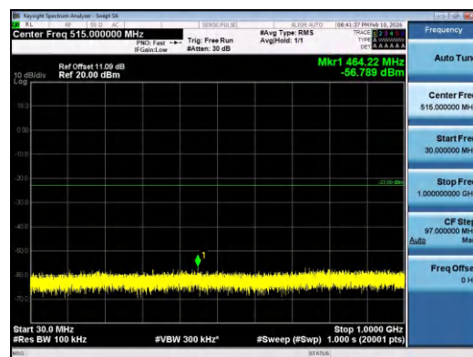
Band2-10MHz-16QAM-19150-1RB#0-30~1000-PASS
