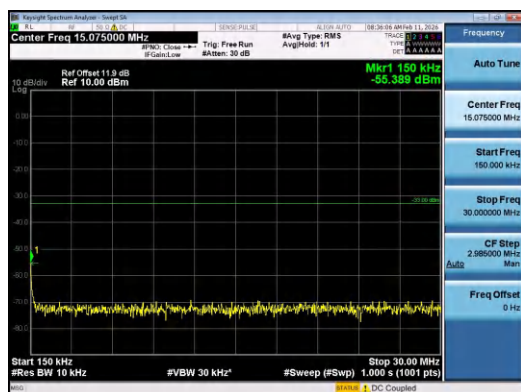
Band2-15MHz-16QAM-18675-1RB#0-0.15~30-PASS
