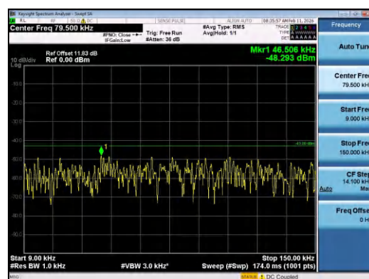
Band2-15MHz-16QAM-18675-1RB#0-0.009~0.15-PA SS
