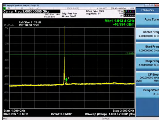
Band2-15MHz-QPSK-18900-1RB#74-1000~3000-PA SS
