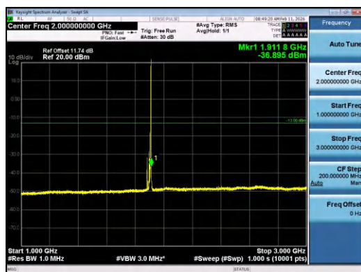
Band2-15MHz-QPSK-19125-1RB#74-1000~3000-PA SS
