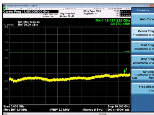
Band2-15MHz-QPSK-18675-75RB#0-3000~20000-P ASS
