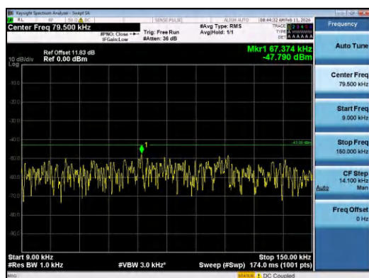
Band2-15MHz-QPSK-18900-75RB#0-0.009~0.15-PA SS
