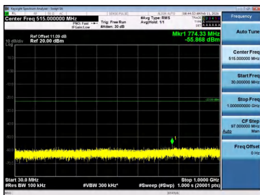
Band2-15MHz-QPSK-18900-75RB#0-30~1000-PASS
