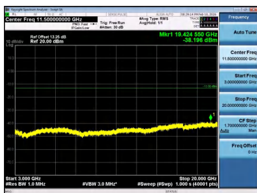
Band2-10MHz-QPSK-18900-50RB#0-3000~20000-P ASS
