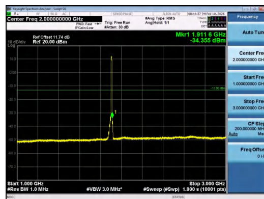
Band2-10MHz-QPSK-19150-50RB#0-1000~3000-PASS
