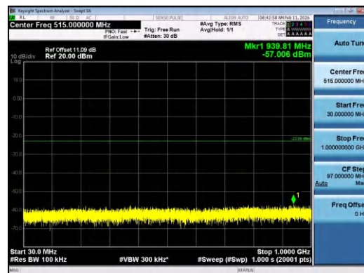
Band2-15MHz-QPSK-18900-1RB#74-30~1000-PASS
