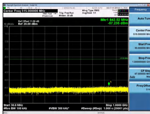
Band2-15MHz-16QAM-19125-1RB#0-30~1000-PASS
