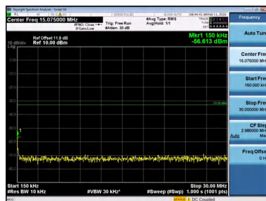
Band2-15MHz-QPSK-18900-75RB#0-0.15~30-PASS
