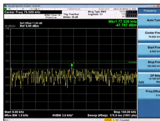
Band2-15MHz-16QAM-18900-1RB#0-0.009~0.15-PASS SS
