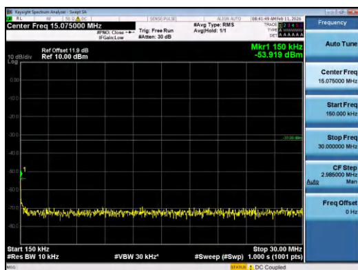
Band2-15MHz-16QAM-18900-1RB#0-0.15~30-PASS
