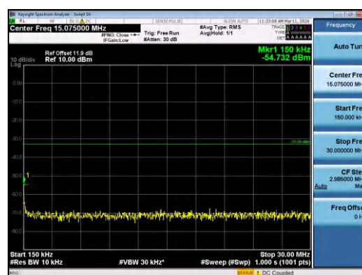
Band4-3MHz-QPSK-19965-15RB#0-0.15~30-PASS
