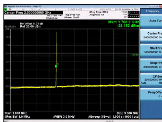
Band4-3MHz-QPSK-19965-15RB#0-1000~3000-PAS
