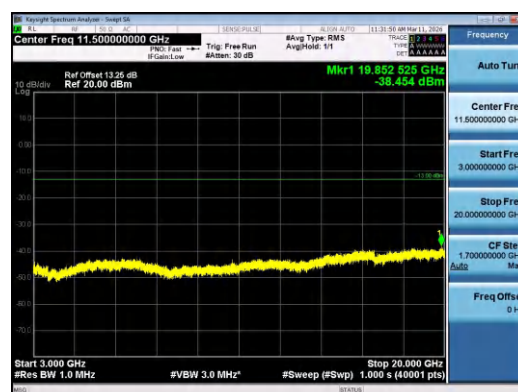
Band4-3MHz-QPSK-19965-1RB#14-3000~20000-PAS
