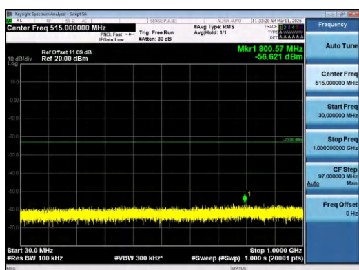
Band4-3MHz-QPSK-19965-15RB#0-30~1000-PASS
