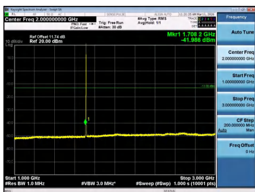
Band4-3MHz-QPSK-19965-1RB#14-1000~3000-PAS
