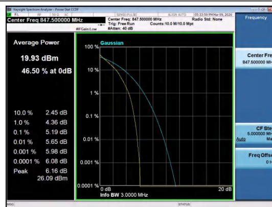
Band5-3MHz-16QAM-20635-15RB#0-PASS
