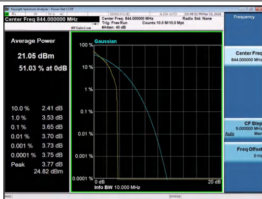
Band5-10MHz-QPSK-20600-1RB#0-PASS
