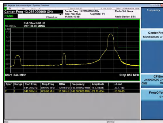
Band5-5MHz-QPSK-20625-1RB#24-PASS
