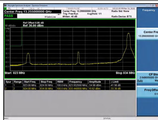
Band5-10MHz-QPSK-20450-1RB#49-PASS
