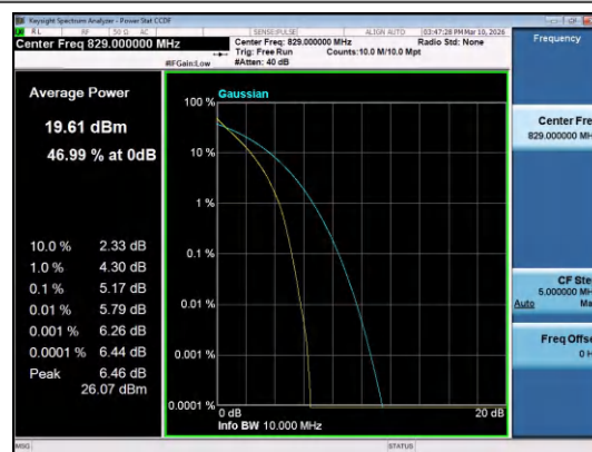
Band5-10MHz-16QAM-20450-50RB#0-PASS
