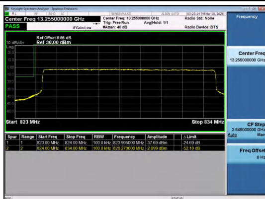
Band5-10MHz-QPSK-20450-50RB#0-PASS
