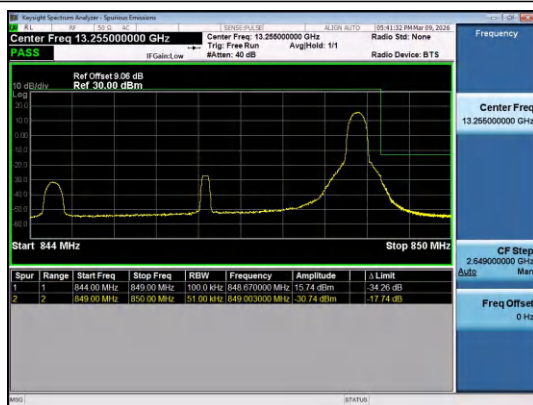
Band5-5MHz-16QAM-20625-1RB#24-PASS
