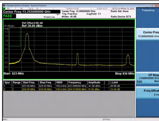
Band5-10MHz-QPSK-20450-1RB#0-PASS
