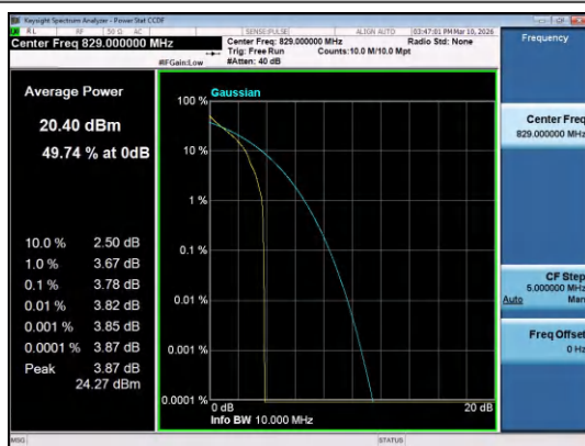
Band5-10MHz-16QAM-20450-1RB#0-PASS
