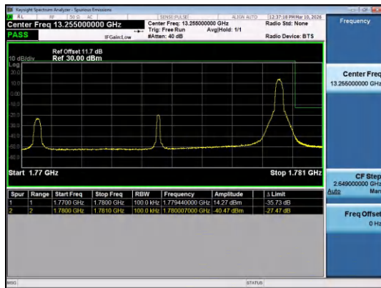
Band66-10MHz-16QAM-132622-1RB#49-PASS
