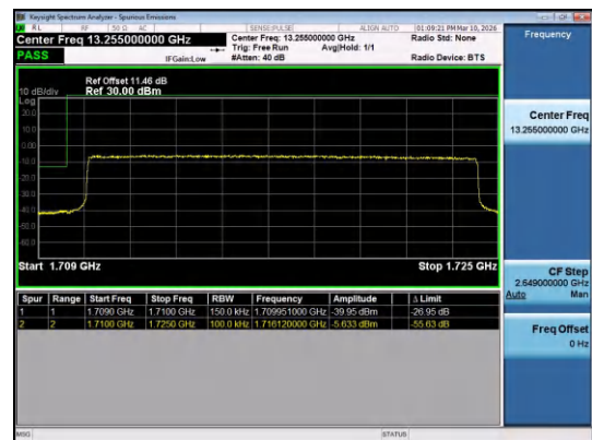
Band66-15MHz-16QAM-132047-75RB#0-PASS
