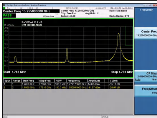
Band66-15MHz-16QAM-132597-1RB#74-PASS
