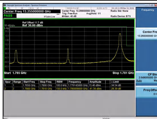
Band66-15MHz-QPSK-132597-1RB#74-PASS
