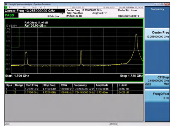
Band66-15MHz-QPSK-132047-1RB#74-PASS
