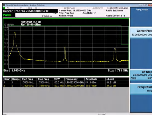
Band66-15MHz-QPSK-132597-1RB#0-PASS
