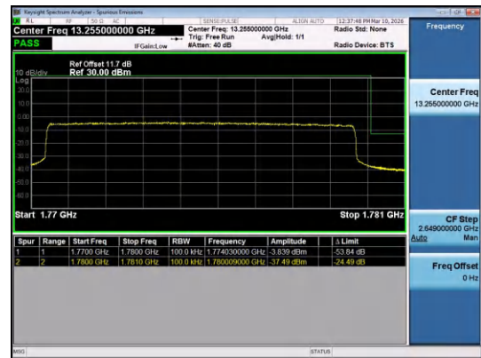
Band66-10MHz-16QAM-132622-50RB#0-PASS
