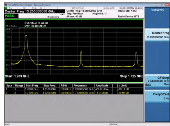
Band66-15MHz-16QAM-132047-1RB#0-PASS
