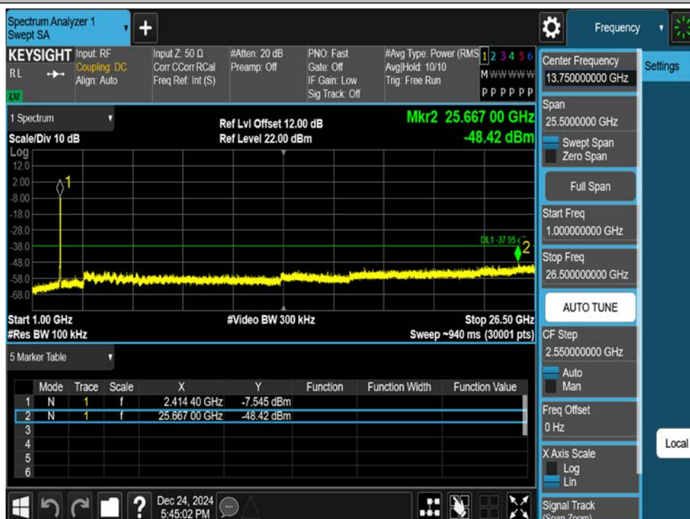
11G-Ant1-2412-1000~26500-PASS
