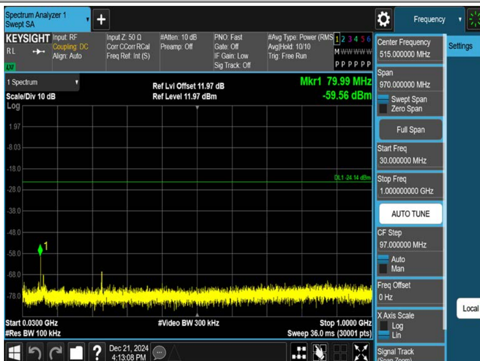
11B-Ant1-2462-30~1000-PASS
