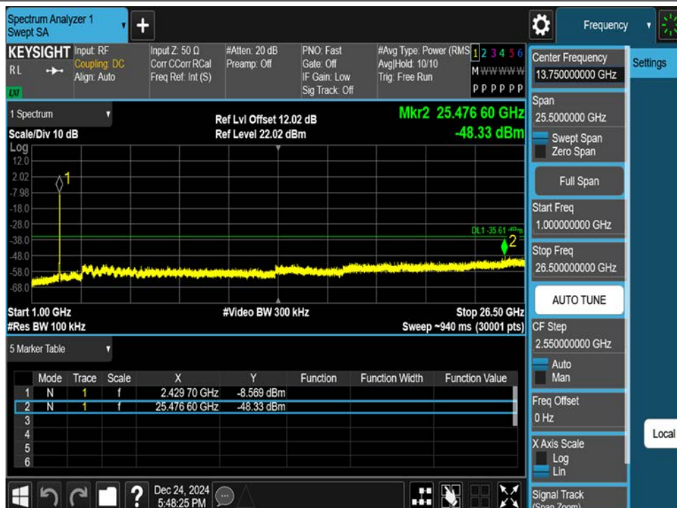
11N20SISO-Ant1-2437-1000~26500-PASS
