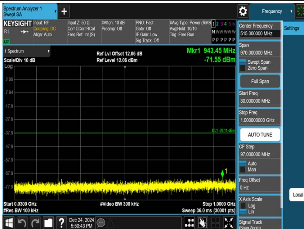
11N40SISO-Ant1-2452-30~1000-PASS
