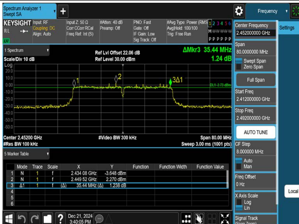
11N40SISO-Ant1-2452-PASS
