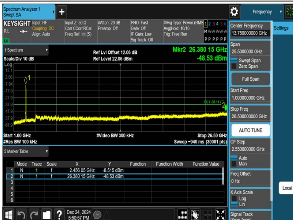
11N40SISO-Ant1-2452-1000~26500-PASS
