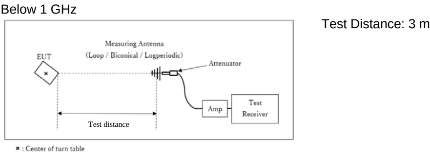
Figure 2: Test Setup
