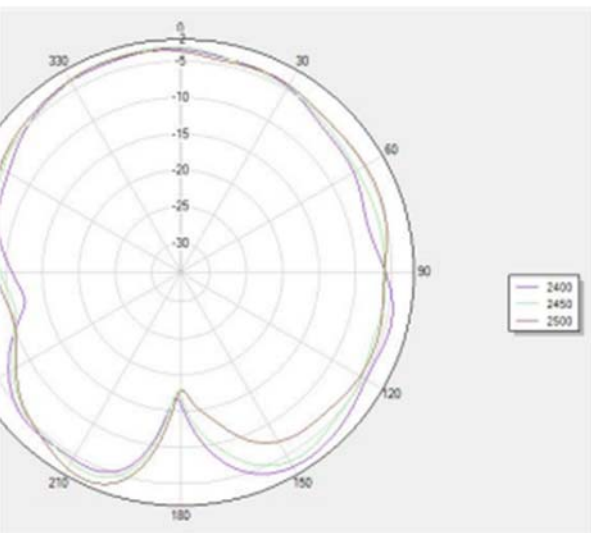
Phi 0 2 D Figure
