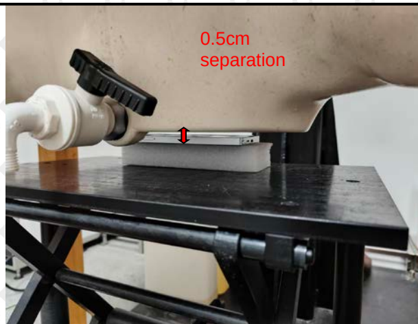
Body/ Hotspot (Front Side)
