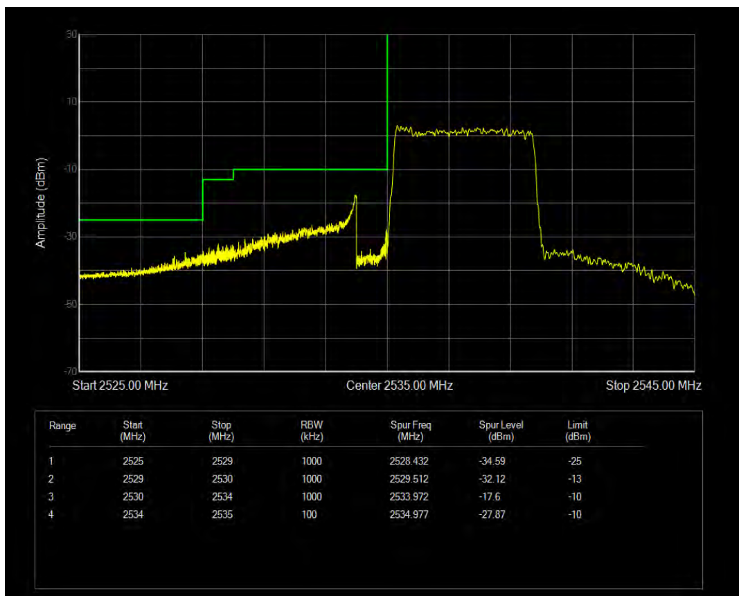
Band41(2535-2675) QPSK BW=5MHz Channel=40065 RB Size=25 Position=#0
