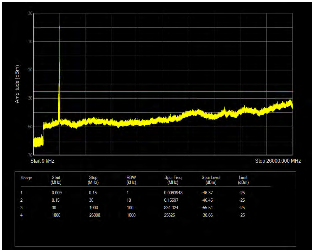
Band41(2535-2675) QPSK BW=15MHz Channel=40115 RB Size=75 Position=#0
