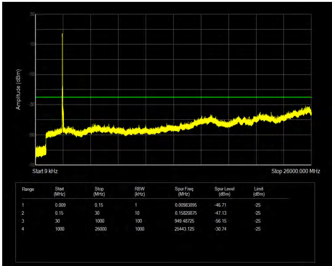
Band41(2535-2675) QPSK BW=15MHz Channel=41365 RB Size=75 Position=#0
