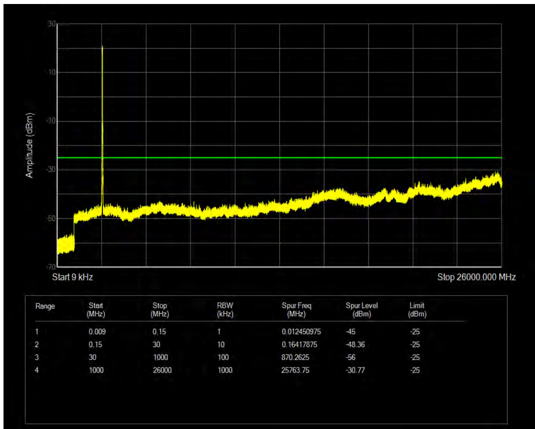
Band41(2535-2675) QAM16 BW=15MHz Channel=41365 RB Size=75 Position=#0
