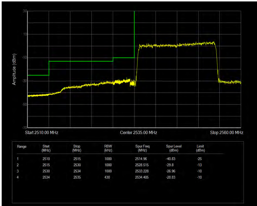
Band41(2535-2675) QAM16 BW=20MHz Channel=40140 RB Size=100 Position=#0
