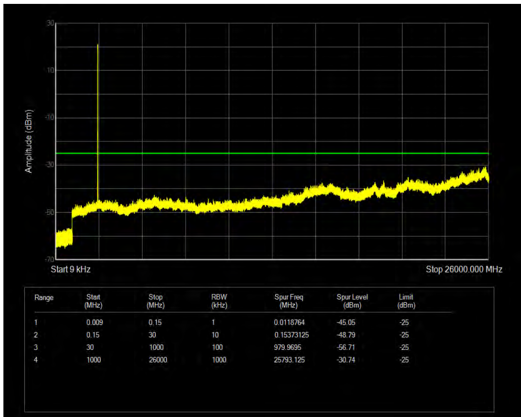
Band41(2535-2675) QPSK BW=5MHz Channel=40065 RB Size=25 Position=#0
