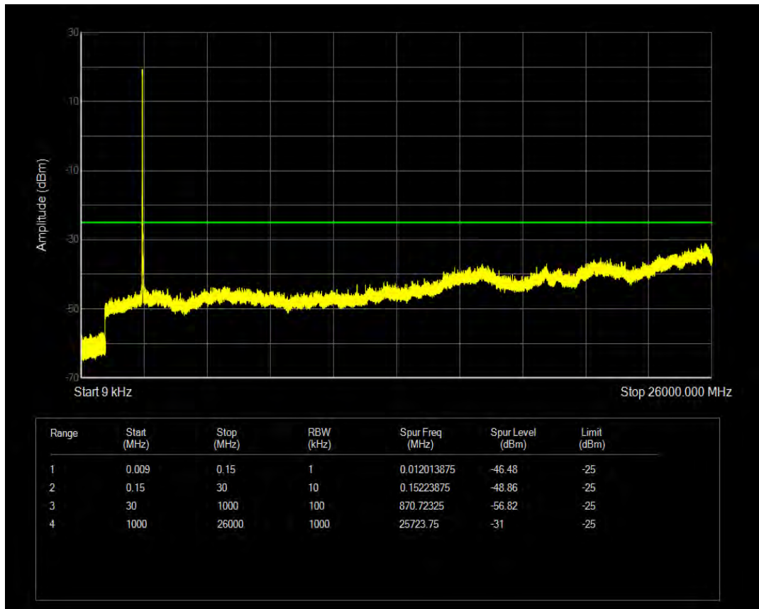
Band41(2535-2675) QPSK BW=10MHz Channel=41390 RB Size=50 Position=#0
