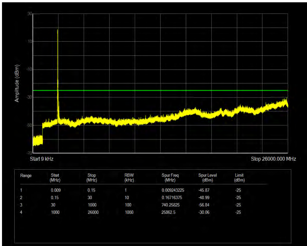
Band41(2535-2675) QAM16 BW=15MHz Channel=40115 RB Size=75 Position=#0
