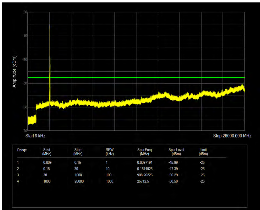
Band41(2535-2675) QPSK BW=20MHz Channel=41340 RB Size=100 Position=#0
