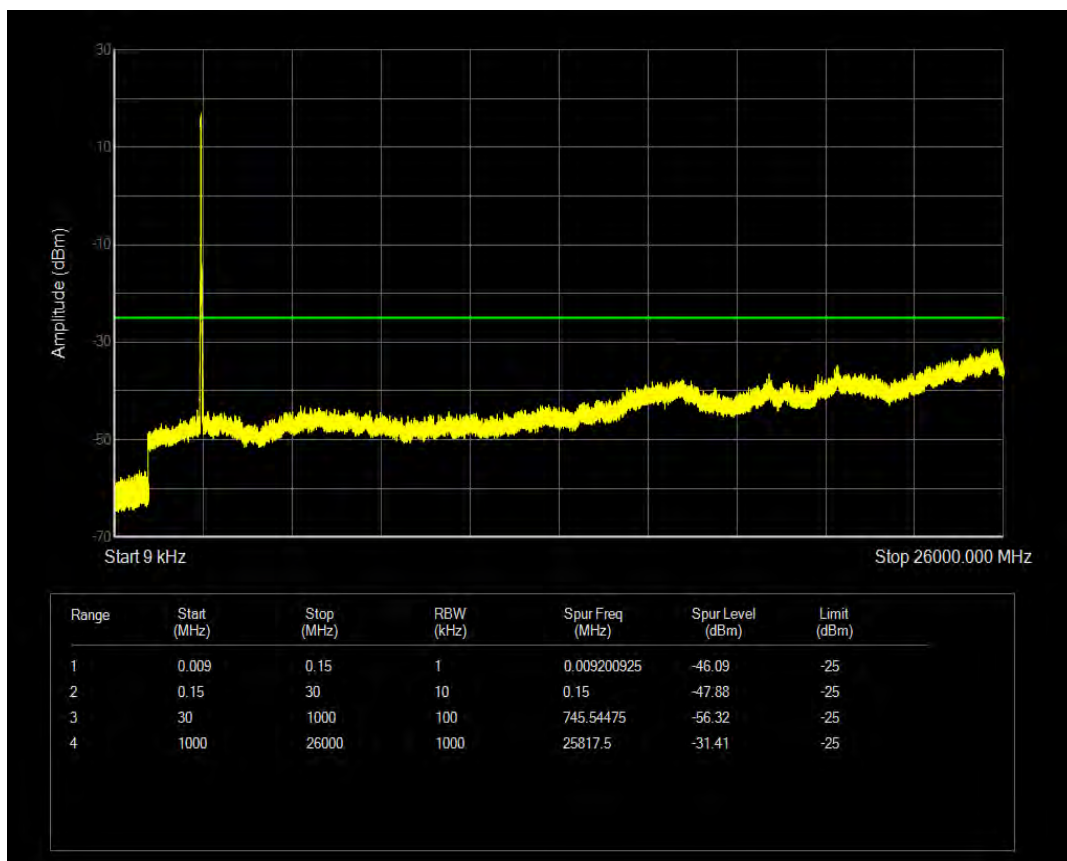
Band41(2535-2675) QAM16 BW=20MHz Channel=41340 RB Size=100 Position=#0
