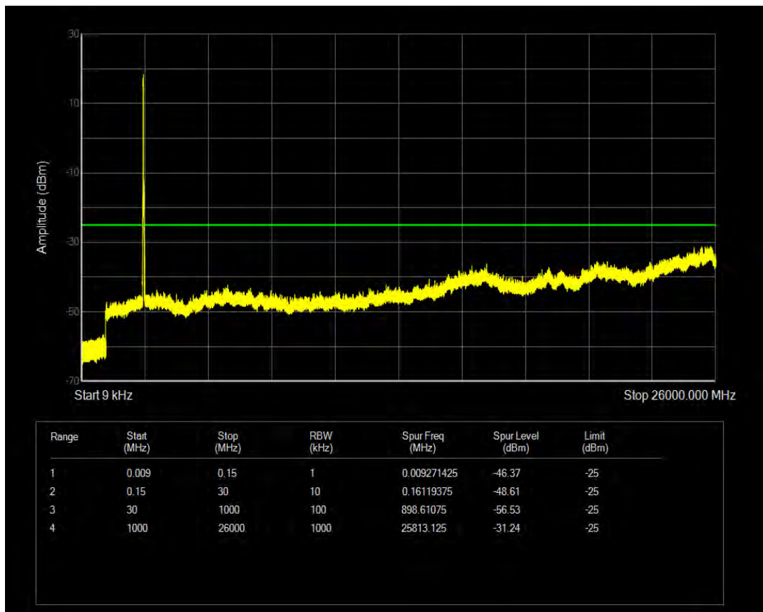
Band41(2535-2675) QAM16 BW=20MHz Channel=40140 RB Size=100 Position=#0
