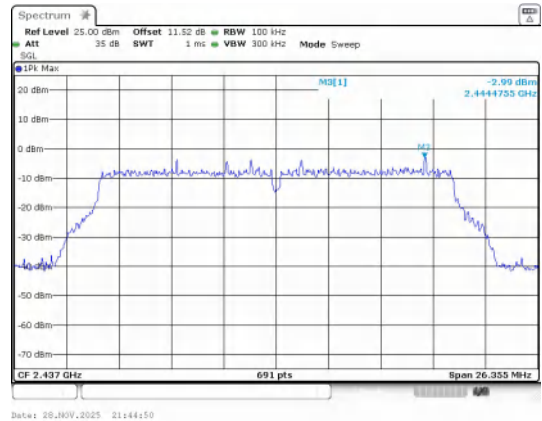
In-Band Reference Level IEEE 802.11n_Channel 6_20MHz_Antenna 1
