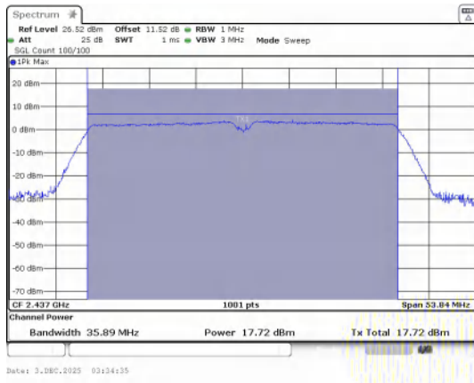
Conducted Output Power IEEE 802.11n_40_Channel 6_Antenna 1
