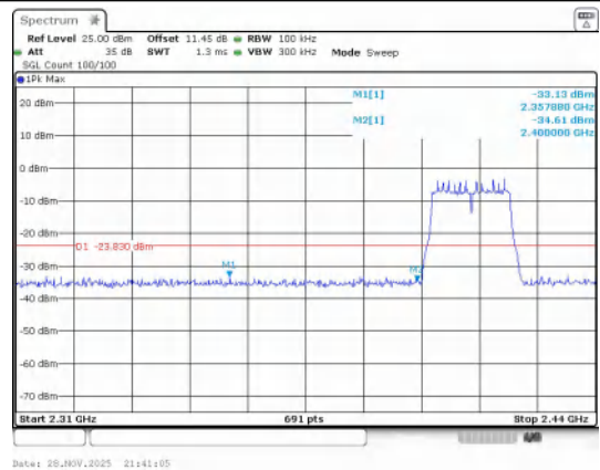
Out Of Band Emission IEEE 802.11n_Channel 1_20MHz_Antenna 1
