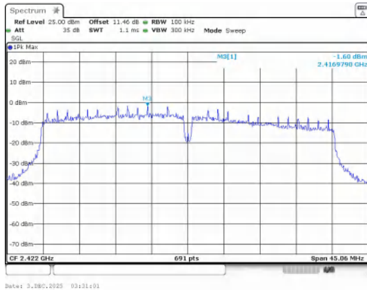
In-Band Reference Level IEEE 802.11n_Channel 3_40MHz_Antenna 1
