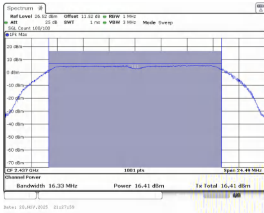
Conducted Output Power IEEE 802.11g_Channel 6_Antenna 1
