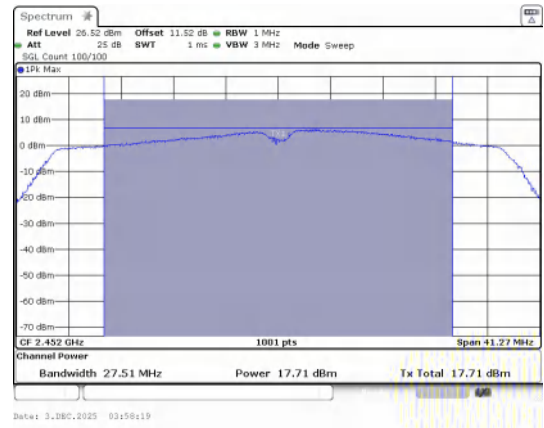
Conducted Output Power IEEE 802.11n_Channel 9_Antenna 0
