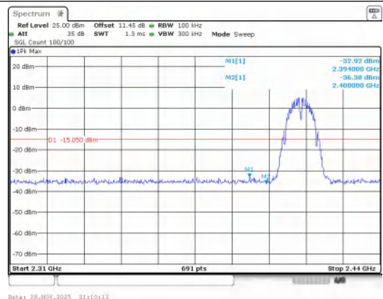
Out Of Band Emission IEEE 802.11b_Channel 1_20MHz_Antenna 1
