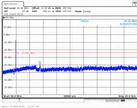
30.0 MHz - 25000.0 MHz IEEE 802.11n_Channel 1_20MHz_Antenna 1
