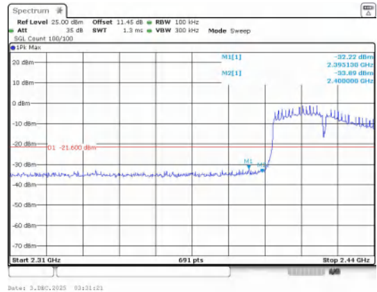
Out Of Band Emission IEEE 802.11n_Channel 3_40MHz_Antenna 1
