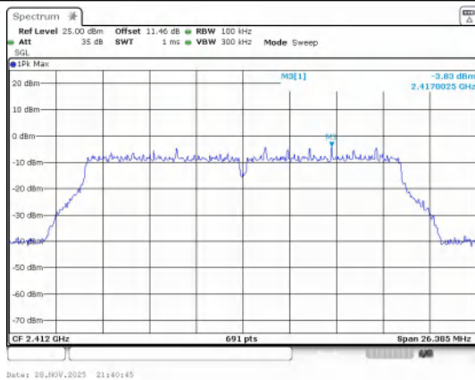
In-Band Reference Level IEEE 802.11n_Channel 1_20MHz_Antenna 1
