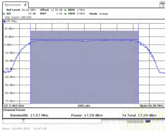
Conducted Output Power IEEE 802.11n_20_Channel 11_Antenna 1
