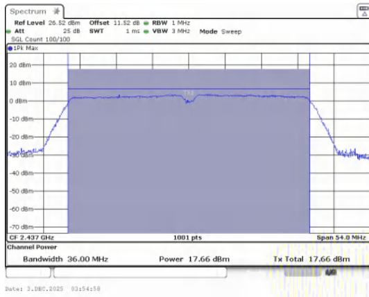
Conducted Output Power IEEE 802.11n_Channel 6_Antenna 0
