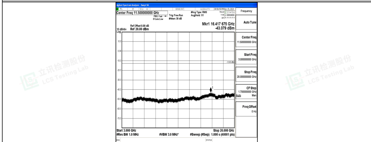
Band2-5MHz-16QAM-18900-1RB#0-3000~20000-PASS
