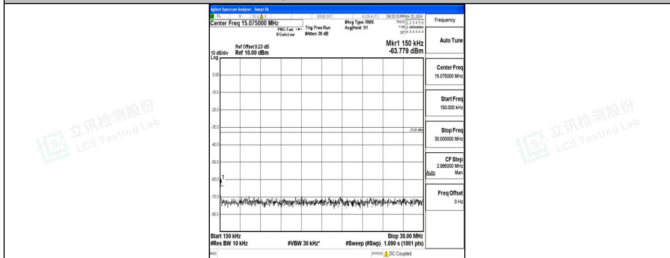
Band2-3MHz-16QAM-18900-1RB#0-0.15~30-PASS
