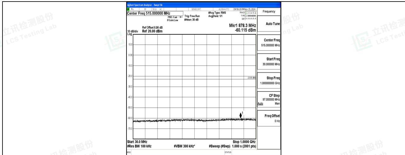
Band2-5MHz-16QAM-18900-1RB#0-30~1000-PASS
