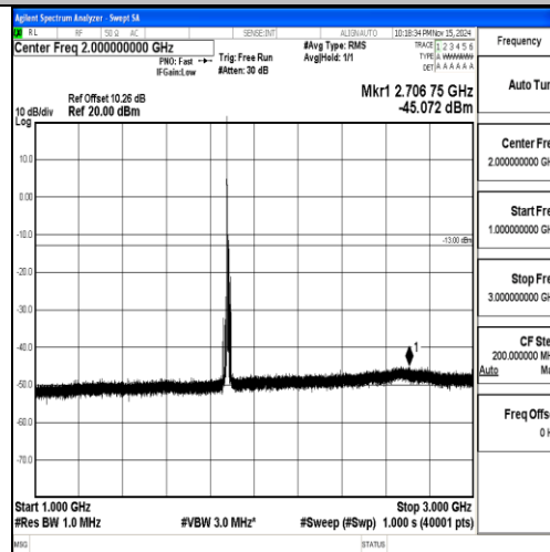
Band2-10MHz-QPSK-18900-1RB#0-1000~3000-PASS
