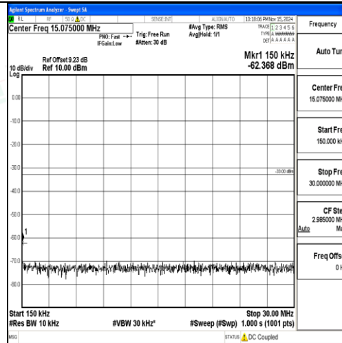
Band2-10MHz-QPSK-18900-1RB#0-0.15~30-PASS
