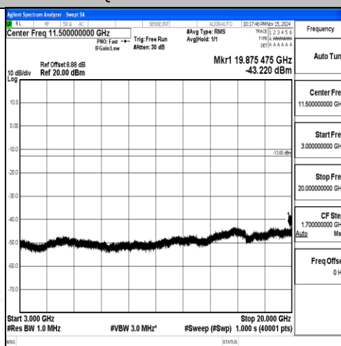
Band2-10MHz-16QAM-18650-1RB#0-3000~20000-PASS
