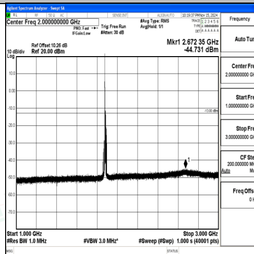
Band2-10MHz-16QAM-18900-1RB#0-1000~3000-PASS
