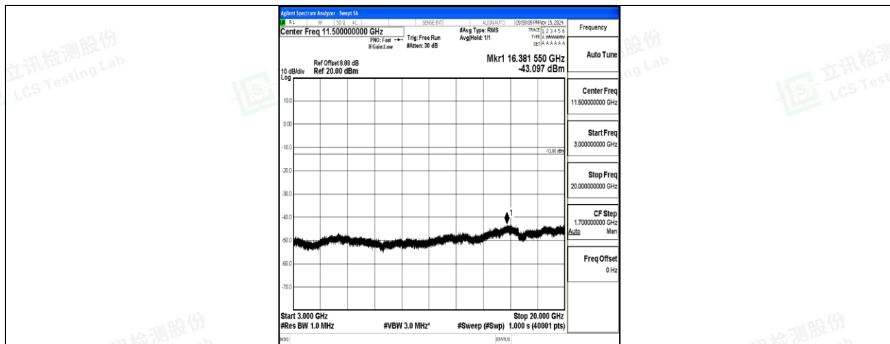
Band2-5MHz-16QAM-19175-1RB#0-3000~20000-PASS
