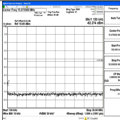
Band2-3MHz-QPSK-18900-1RB#0-0.15~30-PASS
