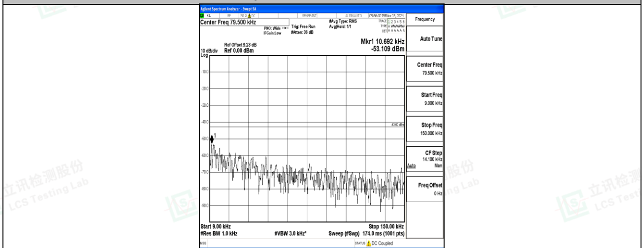
Band2-5MHz-16QAM-18900-1RB#0-0.009~0.15-PASS
