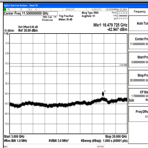
Band2-10MHz-16QAM-18900-1RB#0-3000~20000-PASS
