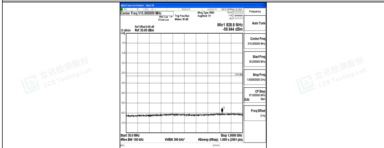
Band2-3MHz-16QAM-18615-1RB#0-30~1000-PASS
