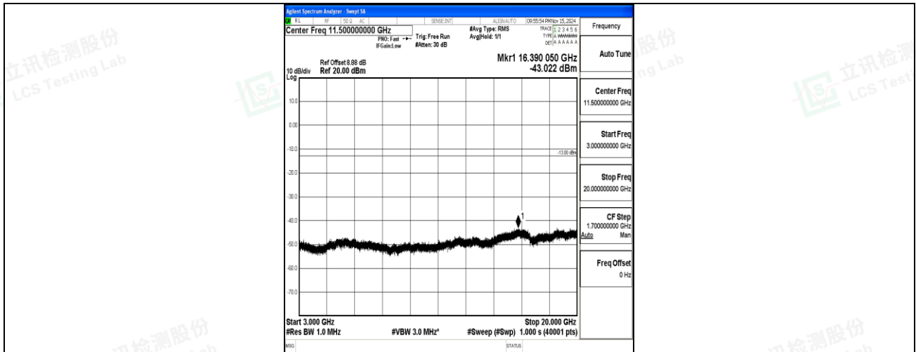
Band2-5MHz-QPSK-18900-1RB#0-3000~20000-PASS
