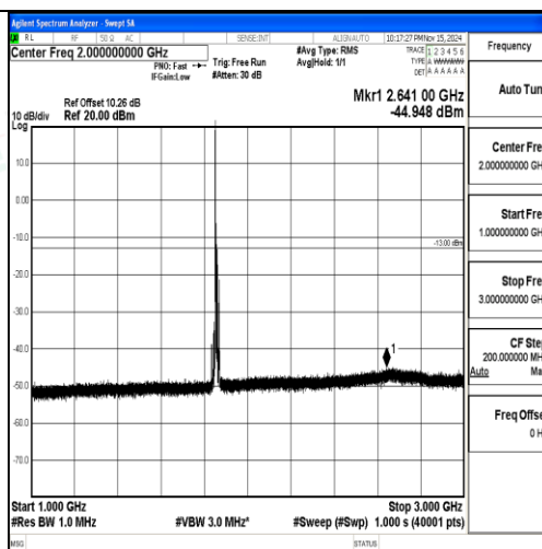
Band2-10MHz-16QAM-18650-1RB#0-1000~3000-PASS
