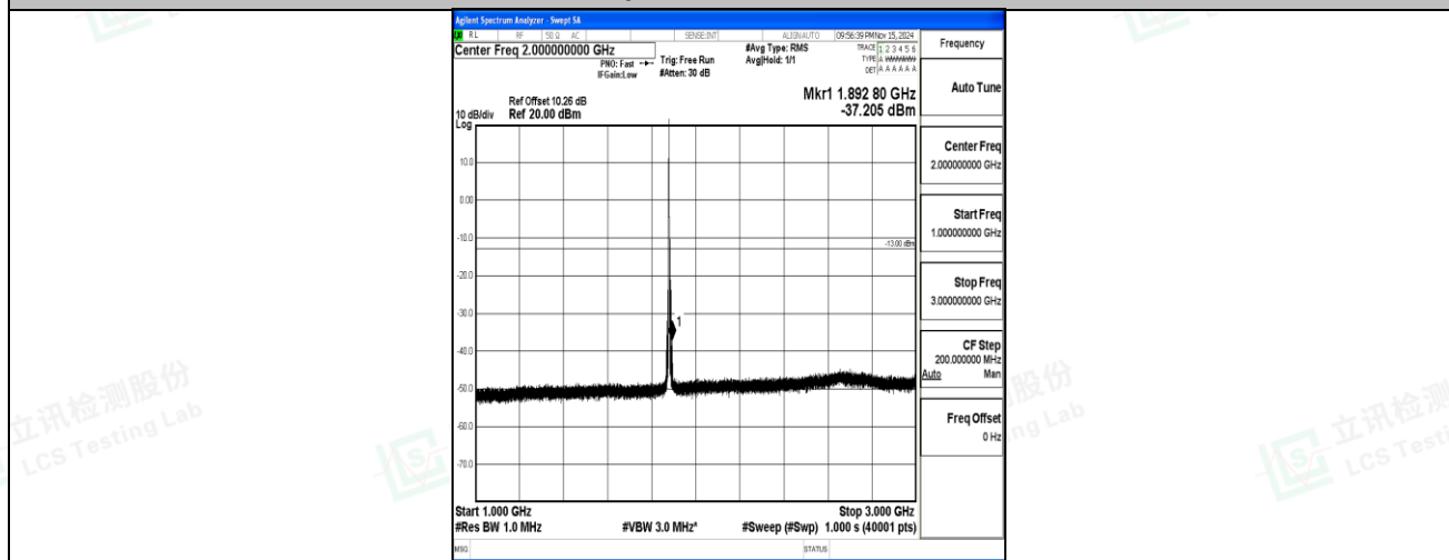
Band2-5MHz-16QAM-18900-1RB#0-1000~3000-PASS
