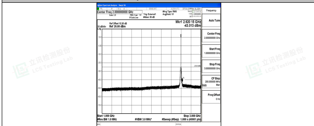
Band38-10MHz-16QAM-38000-50RB#0-1000~3000-PASS
