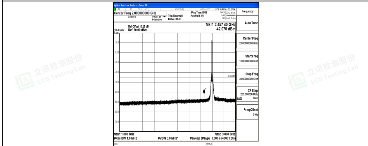
Band38-15MHz-QPSK-38000-75RB#0-1000~3000-PASS
