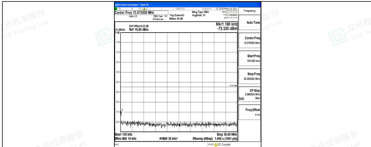
Band38-10MHz-16QAM-38200-50RB#0-0.15~30-PASS
