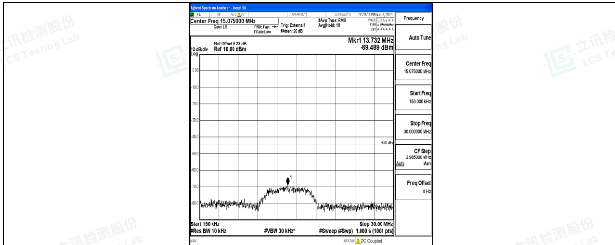
Band38-10MHz-QPSK-37800-50RB#0-0.15~30-PASS
