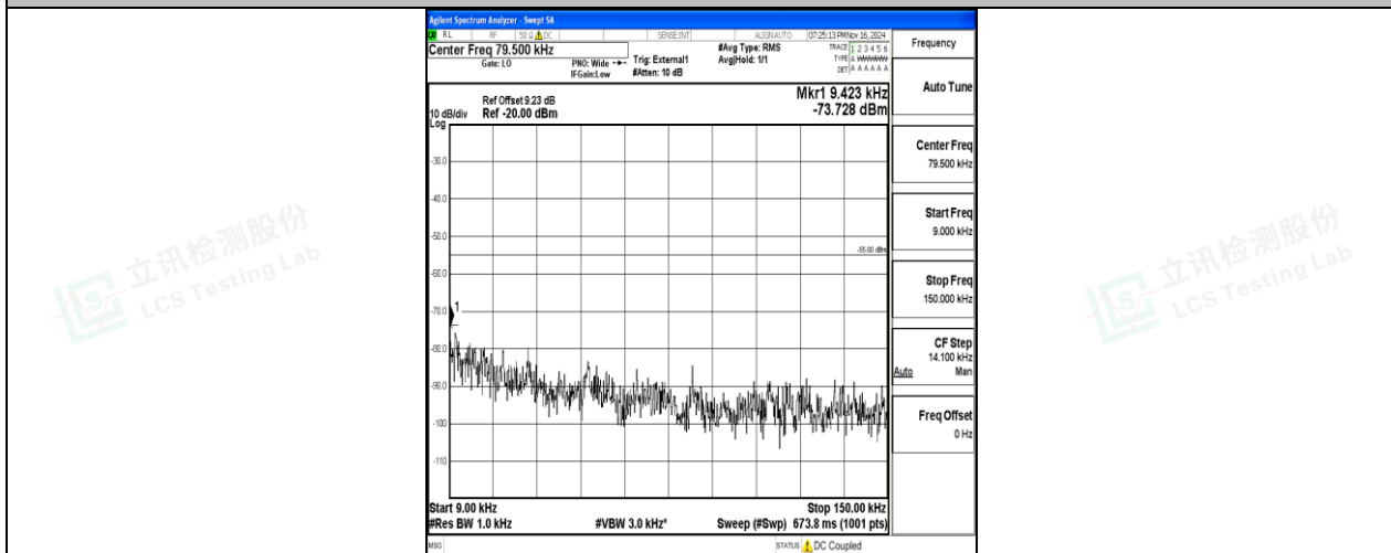
Band38-10MHz-16QAM-37800-50RB#0-0.009~0.15-PASS
