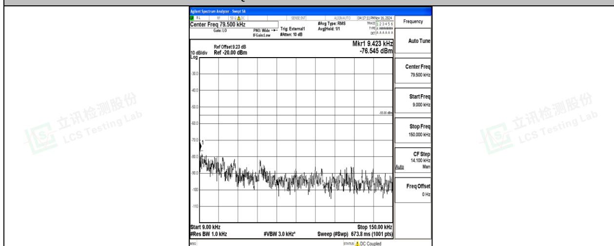
Band38-5MHz-16QAM-38000-25RB#0-0.009~0.15-PASS
