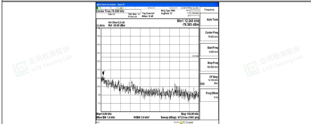
Band38-15MHz-QPSK-38000-75RB#0-0.009~0.15-PASS
