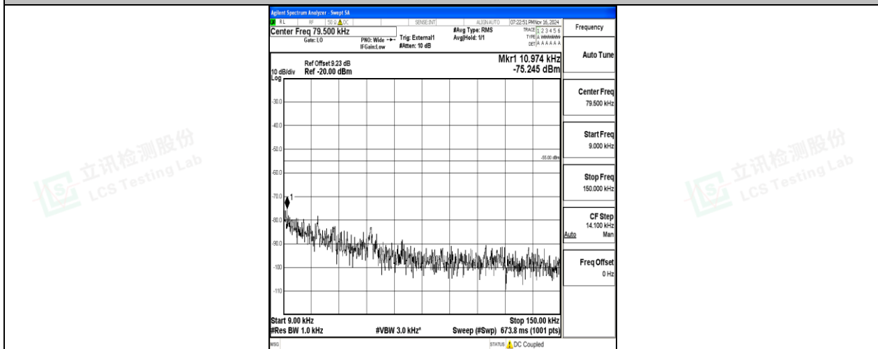
Band38-10MHz-QPSK-37800-50RB#0-0.009~0.15-PASS
