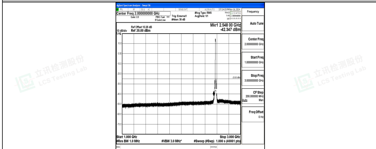
Band38-10MHz-QPSK-37800-50RB#0-1000~3000-PASS
