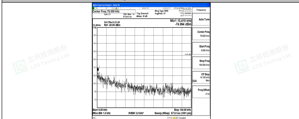
Band38-10MHz-QPSK-38200-50RB#0-0.009~0.15-PASS
