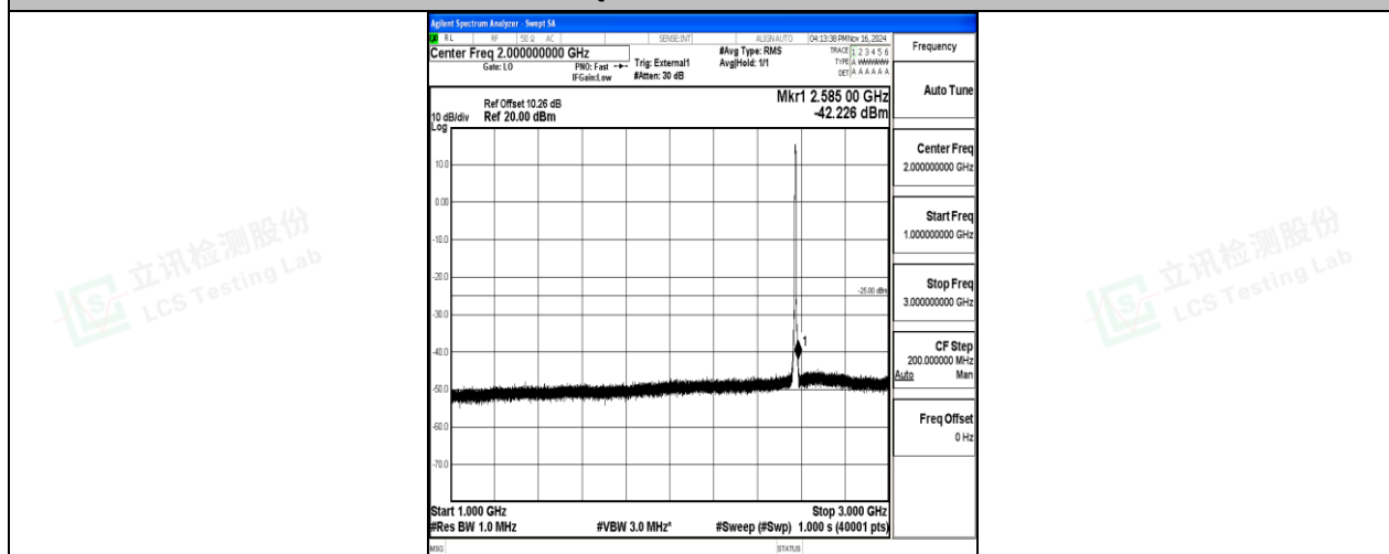
Band38-5MHz-16QAM-37775-25RB#0-1000~3000-PASS
