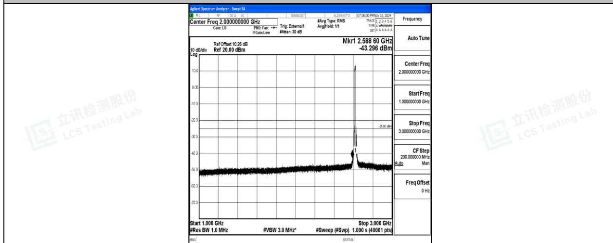
Band38-10MHz-16QAM-38200-50RB#0-1000~3000-PASS
