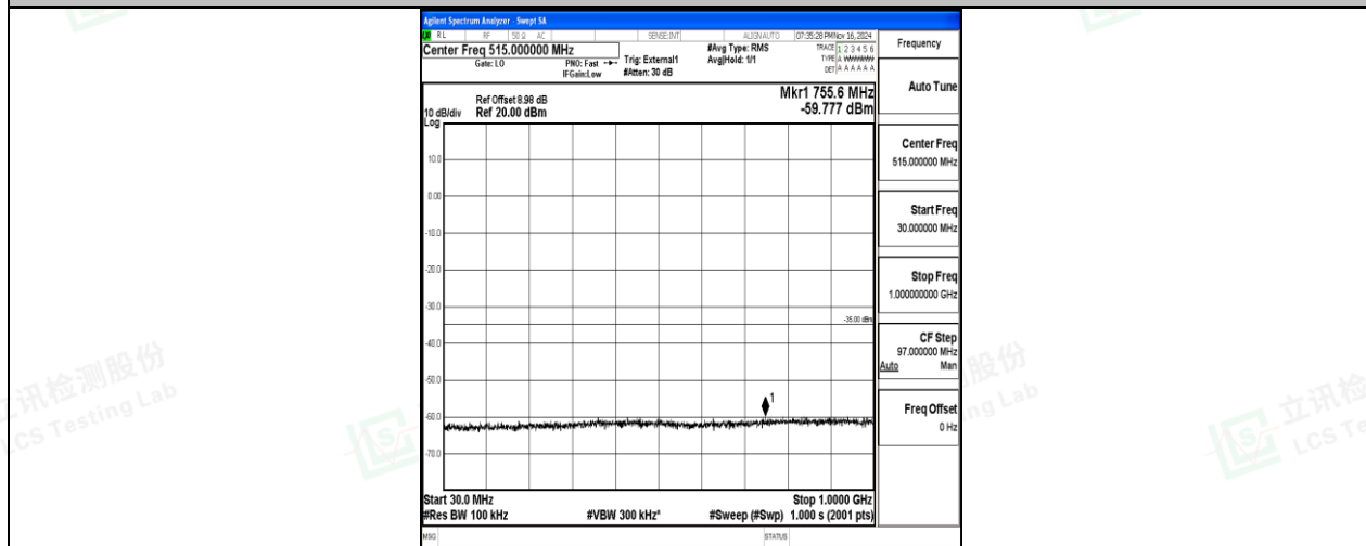
Band38-10MHz-16QAM-38200-50RB#0-30~1000-PASS
