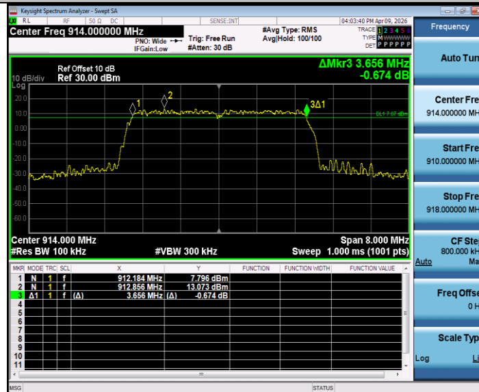
4M_Ant1_914
