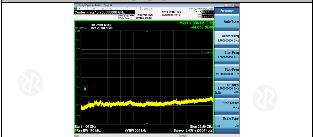
2M_Ant1_903_1000~26500
