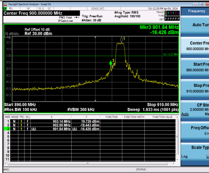
2M_Ant1_Low_903
