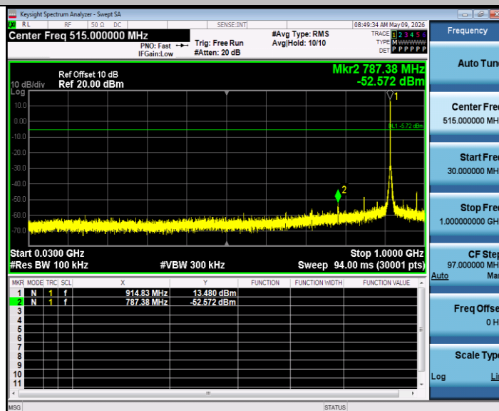
2M_Ant1_915_30~1000
