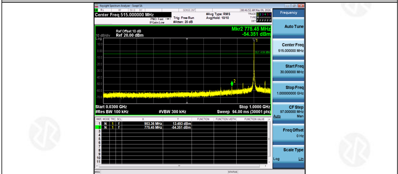
2M_Ant1_903_30~1000
