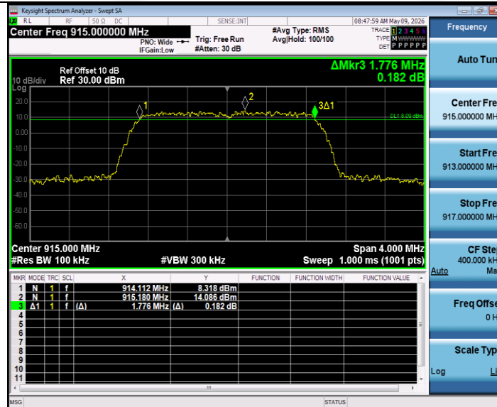
2M_Ant1_915
