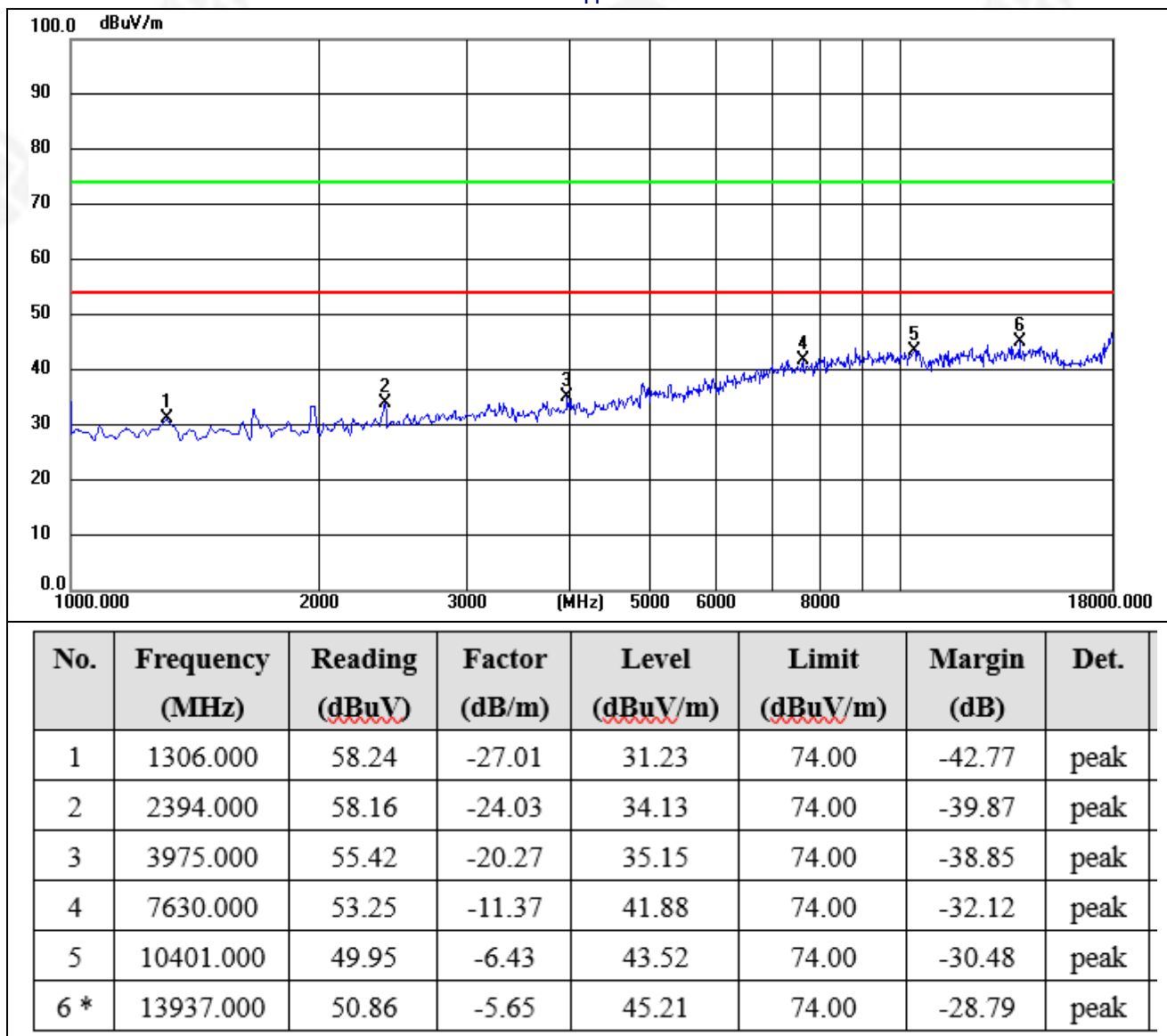
BLE-1M 2440 H
