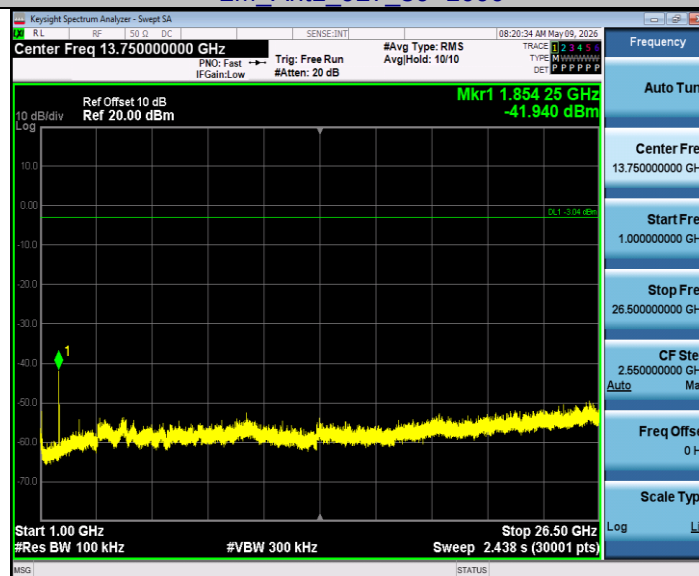
2M_Ant1_927_1000~26500
