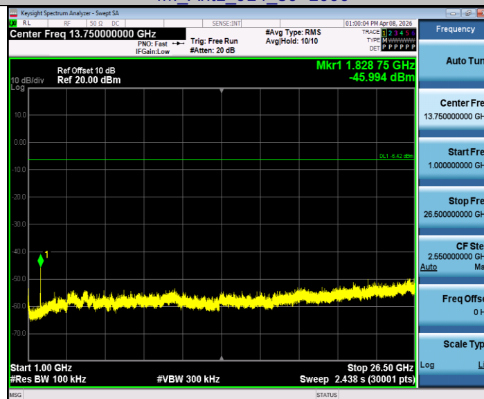
4M_Ant1_914_1000~26500
