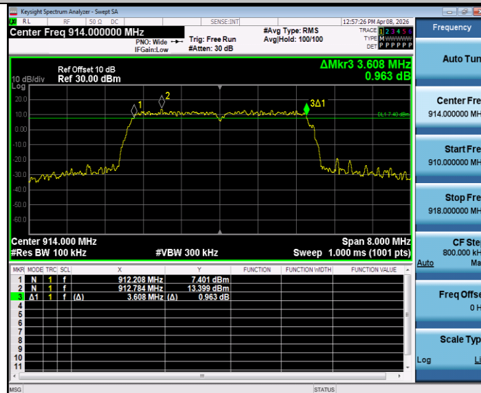
BLE_4M_Ant1_914
