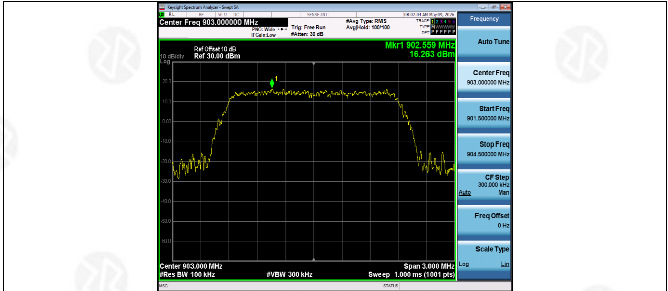
2M Ant1_903_0~Reference
