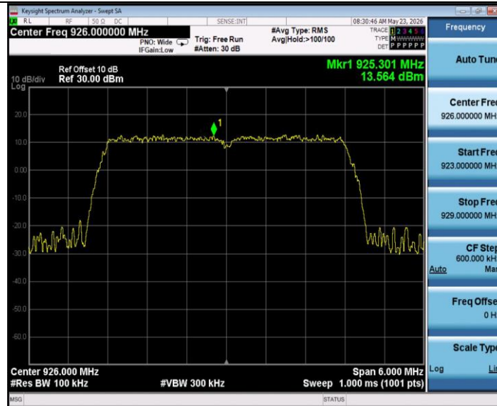
4M_Ant1_926_0~Reference
