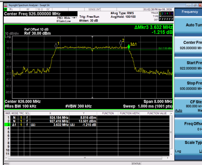
BLE_4M_Ant1_926
