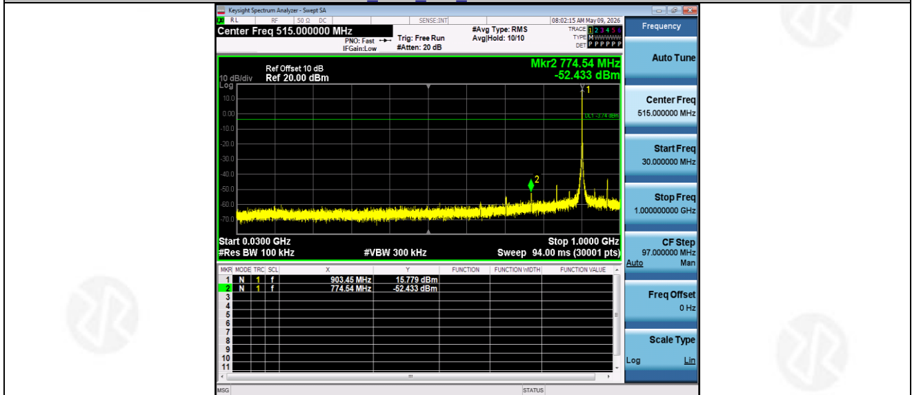
2M Ant1_903_30~1000
