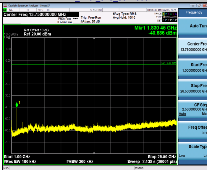
2M_Ant1_915_1000~26500
