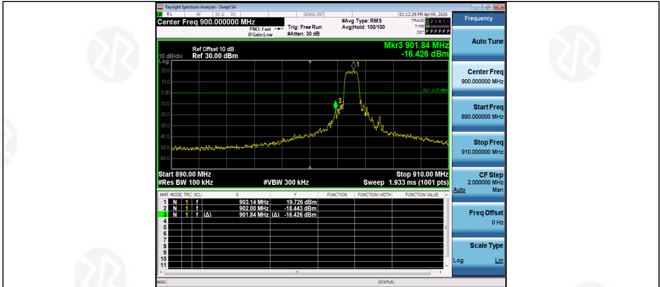
2M_Ant1_Low_903
