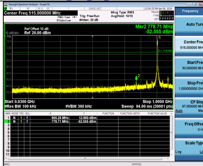
4M_Ant1_906_30~1000
