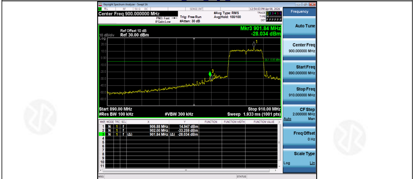
4M_Ant1_Low_906
