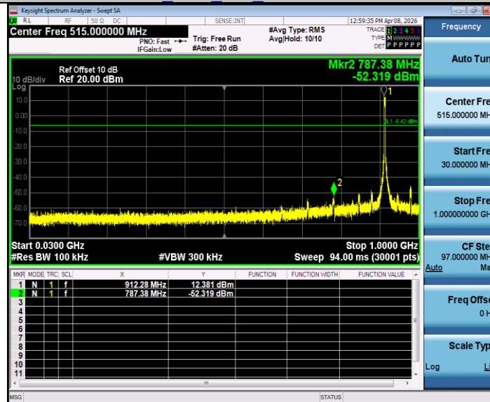
4M_Ant1_914_30~1000
