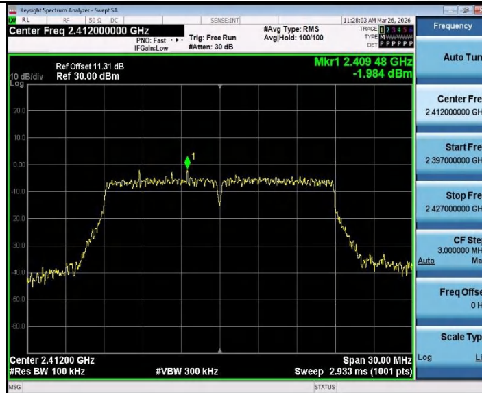
11N20SISO_Ant1_2412_0-Reference
