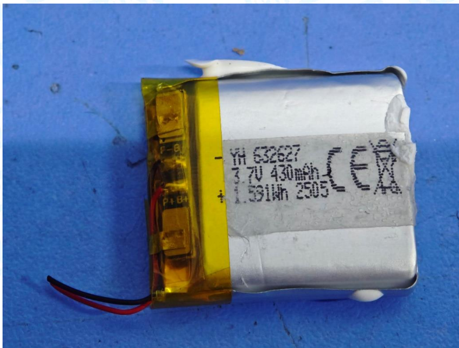
Photo 24 Appearance of Battery
