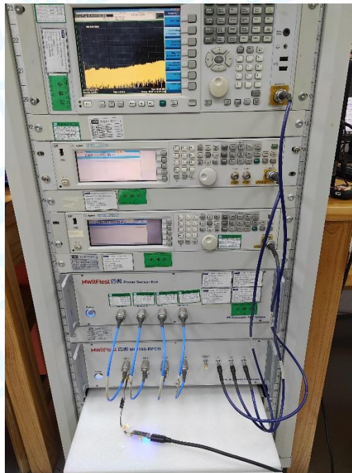
Photo of Setup for Conducted Measurements
