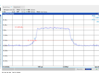
CH116 26 dB Bandwidth
