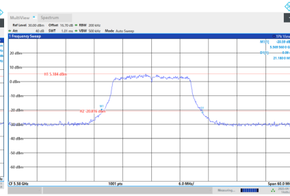
CH116 26 dB Bandwidth
