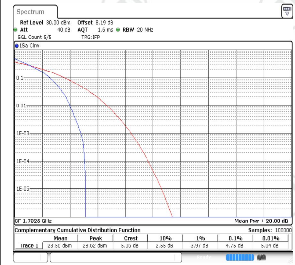
Band4-15MHz-QPSK-20175-PASS
