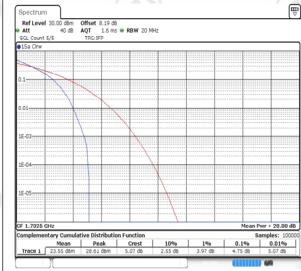
Band4-15MHz-16QAM-20175-PASS
