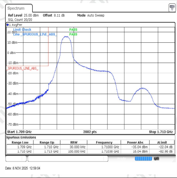
Band4-3MHz-16QAM-19965-PASS
