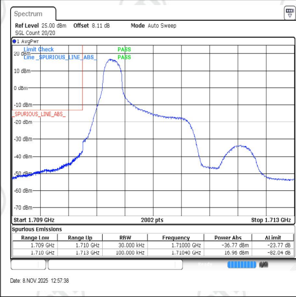
Band4-3MHz-QPSK-19965-PASS
