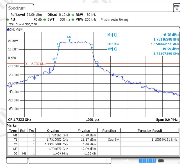
Band4-1.4MHz-16QAM-20175-PASS
