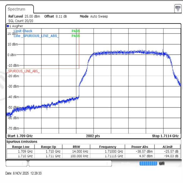
Band4-1.4MHz-16QAM-19957-PASS
