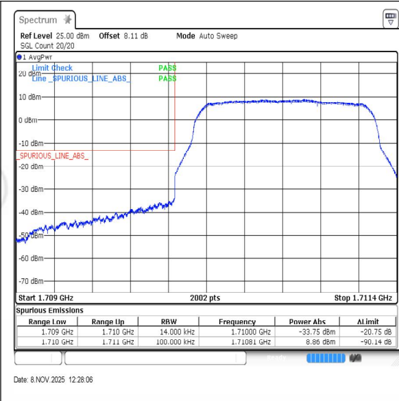
Band4-1.4MHz-QPSK-19957-PASS
