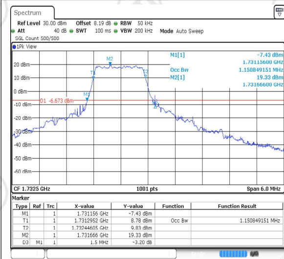
Band4-1.4MHz-QPSK-20175-PASS
