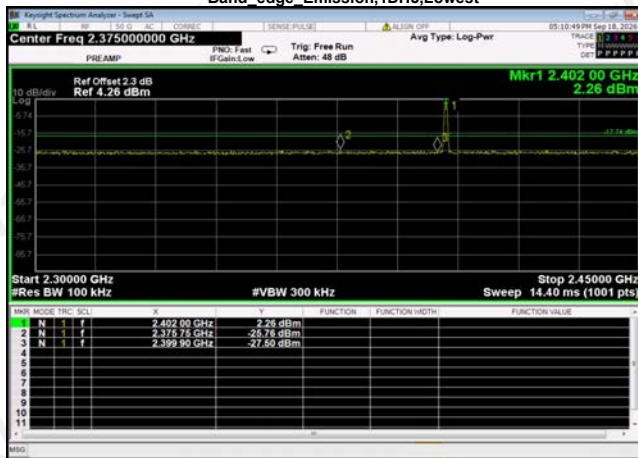
Band edge Emission,1DH5,Lowest
