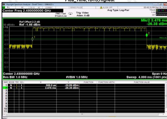
Plus Time,1DH5,Highest
