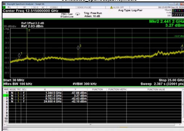
Conducted_Spurious,2DH5,Middle
