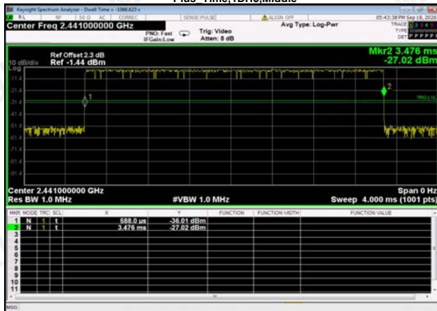
Plus Time,1DH5,Middle
