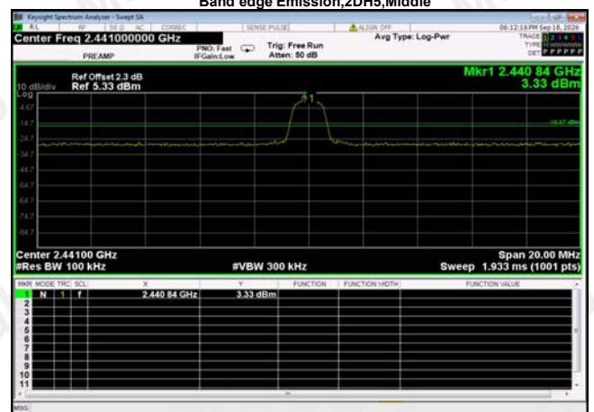
Band edge Emission,2DH5,Middle
