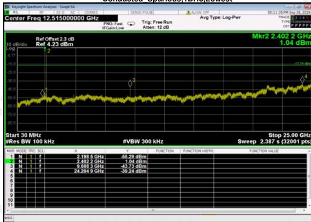
Conducted_Spurious,1DH5,Lowest
