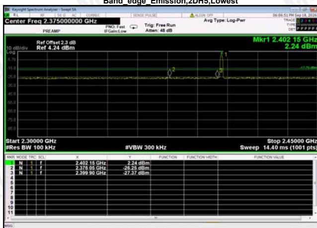
Band edge Emission,2DH5,Lowest
