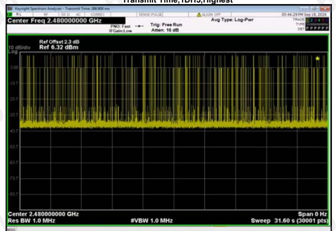
Transmit Time,1DH5,Highest
