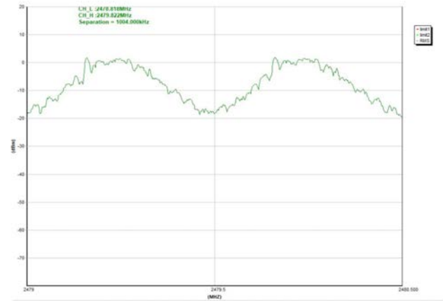
Hopping Frequency Separation,1DH5,Highest
