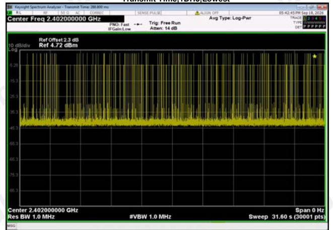
Transmit Time,1DH5,Lowest
