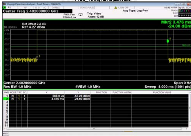
Plus Time,1DH5,Lowest
