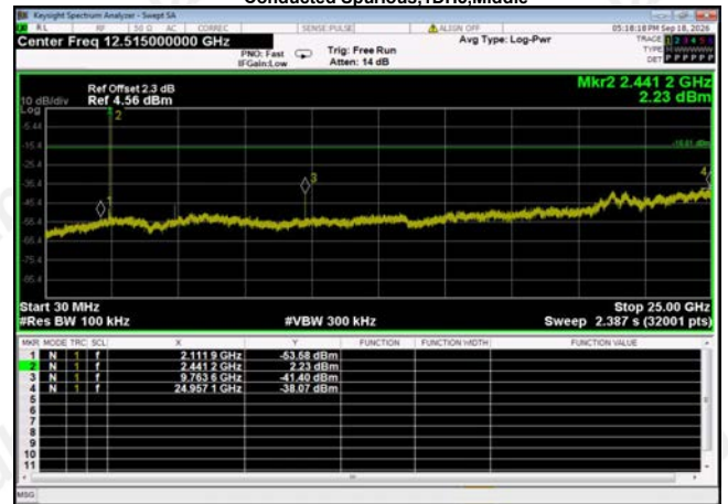
Conducted Spurious,1DH5,Middle
