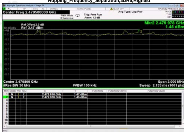
Hopping_Frequency_Separation,3DH5,Highest
