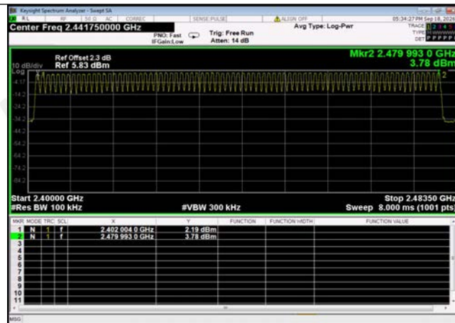
GFSK Modulation
