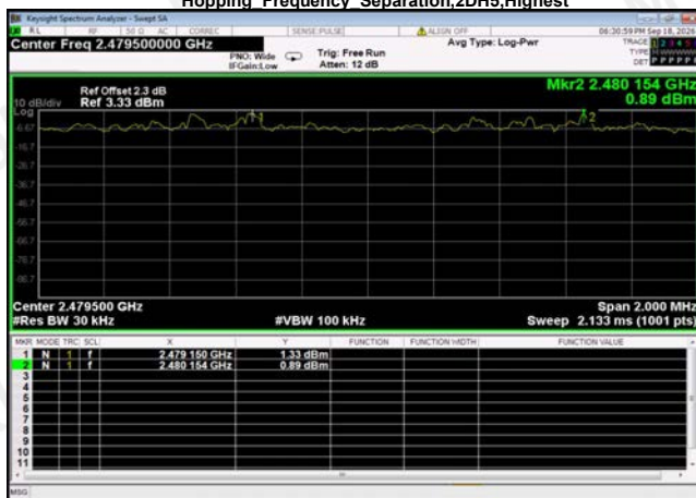
Hopping_Frequency_Separation,2DH5,Highest
