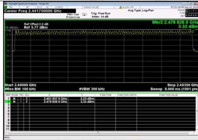
8-DPSK Modulation
