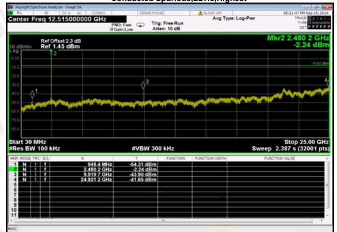
Conducted Spurious,2DH5,Highest
