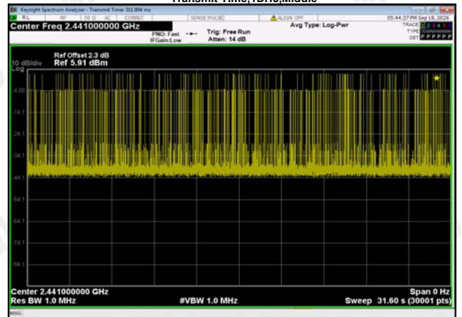
Transmit Time,1DH5,Middle
