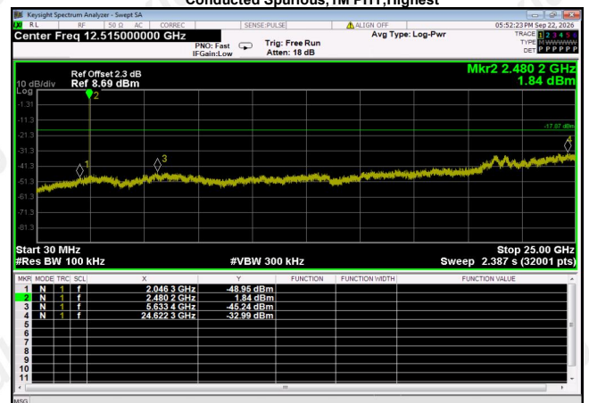
Conducted Spurious,1M PHY,Highest
