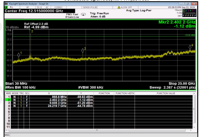
Conducted Spurious,1M PHY,Lowest
