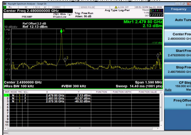
Conducted Spurious Reference,1M PHY,Highest
