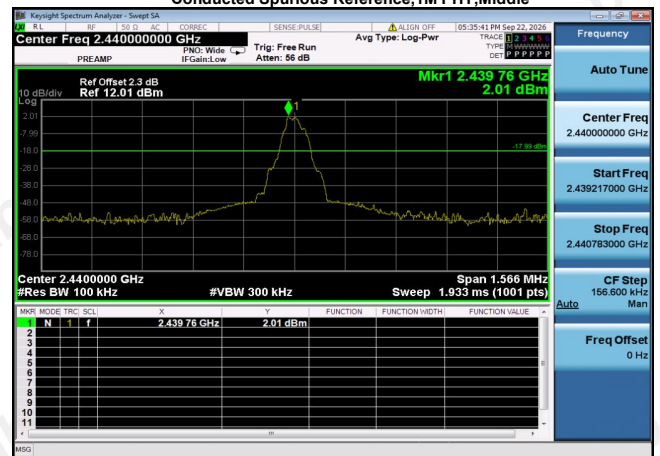
Conducted Spurious Reference,1M PHY,Middle
