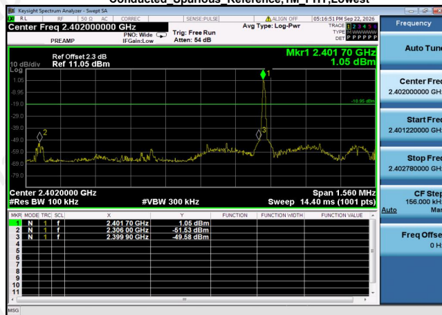
Conducted Spurious Reference,1M PHY,Lowest
