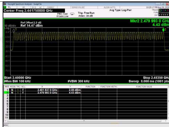
GFSK Modulation
