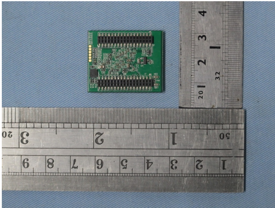
05. Rear view of PCB2
