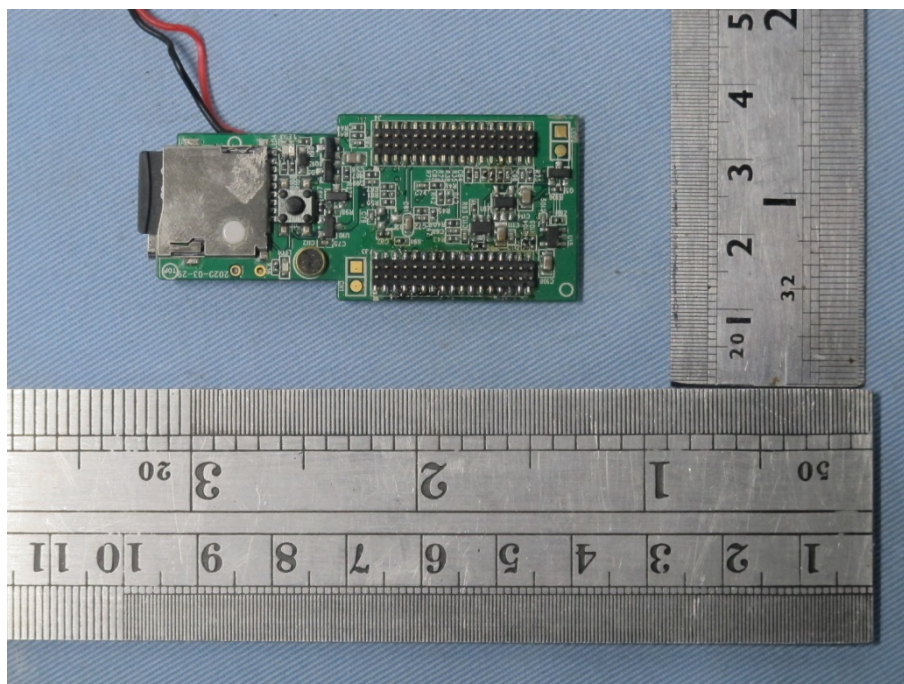
02. Front view of PCB1
