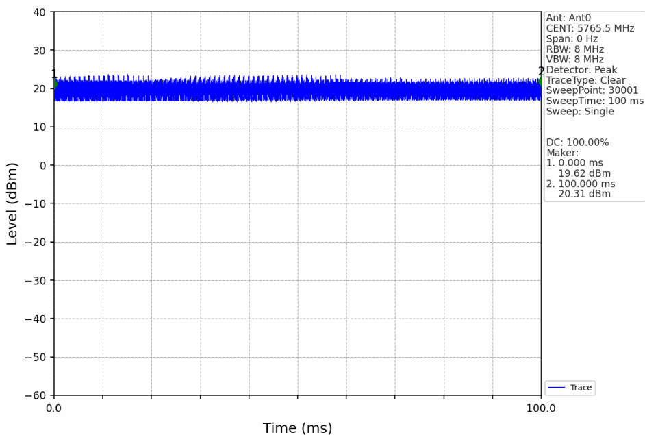
80M_LCH_5765.5MHz_Ant0_NTNV
