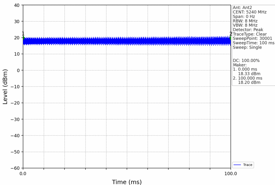
20M_HCH_5240MHz_Ant2_NTNV
