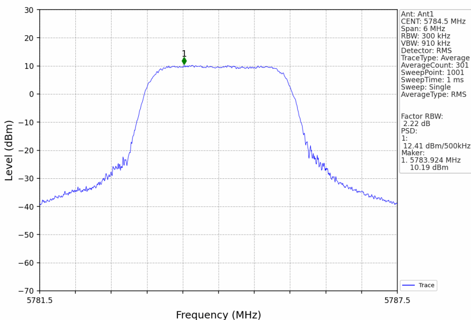
3M_MCH_5784.5MHz_Ant1_NTNV
