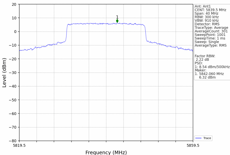
20M_HCH_5839.5MHz_Ant1_NTNV
