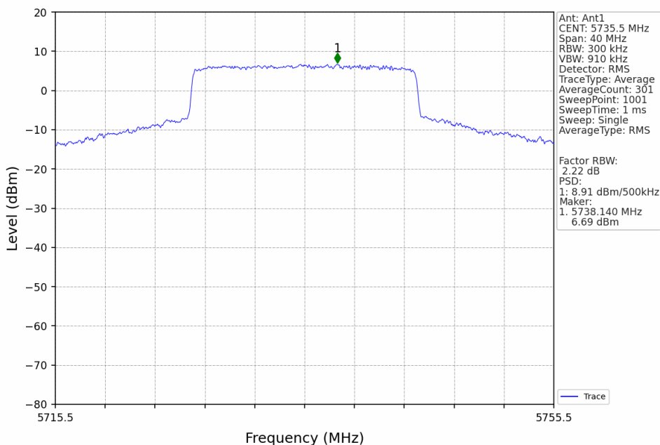
20M_LCH_5735.5MHz_Ant1_NTNV
