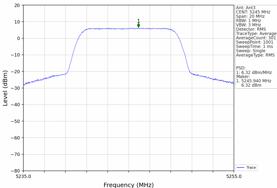
10M_HCH_5245MHz_Ant3_NTNV
