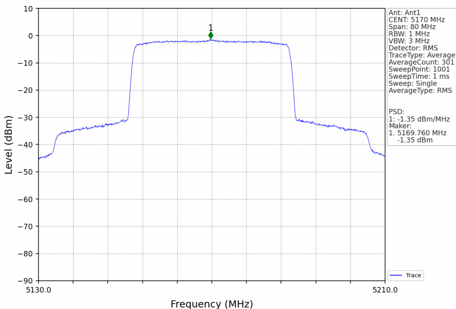
40M_LCH_5170MHz_Ant1_NTNV
