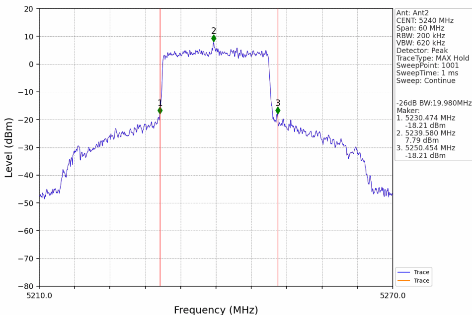
20M_HCH_5240MHz_Ant2_NTNV
