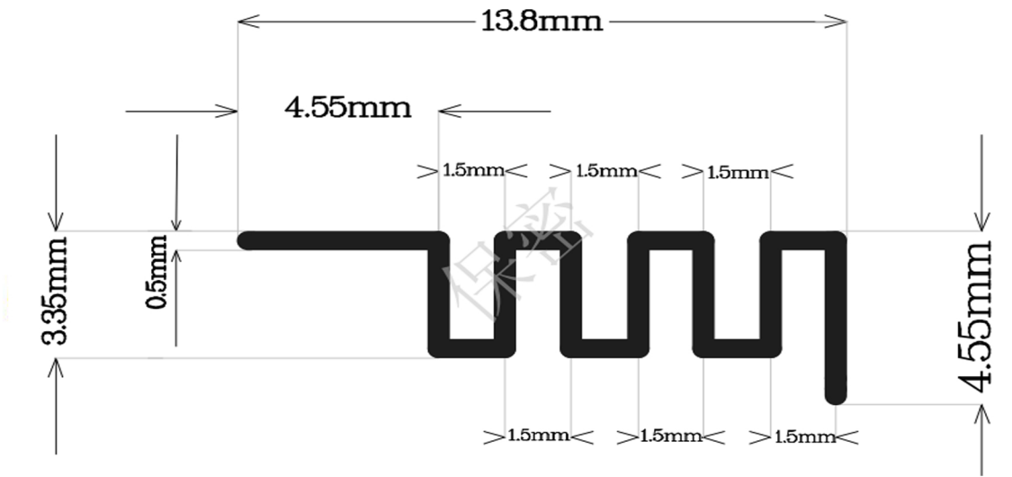
Antenna Photo & Length (mm)
