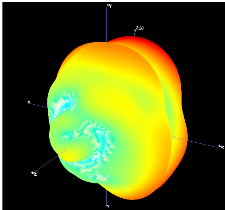
B1.2 3D Pattern for 2440MHz
