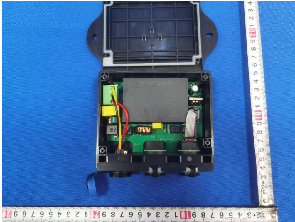
Power supply
