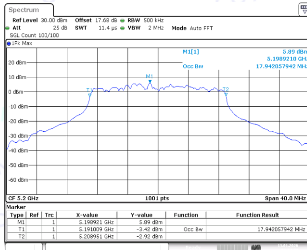
11N20SISO-Ant1-5200
