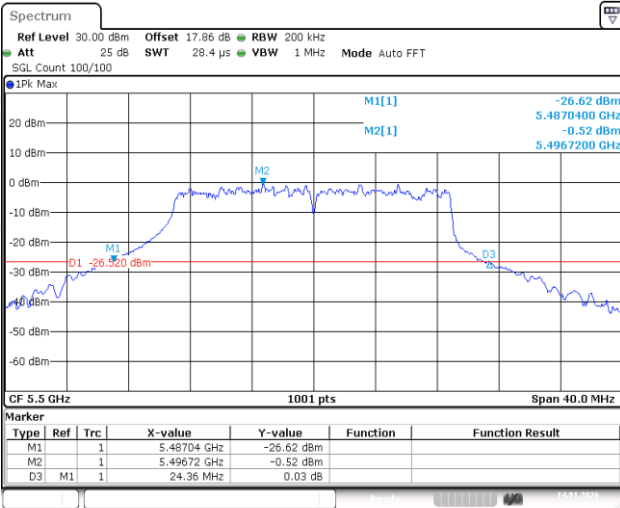
11AX20SISO-Ant1-5500
