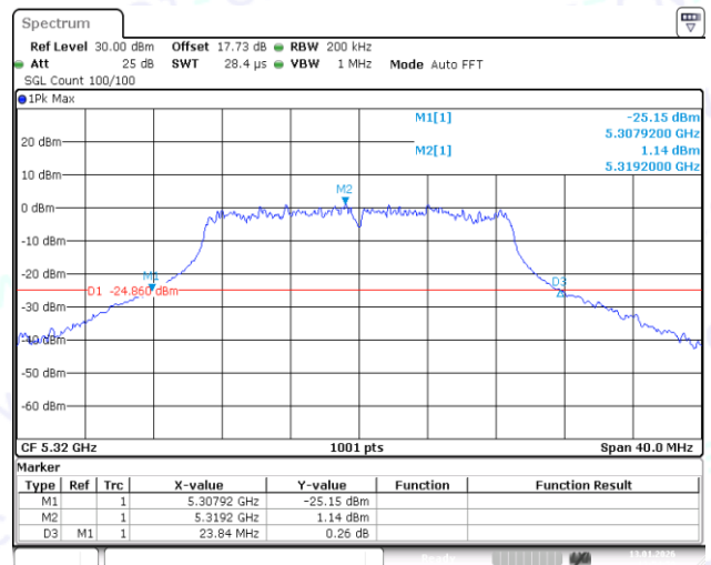
11N20SISO-Ant1-5320
