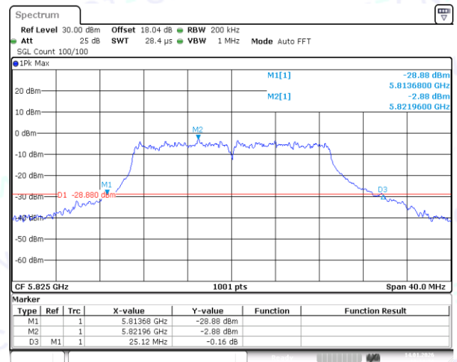
11N20SISO-Ant1-5825
