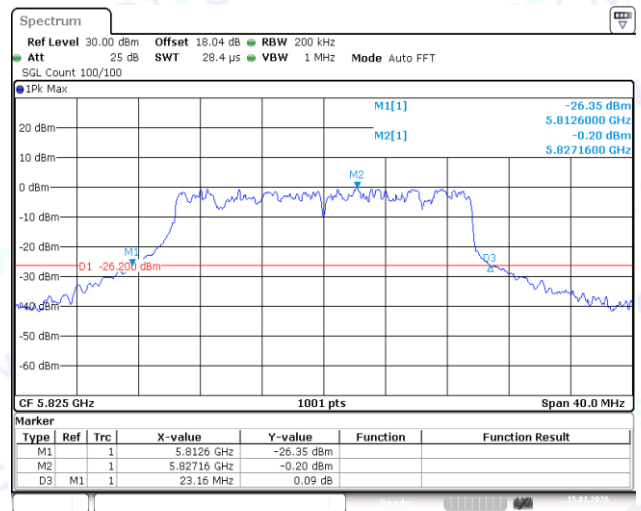
11AX20SISO-Ant1-5825
