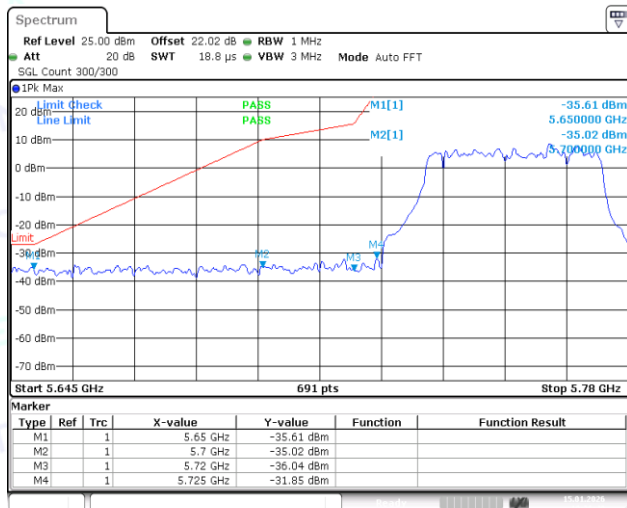
11AX40SISO-Ant1-5755-PASS
