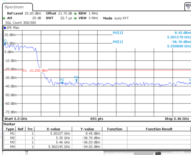
11AC40SISO-Ant1-5310-PASS
