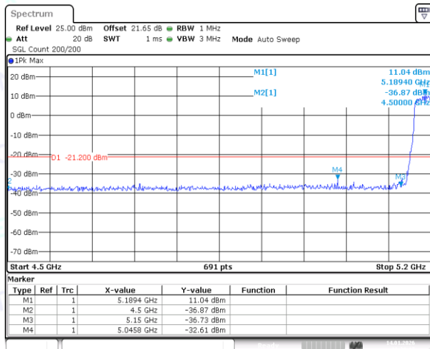
11AX40SISO-Ant1-5190-PASS
